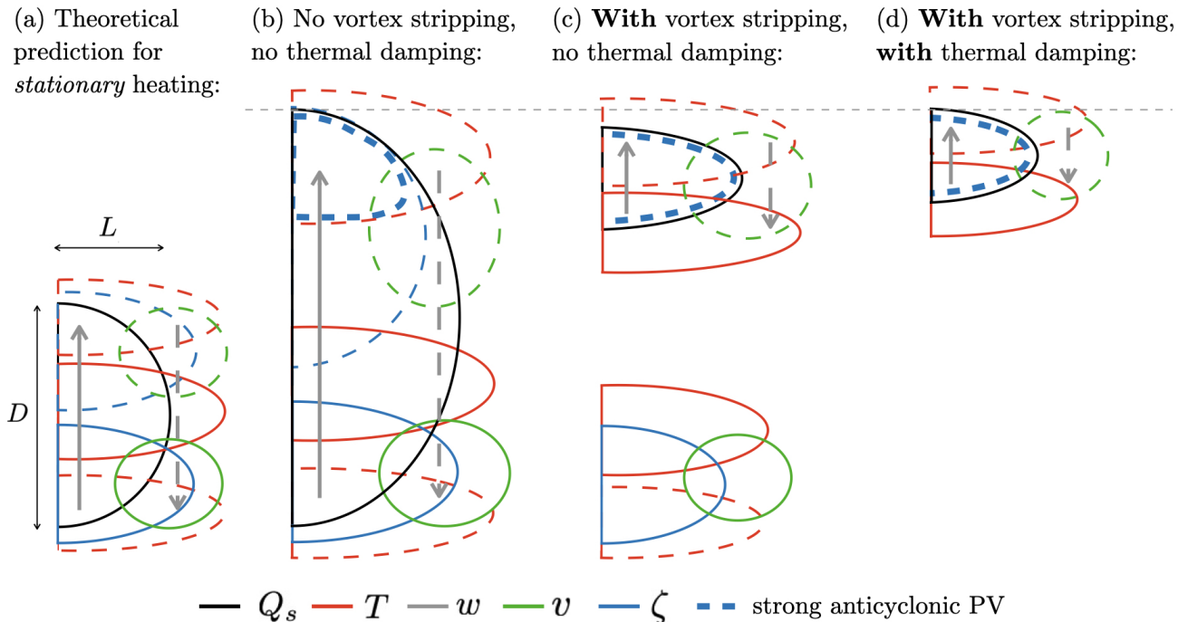
Figure 9. Schematic summarising the physical processes in our theoretical model for aerosol-filled vortices. For reference, panel (a) displays the theoretical prediction for stationary heating (e.g., Hoskins et al., 2003; Davies, 2015). The key behaviour of our coupled tracer-dynamics system is shown in (b) without vortex stripping and without thermal damping, (c) when vortex stripping is applied without thermal damping, (d) with both vortex stripping and thermal damping incorporated.
