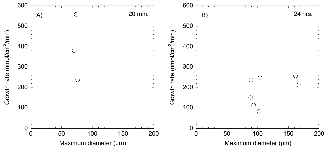
285 Figure 4: The comparison between the size of the individuals and the growth rate: a) in 20 min. b) in 24 hours. Note that for some individuals, only the growth area was recorded during microscope observation instead of capturing the entire individual.
