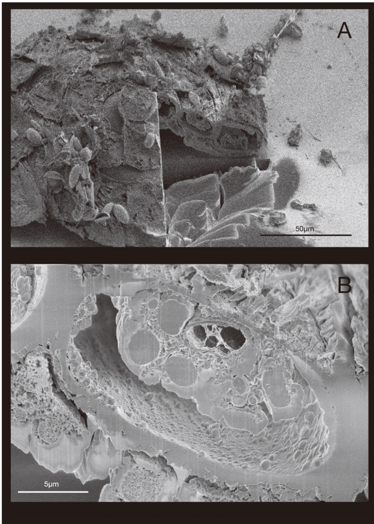
280 Figure 3: Transverse section of S. vivipara tests micromachined by FIB. The cross section of the test is nearly elliptical and tubular.
