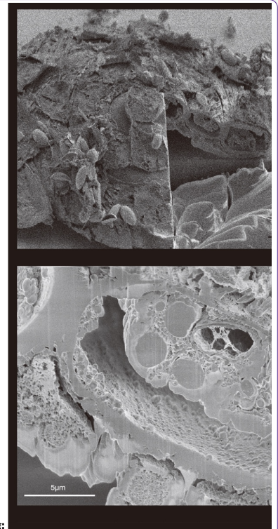
削除: Figure 4: Transverse section of a shell of S. vivipara micromachined by FIB. The cross section of the test is nearly elliptical and tubular.
