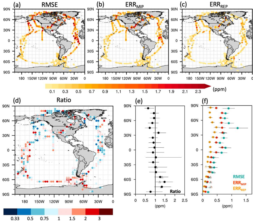
340 Figure 3: Spatial distributions of (a) RMSE , (b) ERR MIP , (c) ERR REP , and (d) Ratio ( = \sqrt{(ERR_{OBS} (= 0.1 \text{ ppm}))^2 + ERR_{REP}^2 + ERR_{MIP}^2} / RMSE ) where ATom (circle) and ORCAS (triangle) airborne measurements were taken and (e and f) their latitudinal distributions smoothed by 10° moving average with 95% confidence intervals derived from 1000 bootstrap samples of datasets (error bar).
