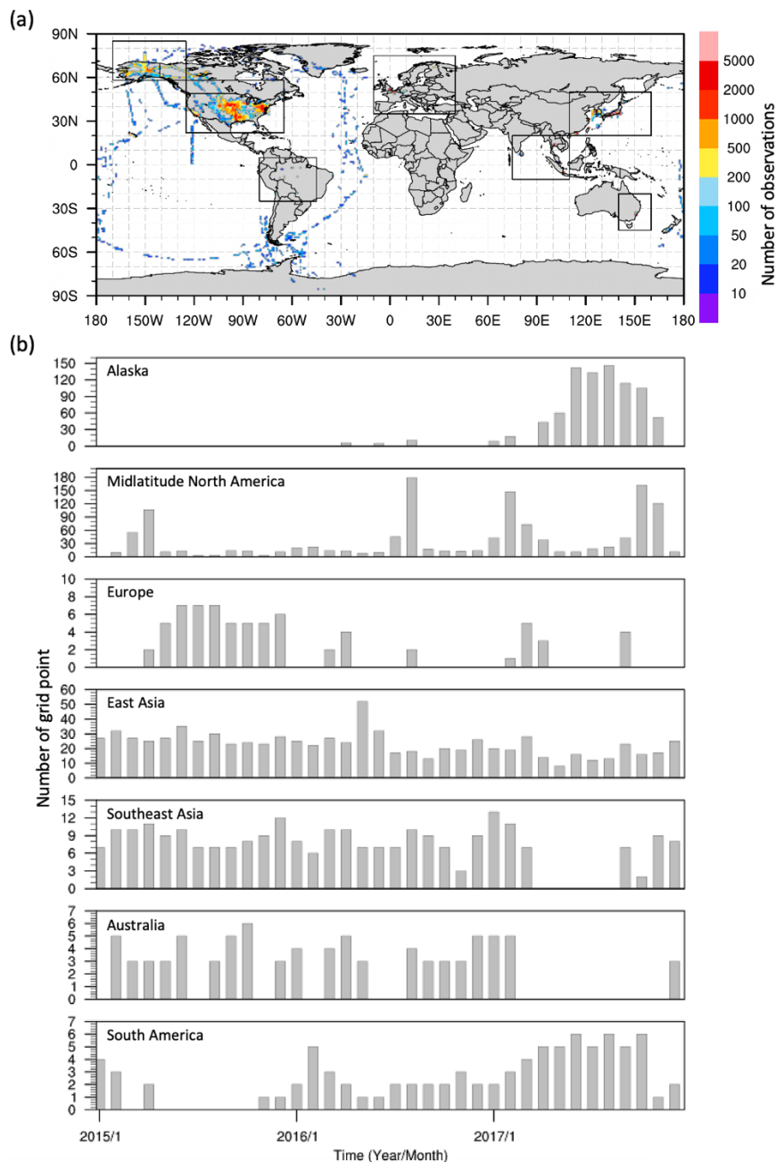
Figure 2: (a) Total number of airborne measurement data used in this study at each 1^\circ \times 1^\circ grid point and (b) the number of 1^\circ \times 1^\circ grid-points, where more than 10 data is available, within each region and each month for the period 2015–2017.
