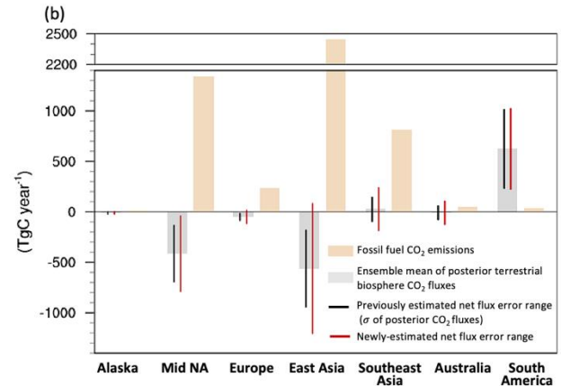
Figure 6: (a) Number of months selected as the effective area for airborne measurements. The outlined area represents selected areas for more than eight months or equal. (b) Annual total terrestrial biosphere CO 2 fluxes obtained from the ensemble mean of ten OCO-2 MIP models and annual total fossil fuel CO 2 emissions estimated from ODIAIC data for each outlined area averaged over the period 2015–2017. The black error bars denote ± in black and red indicate the one standard deviation of the inversion estimates posterior net land fluxes, identical to those of the posterior terrestrial biosphere fluxes. The error bars in red indicate the newly-estimated range of errors range in the posterior net land fluxes from this study, respectively.
