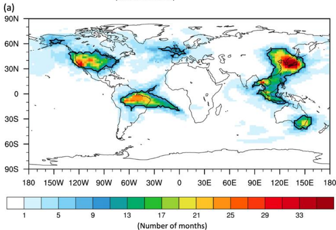
Figure 6: (a) Number of months selected as the effective area for airborne measurements. The outlined area represents selected areas for more than eight months or equal. (b) Annual total terrestrial biosphere CO 2 fluxes obtained from the ensemble mean of ten OCO-2 MIP models and annual total fossil fuel CO 2 emissions estimated from ODIAIC data for each outlined area averaged over the period 2015–2017. The black error bars denote ± in black and red indicate the one standard deviation of the inversion estimates posterior net land fluxes, identical to those of the posterior terrestrial biosphere fluxes. The error bars in red indicate the newly-estimated range of errors range in the posterior net land fluxes from this study, respectively.
