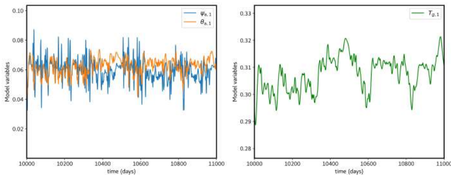
Figure 1. Temporal evolution of barotropic ( \psi_{a1} ) and baroclinic ( \theta_{a1} ) atmospheric streamfunction and the ground temperature ( T_{g1} ) for C_g = 300 \text{ Wm}^{-2} and k_d = 0.085 .
