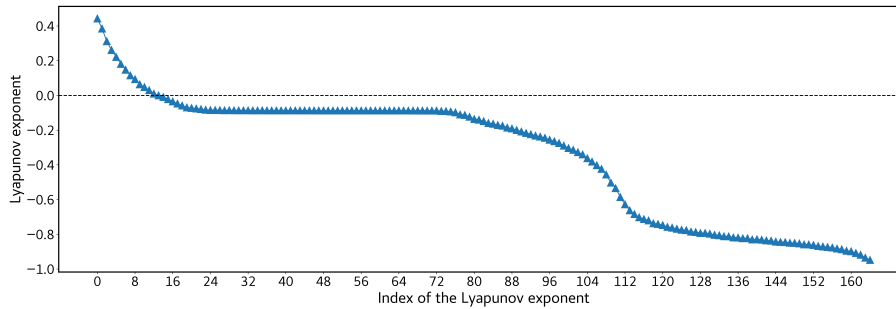
Figure 12. Lyapunov spectrum of the land-atmosphere coupled model for C_g = 300 \text{ Wm}^{-2} and k_d = 0.085 in (5,5) model configuration. The values of the Lyapunov exponents are given in days -1 .
