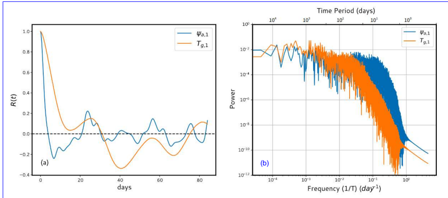
Figure 2. (a) Autocorrelation of barotropic ( \psi_{a,1} ) atmospheric streamfunction and the ground temperature ( T_{g,1} ) for C_g = 300 \text{ W m}^{-2} and k_d = 0.085 . (b) Powerspectrum of the same variables.
