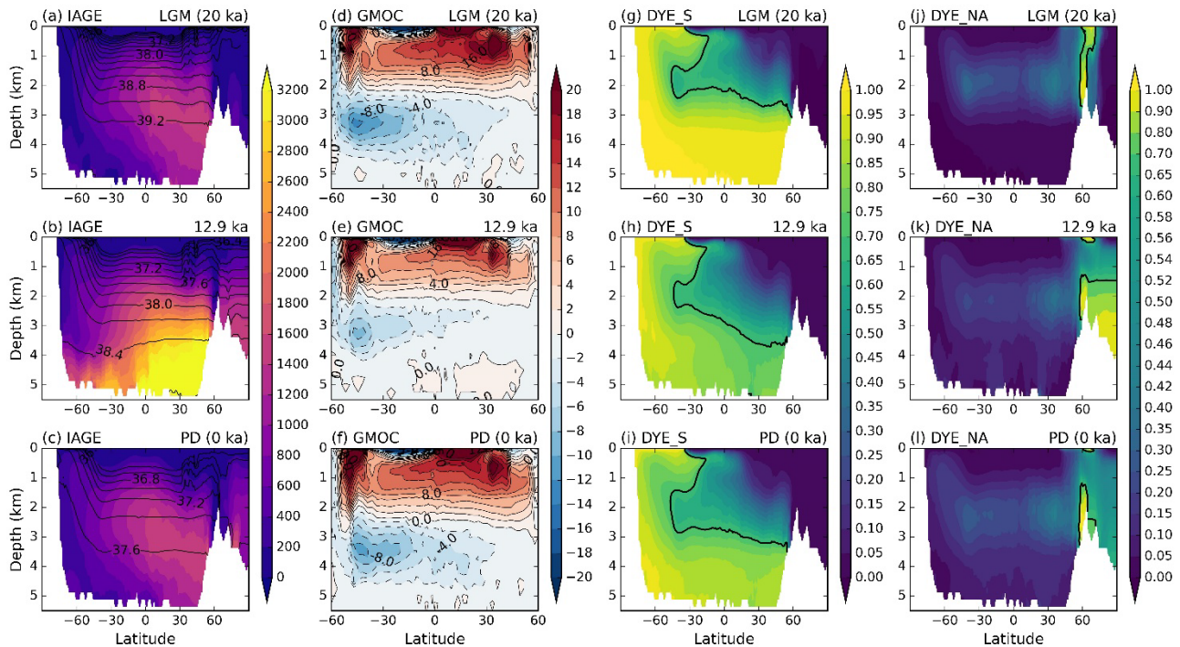
145 Figure 2 The global zonal mean distributions at LGM (20 ka), 12.9 ka, and present day (PD, 0 ka). (a-c) IAGE (shading; unit in year) with isopycnals ( \sigma_2 ; potential density referenced to 2000 m; black contour lines; unit in \text{kg}/\text{m}^3 ). (d-f) Global residual meridional overturning circulation streamfunction (GMOC; unit in Sv). (g-i) Dye-South : percentage of water originating from the Southern Ocean. (j-l) Dye-North: percentage of water originating from the North Atlantic. The thick black contours on dye tracers (g-l) represent the value of 0.7. Note the nonlinear magnitude of the colour bar for Dye-North.
