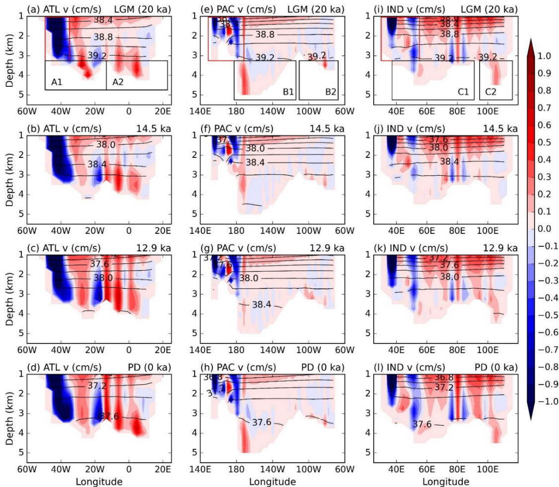
230 Figure 5 Meridional velocity (shading) and potential density (lines) referenced to 2000 m at 30° S during the LGM (20 ka), 14.5 ka, 12.9 ka, and PD (0 ka) in the C-iTRACE. The shading contour interval is 0.1 cm/s and the black line contour interval is 0.2 kg/m 3 . The southward deep western boundary current is defined as the southward integrated volume transport within the highlighted red box on (a, e, i) for the Atlantic, Pacific, and Indian Oceans respectively. The export pathways of AABW in each basin is calculated as the northward integrated volume transport within the black boxes on (a, e, i), noted as A1 and A2 for the Atlantic, B1 and B2 for the Pacific, and C1 and C2 for Indian Ocean.
