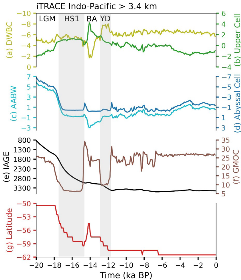
Figure 12 Similar to Fig. 11 but for Indo-Pacific basin.
