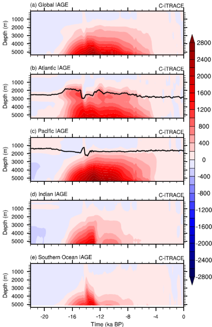
220 Figure 4 Depth-time Hovmöller diagram of IAGE anomalies relative to present day over global and different basins. (a) The global mean. (b) Atlantic basin average. (c) Pacific basin average. (d) Indian basin average. (e) Southern Ocean average. The thick black lines on (b) and (c) are the depth of the zero-contour of Atlantic and Indo-Pacific Meridional Overturning Streamfunction averaged between 60° N and 30° S respectively.
