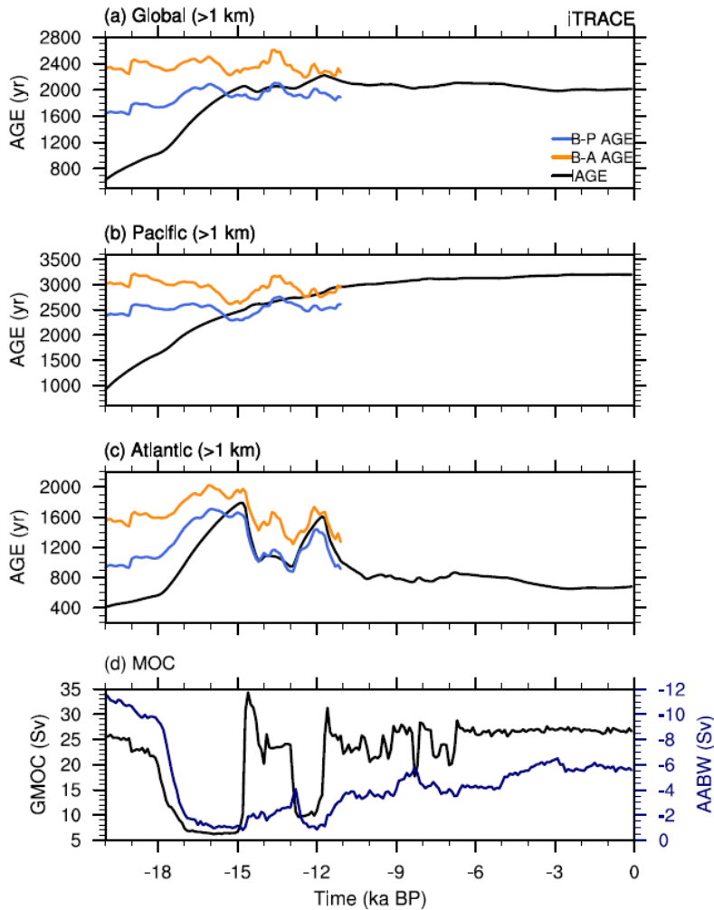
320 Figure 9 Time evolutions in the iTRACE: (a) The global mean ideal age (IAGE; black), B-A age (yellow), and B-P age (blue) averaged below 1 km. (b) The Pacific mean IAGE (black), B-A age (yellow), and B-P age (blue) averaged below 1 km. (c) The Atlantic mean IAGE (black), B-A age (yellow), and B-P age (blue) averaged below 1 km. (d) The GMOC (black) and AABW strength (navy). GMOC intensity is diagnosed as the maximum in the GMOC streamfunction below 500 m over 33° S-60° N, and AABW strength is diagnosed as the maximum in the GMOC streamfunction below 2km from 2° S-70° S.
