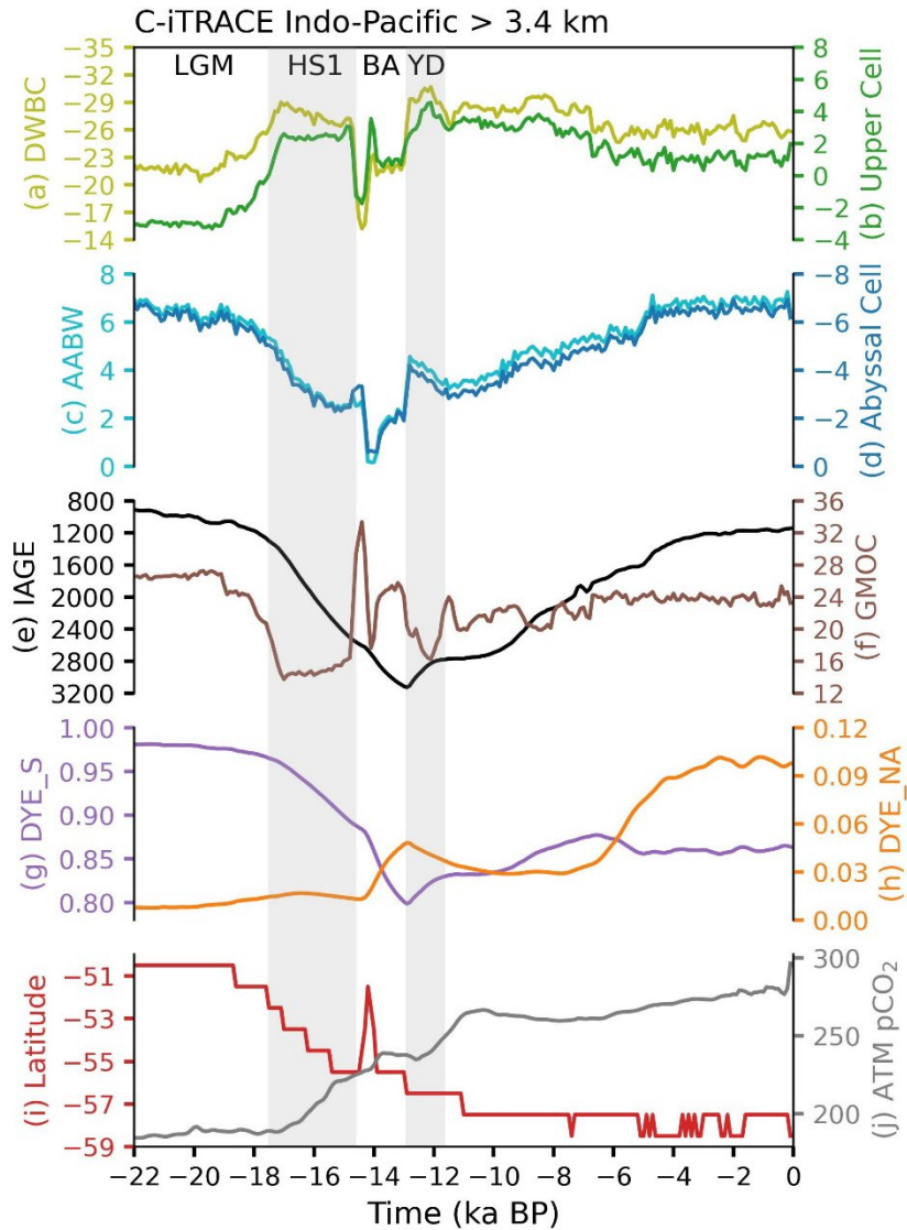
Figure 7 Similar to Fig. 6 but for Indo-Pacific basin.
