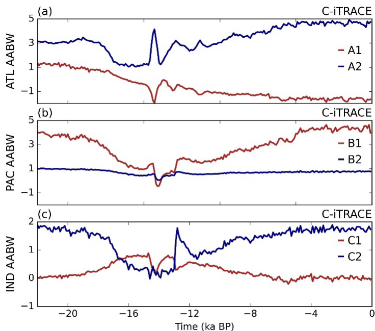
Figure 8 Time evolutions of AABW export pathways into the (a) Atlantic, (b) Pacific, and (c) Indian Oceans in the C-iTRACE. Each branch of AABW transport (unit in Sv) across basins is calculated as the northward integrated volume transport within the black boxes on Figure 5a, 5e, and 5i, noted as A1 and A2 for the Atlantic, B1 and B2 for the Pacific, and C1 and C2 for Indian Ocean.
