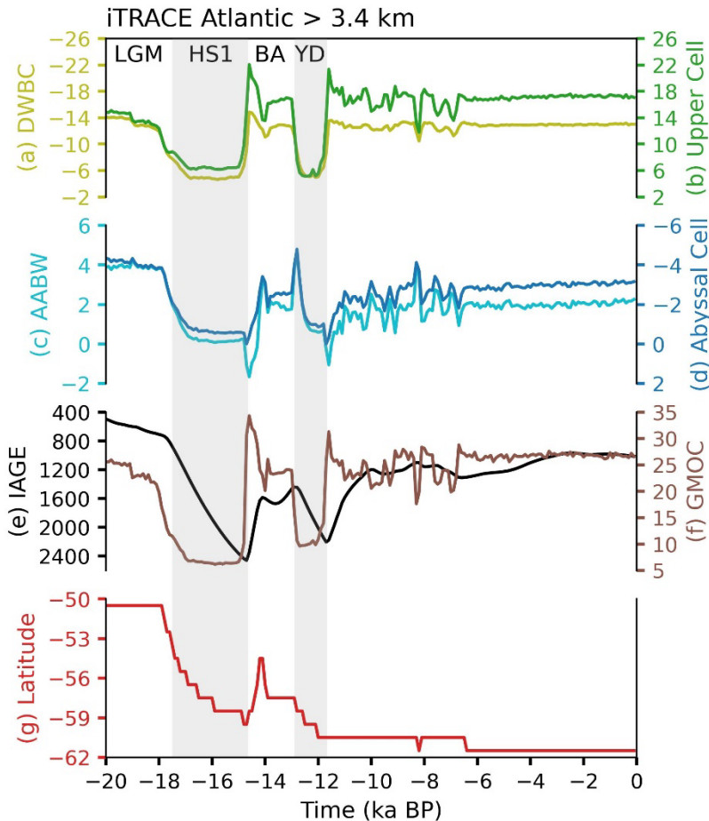
350 Figure 11 Atlantic deglacial evolutions in the iTRACE: (a) Southward DWBC (light olive, unit in Sv) defined as the southward integrated volume transport within the red box in Figure 10, (b) Upper cell (green, unit in Sv) defined as the maximum in AMOC between 0.6-3.5 km at 30° S, (c) AABW transport (cyan, unit in Sv) defined as \Psi_{AABW} = -\int_{z=-H}^{z=-3.4km} \int v dx dz where v is meridional velocity component and H is the bottom seafloor, (d) abyssal cell (blue, unit in Sv) defined as the minimum in AMOC below 2.5 km m at 30° S, (e) IAGE (black, unit in yr) averaged below 3.4 km, (f) GMOC strength (brown, unit in Sv), and (g) the 355 latitude of 20% sea ice coverage averaged over Southern Ocean (red). The gray shadings delimit periods of abrupt change. LGM- Last Glacial Maximum; HS1-Heinrich Stadial 1; BA-Bølling-Allerød; YD-Younger Dryas.
