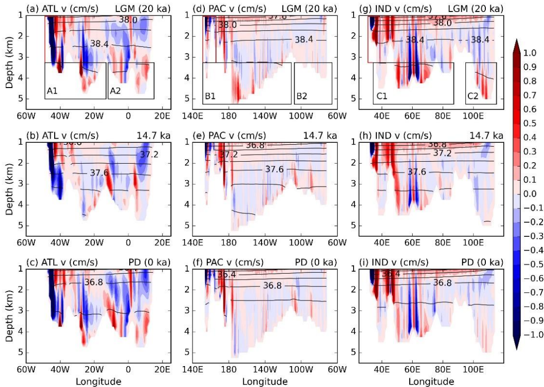
330 Figure 10 Meridional velocity (shading) and potential density (lines) referenced to 2000 m at 30° S during the LGM (20 ka), 14.7 ka, and PD (0 ka) in the iTRACE. The shading contour interval is 0.1 cm/s and the black line contour interval is 0.2 kg/m 3 . The deep western boundary current excluding AABW is defined as the southward integrated volume transport within the highlighted red box on (a, d, g) for the Atlantic, Pacific, and Indian Oceans respectively. The export pathways of AABW in each basin is calculated as the northward integrated volume transport within the black boxes on (a, d, g), noted as A1 and A2 for the Atlantic, B1 and B2 for the Pacific, and C1 and C2 for Indian Ocean. 335
