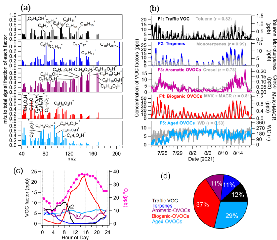
970 Figure 4. Source apportionment of VOCs measured by the PTR-MS. (a) Normalized VOC factor spectra from PMF analysis on the m/z peaks (relative contribution of each factor to each ion); (b) time series of VOC factors including traffic, terpenes, aromatic-OVOCS, biogenic- OVOCS and aged-OVOCS with external tracer species including toluene, monoterpenes, cresol, MVK + MACR and wind direction (WD); (c) median diurnal variations of VOC factors and O_3 975 ( NO_2 + O_3 ); (d) relative contribution of each VOC factors to total VOC concentrations.
