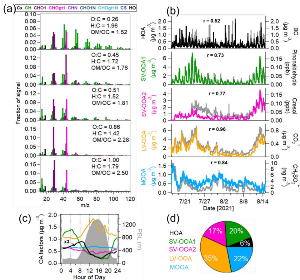
Figure 5. Source apportionment of OA measured by the AMS. (a) Mass spectra of OA factors: hydrocarbon-like OA (HOA), two semi-volatile oxygenated OA (SV-OOA1 and SV-OOA2), 980 low-volatility oxygenated OA (LV-OOA) and marine oxygenated OA (MOOA); (b) time series of OA factors and external tracer species (BC, pinonaldehyde and cresol measured by the PTR-MS, CO 2 + and CH 3 SO 2 + measured by the AMS); (c) median diurnal variations of OA factors and PBL height; and (d) mass fraction of OA factors in total OA mass.
