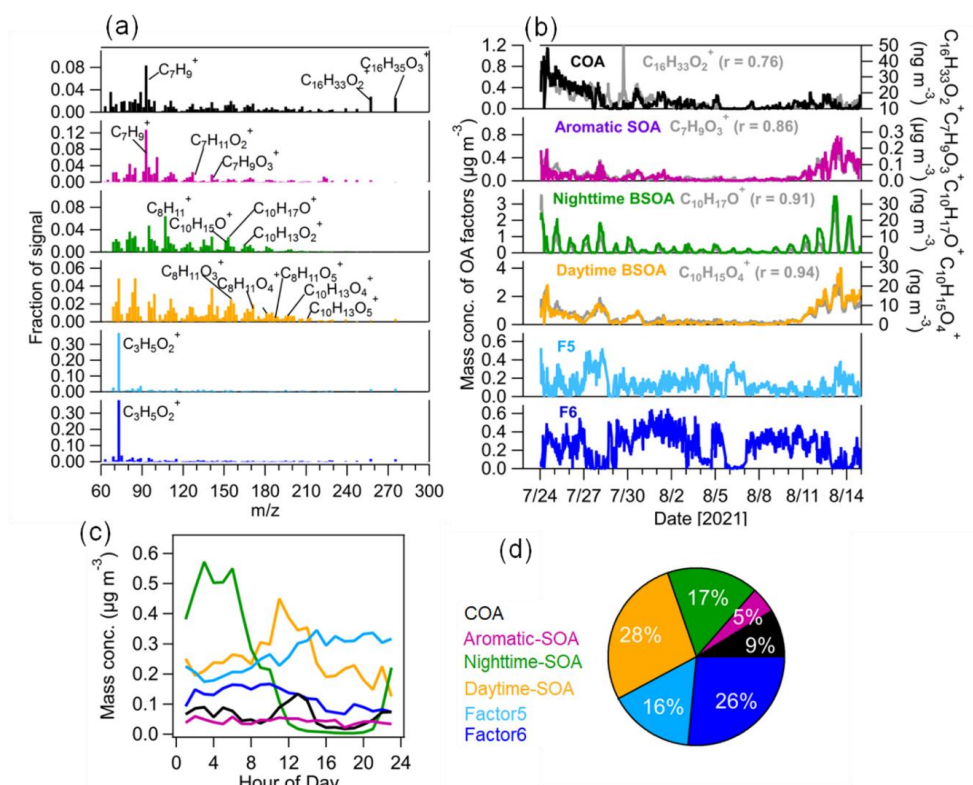
985 Figure 6. Source apportionment of OA measured by the CHARON-PTR-MS. (a) mass spectra of six factors of OA from PMF analysis; (b) time series of six OA factors including cooking- related OA (COA), aromatic hydrocarbon oxidation-related SOA (aromatic-SOA), nighttime and daytime biogenic SOA (Daytime-SOA and nighttime-SOA) with marker ions including C_{16}H_{33}O_2^+ , C_7H_9O_3^+ , C_{10}H_{17}O^+ and C_{10}H_{15}O_4^+ , respectively. Two factors (F5 and F6) 990 dominated by C_3H_5O_2^+ could not be assigned to specific sources; (c) median diurnal variations of OA factors; (d) relative contributions of each OA factor to total OA mass.
