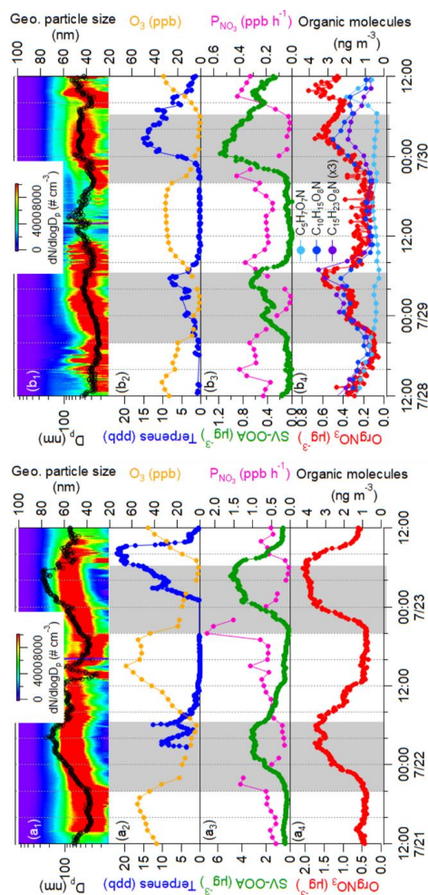
Figure 10. Two cases showing the nighttime particle growth. Time series of particle number size distributions and geometric mean particle size, and mixing ratios of terpenes factor and O 3 , production rate of nitrate radicals (P NO 3 ), and mass concentrations of SV-OOA1 and organic nitrate calculated from the AMS during 21 st -23 rd (a1-a4) and 28 th -30 th July, 2021 (b1-b4). Three particulate organic nitrate molecules (C 5 H 7 O 7 N, C 10 H 15 O 8 N, C 15 H 23 O 8 N) detected by the FIGAERO-CIMS are plotted in (b4). The grey area represents the nighttime from 20:00 to 6:00 next day (local time).
