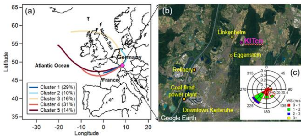
Figure 1. Location of the measurement site along with the clusters of air mass back-trajectories. (a) five major air mass clusters, (b) map of sampling location (KITcn), Eggenstein (LUBW air quality monitor station), two industrial sources (a refinery and a coal-fired power plant) and Linkenheim (a sampling site in summer 2016, Huang et al., 2019) (©Google Earth). (c) Wind rose plot for the entire campaign.
