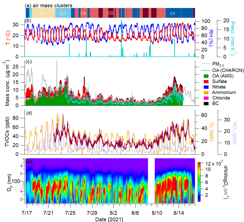
960 Figure 2. Time series of (a) origins of air mass clusters; (b) temperature (T) and relative humidity (RH) and precipitation; (c) mass concentrations of PM 2.5 measured by the OPC, OA measured by the CHARON, OA, sulfate, nitrate, ammonium, chloride measured by the AMS and BC; (d) concentrations of total VOCs (TVOCs, brown line), O 3 and NO 2 ; (e) particle number size distribution measured by the SMPS.
