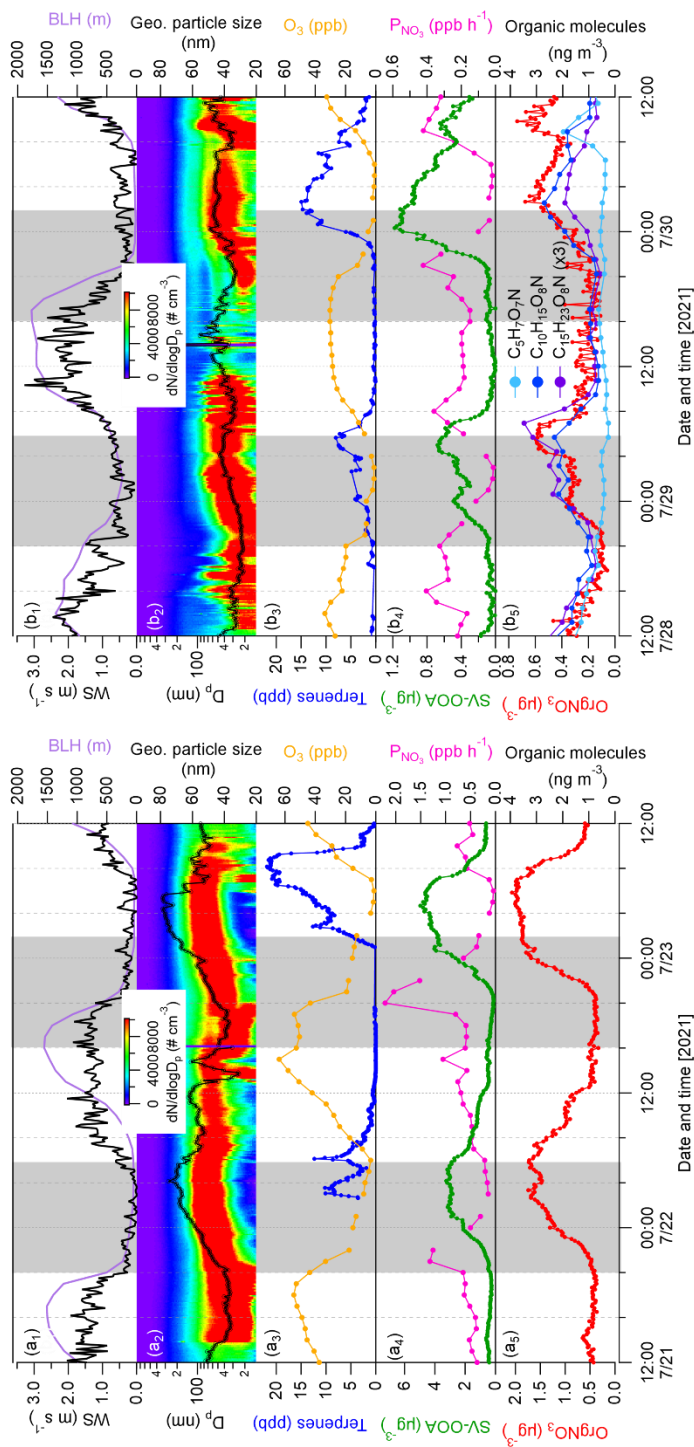
10 Figure 10. Cases showing the nighttime particle growth events as marked in gray shaded areas. Time series of wind speed, boundary layer height, particle number size distributions and geometric mean particle size, and mixing ratios of terpenes factor and O_3 , production rate of nitrate radicals ( P_{NO_3} ), and mass concentrations of SV-OOA1 and organic nitrate calculated from the AMS during 21 st -23 rd (a1-a5) and 28 th -30 th July, 2021 (b1-b5). Three particulate organic nitrate molecules ( C_5H_7O_7N , C_{10}H_{15}O_8N , C_{15}H_{23}O_8N ) detected by the FIGAERO-CIMS are plotted in (b5).
