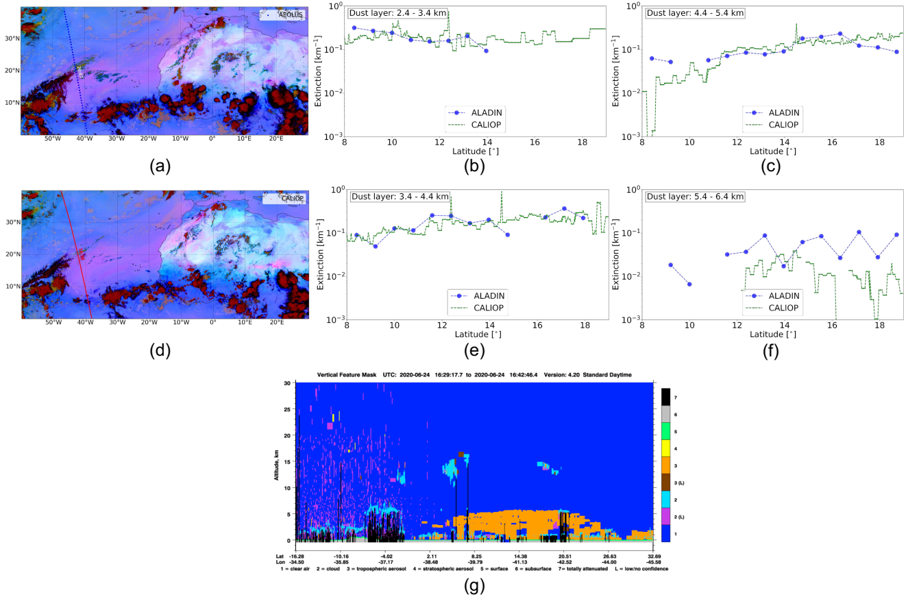
Figure 6. Comparison of aerosol extinction retrievals from collocated orbits on the 24 th June 2020, featuring (a) an Aeolus overpass at 20:47 and (d) a CALIPSO overpass at 16:39, with SEVIRI dust RGB displayed in the background of each. The extinction retrievals from cloud-free regions located between 8° N and 19° N are compared across various altitude layers: (b) 2.4 - 3.4 km, (e) 3.4 - 4.4 km, (c) 4.4 - 5.4 km, and (f) 5.4 - 6.4 km. (g) shows the CALIPSO vertical feature mask retrieved from NASA CALIPSO Standard Browse Images 3 .
