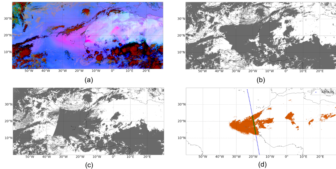
Figure 3. Illustration of SEVIRI products and a generated dust flag used on the 17th June 2020 at 19:12 UTC. (a) SEVIRI dust RGB composite based on three thermal bands (8.7, 10.8 and 12 \mu\text{m} ), where shades of pink to violet denote dust. (b) SEVIRI CLM, highlighting regions identified as clouds in grey. (c) CM SAF cloud mask. (d) Generated dust flag using the method proposed by Ashpole and Washington (2012), illustrating the accurate automatic detection of dust regions over the entire study area. The blue dots in (d) represent the footprints of Aeolus at a horizontal step of approximately 87 km, and the green plus sign marks the location where Aeolus detects dust aerosol in that profile.
