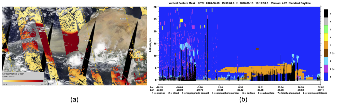
Figure 8. Collocated MODIS Aqua and CALIPSO observations on the 18 th of June 2020, with a time difference of \sim 50 minutes. Panel (a) displays the MODIS Aqua cloud-free AOD at a 3-km resolution accompanied by the ascending CALIPSO track (available from NASA Worldview, last accessed on the 3 rd of July 2023). Panel (b) illustrates the corresponding CALIOP vertical feature mask.
