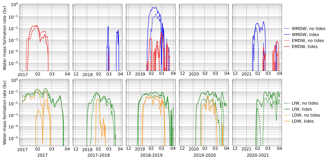
Figure 11. Daily water mass formation rate in winter-winter (DJFM) 2017-2021, for the tidal experiment (solid lines) and the non-tidal experiment (dashed lines). Four types of water mass are included: Western Mediterranean Deep Water (blue), Eastern Mediterranean Deep Water (red), Levantine Intermediate Water (green), and Levantine Deep Water (orange).
