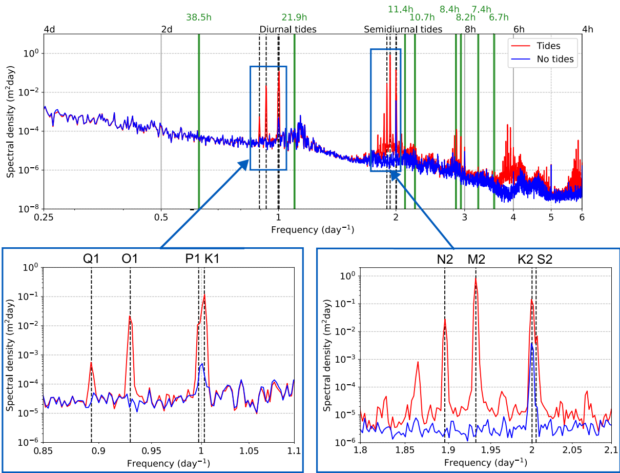
Figure 2. Energy density spectrum of hourly mean sea surface height in the Mediterranean Sea for the period 2017-2021, for the experiment without tides (blue) and with tides (red). The basin-mean spectrum is calculated as an area-weighted mean of the periodogram at each gridpoint in the Mediterranean Sea. Boxes below the figure show the key diurnal and semidiurnal ranges to highlight the representation of each individual tidal component. Green lines on the figure indicate frequencies of known barotropic oscillations in the Mediterranean Sea and its sub-basins.
