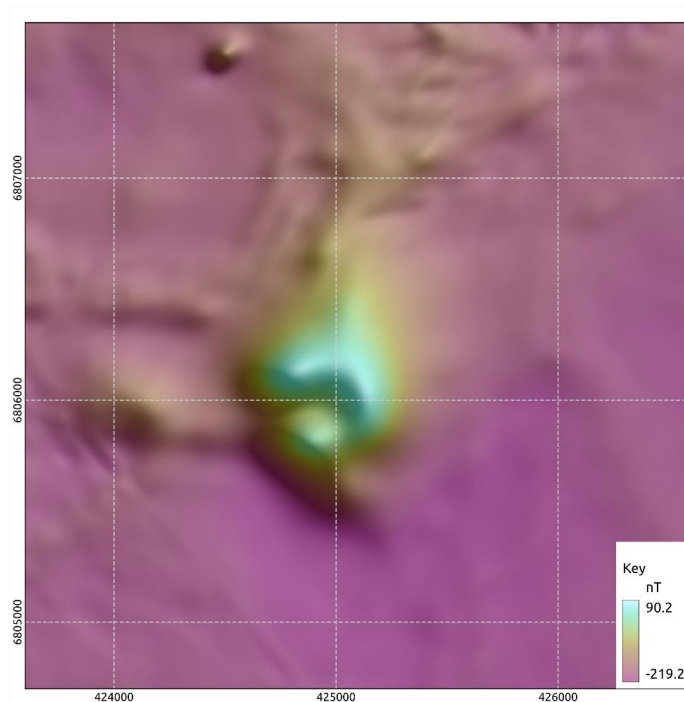
Figure 7. Field TMI data for the Callisto model.
