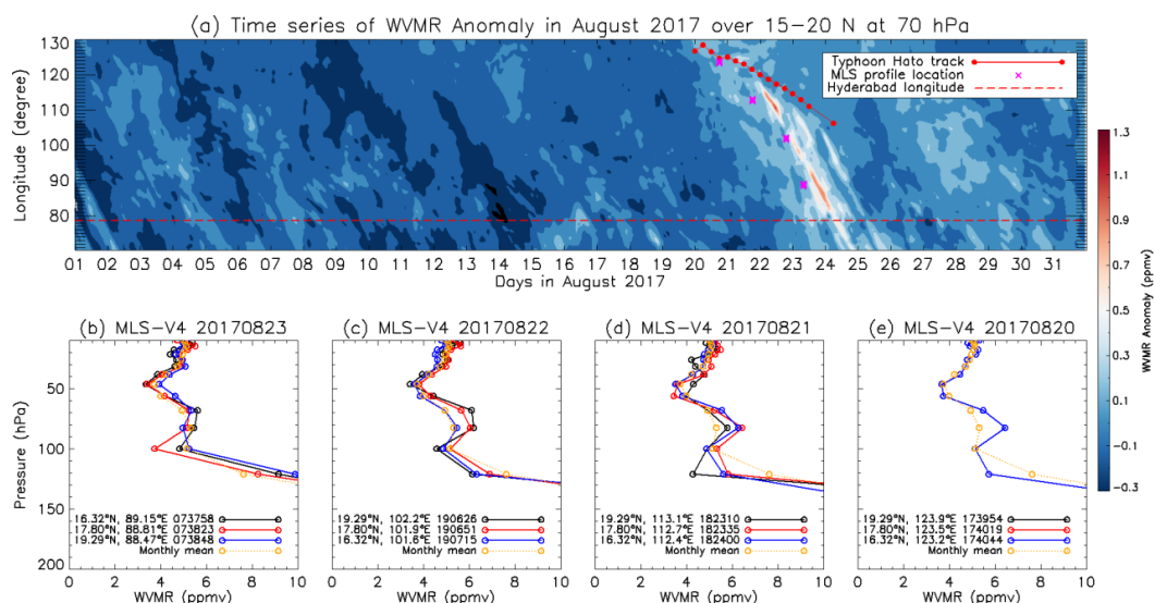
3 4 Figure 10: (a) Hovmöller plot for the anomaly in water vapour mixing ratio (WVMR) derived from ERA5 5 temperature and relative humidity at 70 hPa pressure level for August 2017. Anomaly is computed by 6 subtracting the monthly mean WVMR for each grid between 15° N and 20° N. Dashed red line marks the 7 longitude of TIFR-BF in Hyderabad. Red dots represent the track of typhoon Hato while magenta crosses 8 show the location of nearest MLS profiles on different dates. Vertical profiles of WVMR from MLS between 9 15° N and 20° N observed on (b) 23 August 2017, (c) 22 August 2017, (d) 21 August 2017, and (e) 20 August 10 2017 at different times in UTC shown by different colors in the legend. The profiles affected by clouds are 11 filtered out. The orange line with orange circles in each panel represents the mean MLS profile for August 12 2017 obtained by averaging all profiles located in the region bounded by 15°-20° N and 70°-130° E.
