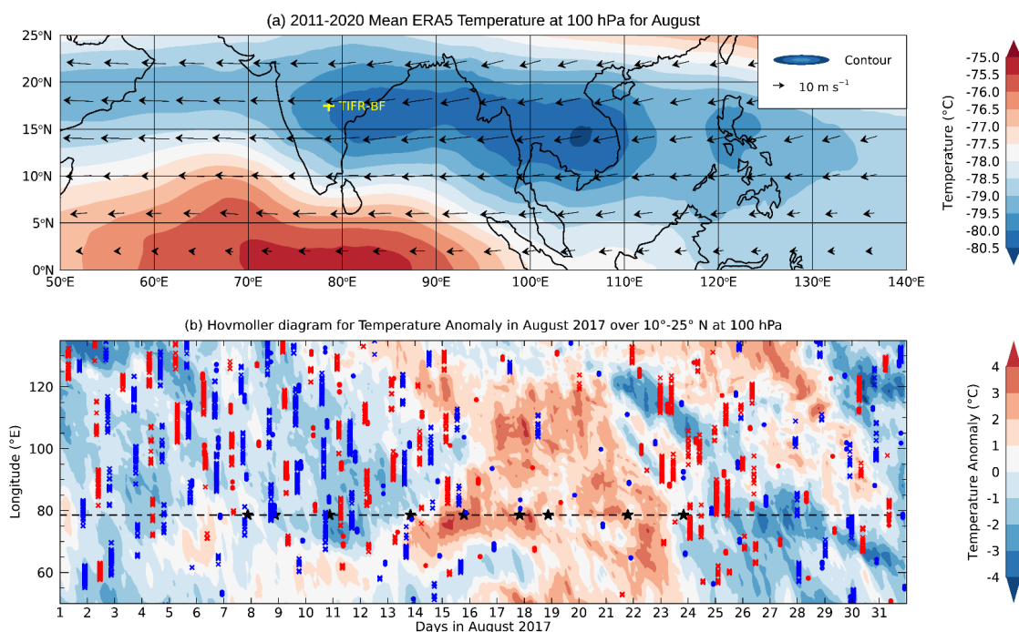
Figure 1: (a) Filled colour contour showing the 10-year (2011-2020) mean ERA5 temperature superimposed with wind vectors representing the mean ERA5 horizontal wind speed and direction at 100 hPa pressure level for the month of August. The yellow “plus” sign indicates the location of the TIFR-BF in Hyderabad, India. (b) Hovmöller plot for the anomaly in temperature from ERA5 temperature at 100 hPa pressure level for August 2017. The anomaly is computed by subtracting the monthly mean (for August 2017) temperature for each grid between 10° N and 25° N. The dashed horizontal black line marks the longitude (78.58° N) of the TIFR-BF with each black star on it showing the launch time of the balloon. The red (blue) filled circles and crosses superimposed on the filled colour contours represent the locations of cirrus cloud layers detected by CALIOP and CATS during daytime (nighttime), respectively, with their base altitude located at 16 km or above.
