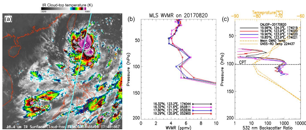
2 Figure 7: (a) 10.4 μm infrared cloud-top temperature from Himawari-8 at 17:40 UTC on 20 August 2017 3 showing the overshoots during the development phase of typhoon Hato . The cyan line represents the 4 CALIPSO orbit track that observed the overshoot on 20 August 2017 between 17:27 and 17:40 UTC. (b) Co- 5 located vertical profiles of water vapour mixing ratio (WVMR) from MLS on 20 August 2017 near the 6 overshoot region observed during daytime and night-time overpasses of Aura satellite. (c) Vertical profiles of 7 532 nm backscatter ratio obtained from the CALIOP on 20 August 2017 at around 17:40 UTC. Dashed 8 orange lines show the mean temperature profile obtained from GMAO along CALIPSO track and from 9 GNSS-RO at 22:44 UTC. Dashed horizontal black line represents the CPT.
