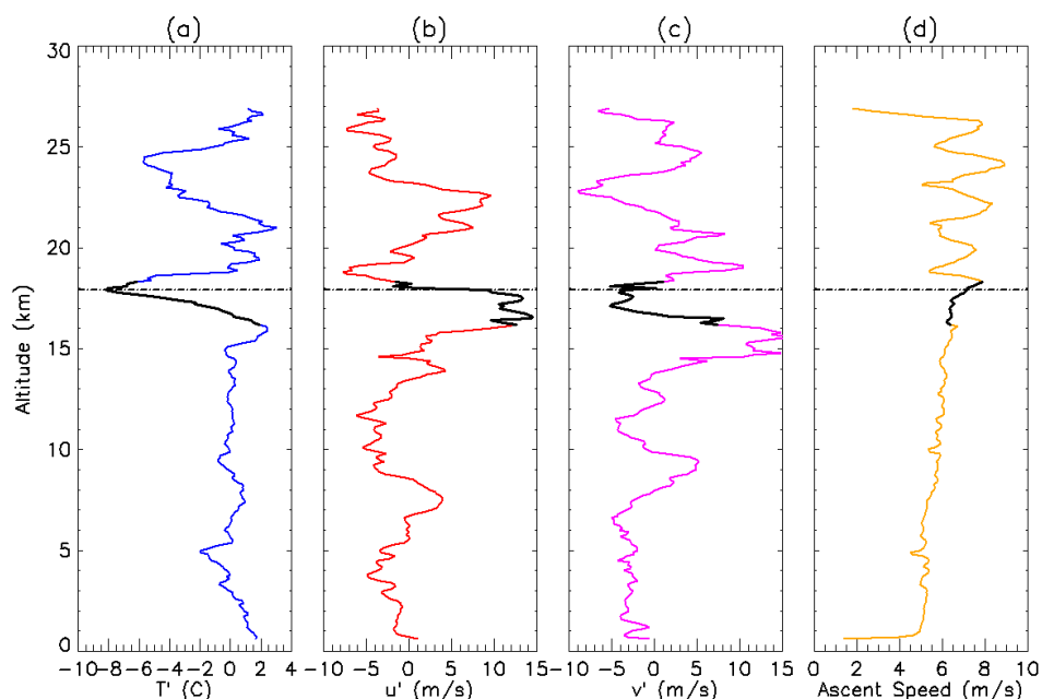
Figure 14: Vertical profile of (a) temperature anomaly, (b) zonal wind speed anomaly, (c) meridional wind speed anomaly and (d) ascent speed of the balloon observed on 23 August 2017. Anomalies are estimated by subtracting the monthly mean profile from the profile obtained on 23 August 2017. Mean profiles are obtained from all the radiosonde profiles at 00 UTC and Batal flights over Hyderabad for August 2017. The black dashed horizontal line in each panel denotes the location of the CPT (at 17.9 km) observed on 23 August 2017 at around 21:00 UTC from the balloon. Black shading in each profile shows the location of the tropopause cirrus cloud.
