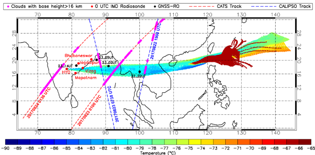
1 2 Figure 11: Filled coloured circles on the map show the temperature and location of the air parcel at every 3 hour along the back-trajectories run from the balloon measurement sites between 16 and 19 km on 23 August 4 2017 at 20:00 UTC. Red and blue dashed lines represent the nearest orbit tracks of CATS (on 24 August 2017 5 at 01:36 UTC and 23 August 2017 at 01:00 UTC) and CALIPSO (23 August 2017 at 07:38 UTC and 22 6 August 2017 at 19:00 UTC), respectively, with respect to the air parcels. Filled magenta circles superimposed 7 on the orbit tracks represent the locations of cirrus cloud layer with base altitude greater than 16 km. Red 8 filled circles on the map show the locations of the IMD stations from where daily radiosondes are launched at 9 00 UTC. Black filled circles show the locations of available GNSS-RO temperature profiles closest in time and 10 space with CATS and CALIPSO overpasses.
