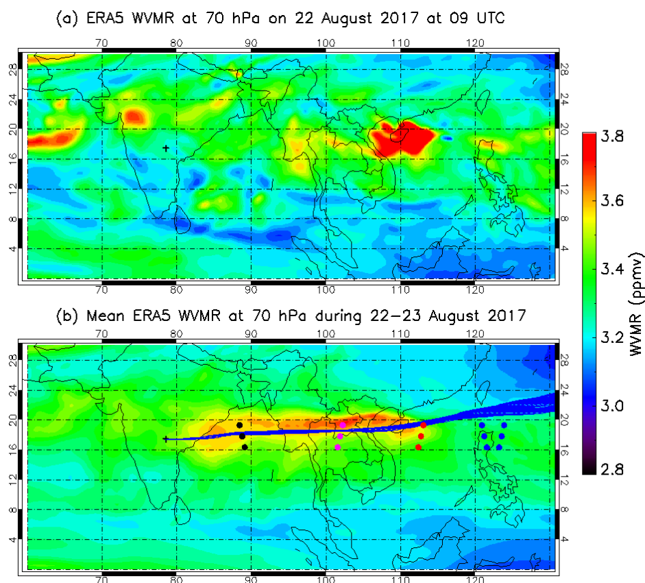
Figure 9: (a) Spatial map of water vapour mixing ratio (WVMR) derived from ERA5 data at 70 hPa level on 22 August 2017 at 09:00 UTC showing large enhancement over the South China Sea. (b) Average water vapour mixing ratio derived from ERA5 for 22 and 23 August 2017 at 70 hPa with back-trajectories superimposed on it. Nearest MLS footprints with respect to the back-trajectories between 16° and 20° N on 20, 21, 22 and 23 August 2017 are represented by blue, red, magenta, and black filled circles, respectively.
