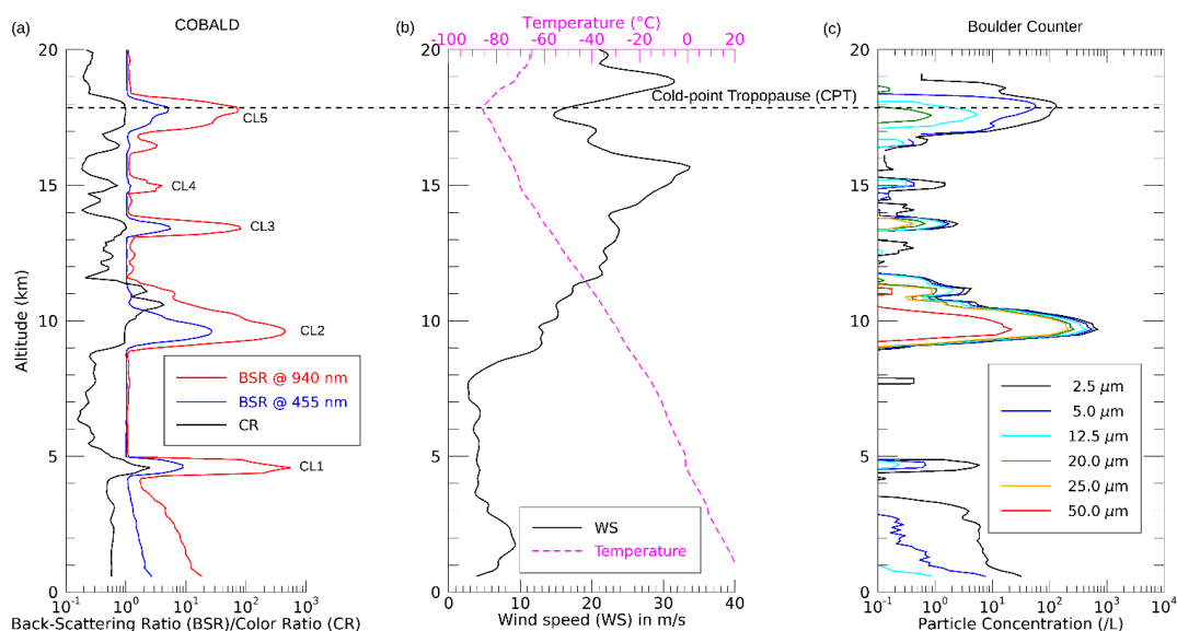
3 4 Figure 2: Vertical profile of (a) backscatter ratio at 455 nm (blue line), 940 nm (red line) and colour ratio 5 (black line) obtained from COBALD, (b) temperature (magenta dashed line) and wind speed (black line) 6 from radiosonde with horizontal dashed black line showing the CPT and (c) cumulative particle number 7 concentration for particles having radius greater than 2.5 (black line), 5 (blue line), 12.5 (cyan line), 20 (green 8 line), 25 (yellow line) and 50 \mu\text{m} (red line) obtained from the Boulder Counter measurements on 23 August 9 2017 over Hyderabad, India during BATAL campaign. The vertical resolution is 100 m for each profile.
