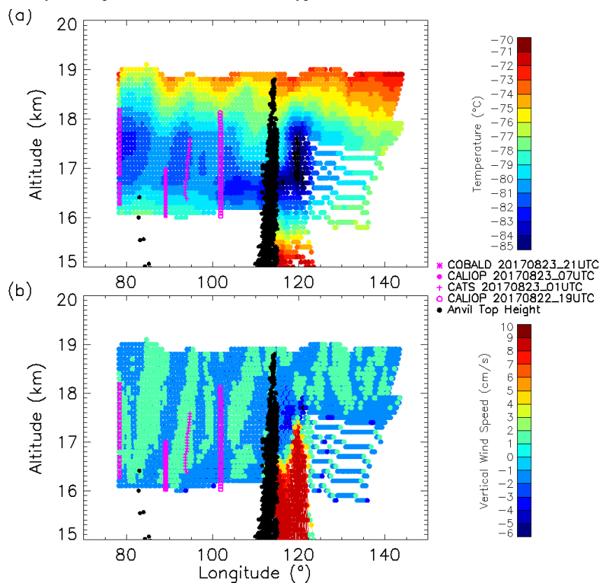
3 4 Figure 12: (a) Temperature history of the air parcels along the back-trajectories run from the balloon 5 measurement sites between 16 and 19 km on 23 August 2017. Each filled coloured circle represents 6 temperature value at every 100 m vertical resolution at each hour. (b) Same as (top) but for the vertical wind 7 derived from the location and time of the back-trajectories. Different magenta symbols represent the location 8 of the layered cirrus clouds observed near the tropopause from CALIOP, CATS and balloon measurements 9 near co-located in space and time with respect to the back-trajectories. The locations of anvil cloud top 10 altitude are represented by black dots. 11
