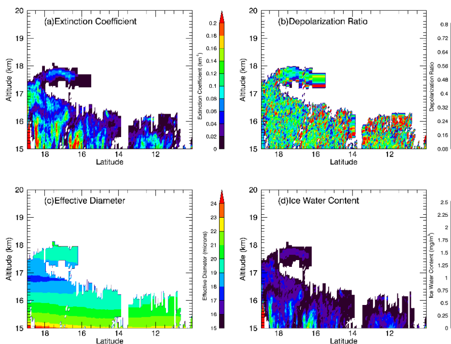
7 8 Figure 8: Optical and microphysical properties of cirrus clouds observed by CALIOP on 22 August 2017 at 9 19:00 UTC over Southeast Asia represented by black stripes in Fig. 6. 10
