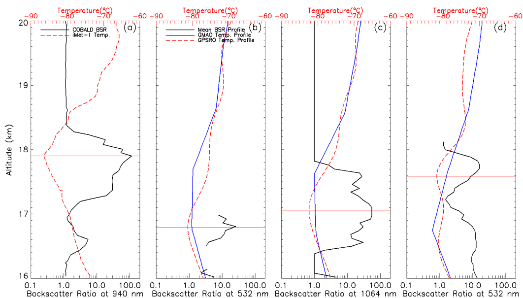
2 Figure 13: Vertical profile of scattering ratio (shown by black line) obtained from (a) COBALD data on 23 3 August 2017 at around 20:40 UTC over 17.45° N, 78.31° E, (b) CALIOP on 23 August 2017 at around 07:38 4 UTC over 16.99° N, 88.88° E, (c) CATS on 23 August 2017 at around 00:59 UTC over 17.01° N, 92.68° E and 5 (d) CALIOP on 22 August 2017 at around 19:07 UTC over 16.99° N, 101.68° E. CALIOP and CATS profiles 6 intersecting with the back-trajectories are averaged between 16° and 18° N. Blue line in (b), (c) and (d) 7 represents the mean temperature profile obtained by averaging the corresponding MERRA-2 temperature 8 profiles provided with CALIOP and CATS data. Dashed red line shows the co-incident and co-located 9 temperature profile obtained from (a) radiosonde measurement, (b) COSMIC GPS RO on 23 August 2017 at 10 05:07 UTC over 20.13° N, 87.37° E, (c) COSMIC GPS RO on 23 August 2017 at 02:33 UTC over 18.29° N, 11 90.87° E, (d) COSMIC GPS RO on 22 August 2017 at 23:42 UTC over 16.63° N, 100.04° E. Horizontal red 12 line in each panel marks the CPT.
