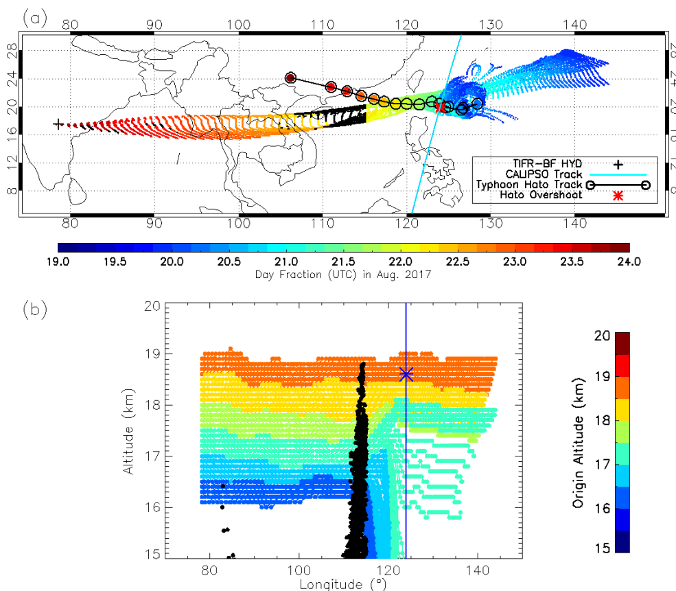
6 7 Figure 5: (a) Five-day back-trajectories initialized on 23 August 2017 at 20:00 UTC from the balloon 8 measurement locations at different altitudes between 16 and 19 km represented by colored dots as a function 9 of latitude and longitude with colour showing the day fraction. The locations of deep convective anvil tops 10 observed after 21 August 2017 from the Himawari-8 brightness temperature images at 10.4 \mu\text{m} wavelength 11 channel that intersected the back-trajectories are shown by black dots. Typhoon Hato track is shown by 12 black outlined coloured circles connected by black line with colour showing the day fraction. The night-time 13 CALIPSO orbit track on 20 August 2017 between 17:27 and 17:40 UTC is shown by cyan line with the 14 location of the overshooting cloud top shown by red asterisk. (b) Five day back-trajectories represented as a 15 function of longitude and altitude with colour showing their origin altitude. The locations of the anvil top 16 altitude that intersected with the back-trajectories are represented by black dots. The locations of CALIPSO 17 overpass and the overshooting cloud top altitude are shown by blue vertical line and blue asterisk, 18 respectively.
