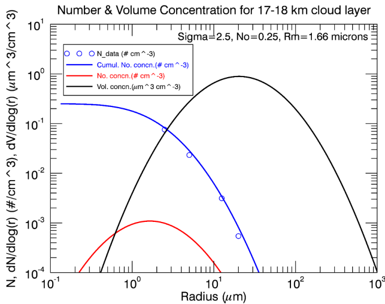
2 Figure 4: Particle size distribution of the cloud layer (CL5) observed between 17 and 18 km from the Boulder 3 Counter measurements on 23 August 2017. Particle number concentration and volume concentration are 4 shown by solid red and black lines, respectively. Measured cumulative number concentration is shown by 5 open blue circles while the solid blue line is log-normal fit to it. The width of the distribution is given by 6 Sigma, which is about 2.5, total particle concentration ( N_0 ) in the mode is 0.25 \text{ per cm}^{-3} and R_m = 1.66 \mu\text{m} is 7 the median radius.
