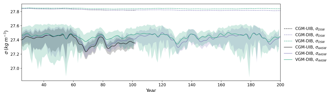
Figure 7. Potential density on the Weddell Sea continental shelf between 30°W and 0°W. \sigma_{AASW} corresponds to the average monthly density above the thermocline (solid lines) and \sigma_{DSW} corresponds to the average monthly density below the thermocline (dashed lines). Both quantities are low-pass-filtered in time with a cutoff of 3 months and the running annual minimum and maximum are bounded with shading. The thermocline depth is calculated as in Hattermann (2018).
