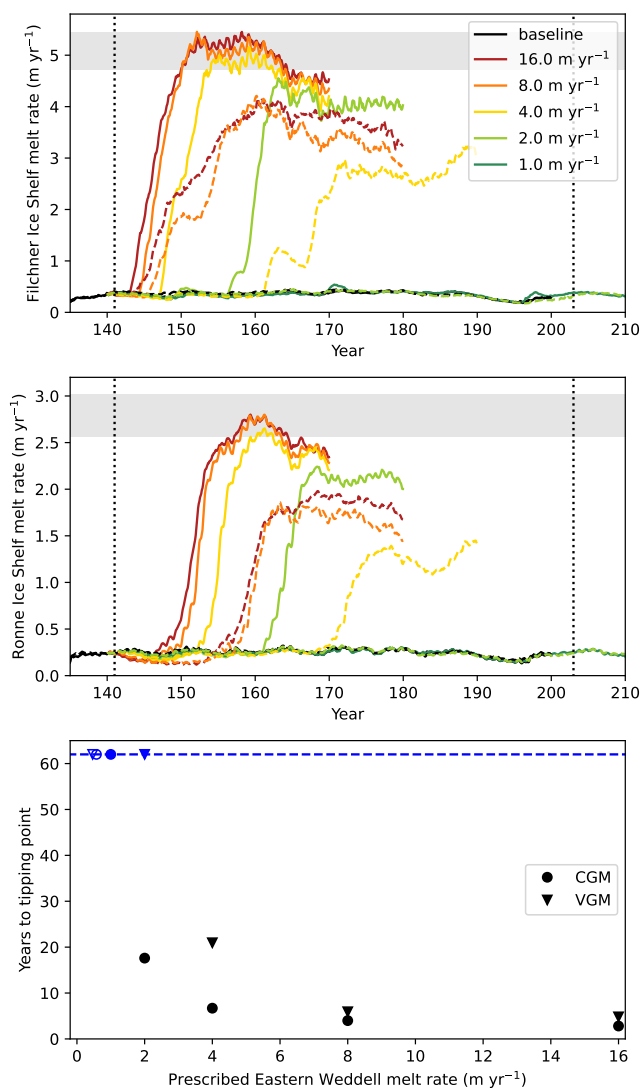
Figure 11. Results of branch runs prescribing melt rates at eastern Weddell Sea ice shelves. All branch runs were begun in year 141 and stopped after 62 years (one complete CORE-II cycle), indicated by vertical dotted lines. a) Area-averaged melt rate modeled at Filchner Ice Shelf. CGM-DIB is shown with solid lines, and VGM-DIB is shown with dashed lines. The baseline simulations are shown in black. The gray shading indicates the range of melt rates simulated after the regime change in the CGM-UIB run. b) Area-averaged melt rate modeled at Ronne Ice Shelf. Line styles same as for panel a. c) Number of years to occurrence of FRIS tipping point as a function of the melt rate prescribed at the eastern Weddell Sea ice shelves for both CGM-DIB (circles) and VGM-DIB (triangles). The open symbols represent the baseline runs. The initiation of the FRIS tipping point is defined here as the first year in which the modeled Filchner Ice Shelf melt rate exceeds twice the mean baseline value. The blue symbols on the blue dashed line indicate simulations that did not reach the FRIS tipping point within a complete CORE-II forcing cycle.
