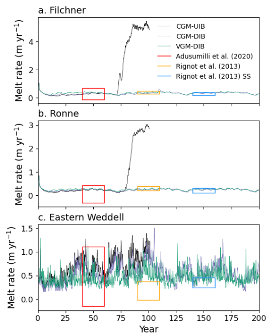
Figure 1. Time series of modeled melt rates averaged over (a) Filchner Ice Shelf, (b) Ronne Ice Shelf, and (c) Eastern Weddell ice shelves consisting of Brunt, Stancomb-Wills, Riiser-Larsen, Quar, and Ekström ice shelves. The mean \pm standard deviation melt rates in each region are represented with boxes placed at arbitrary years for the following: a 2003-2008 satellite-derived estimate (Rignot et al., 2013), the melt rates required to maintain 2003-2008 steady state ice shelf extent (SS) (Rignot et al., 2013), and a 2010-2018 satellite-derived estimate (Adusumilli et al., 2020).
