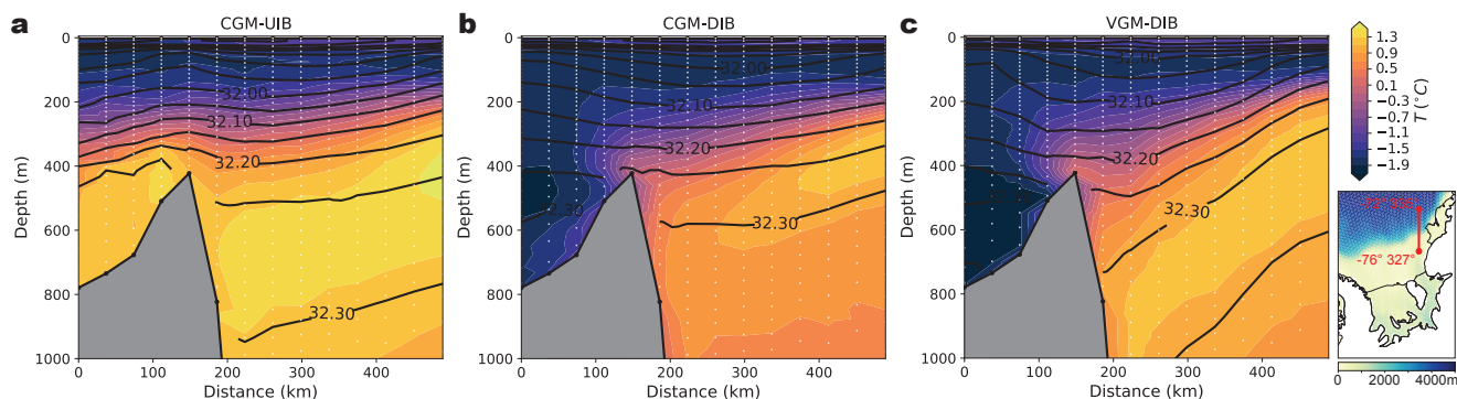
Figure 9. Cross sections of temperature (colors) and potential density anomalies (contours, referenced to 1000 db) along the Filchner Trough averaged over years 91-100 for CGM-UIB (a) and years 191 to 200 for CGM-DIB (b) and VGM-DIB (c). White dots indicate model data points used to construct the cross-section. [TODO: increase font size; replace single year averages with decadal averages; create cleaner inset map and move somewhere better; replace screengrab with tidied up version; add panel labels]
