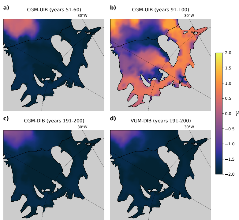
Figure 5. Seafloor potential temperature. a) CGM-UIB run averaged over years 51-60. b) CGM-UIB run averaged over years 91-100, after the melt regime change has occurred. c) CGM-DIB run averaged over years 191-200. d) VGM-DIB run averaged over years 191-200.
