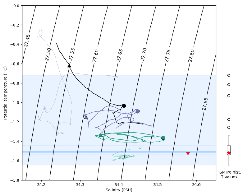
Figure 12. Comparison of modeled Weddell Sea continental shelf water mass properties in E3SM and CMIP5 models used in the ISMIP6 intercomparison. Observed temperature and salinity from WOA are indicated by the red star. The modeled temperature and salinity are represented by their 20-year-mean trajectories, with initial twenty-year average indicated by an x. The three primary simulations described in this paper are shown with thick lines and colored symbols (CGM-UIB: black; CGM-DIB: purple; VGM-DIB: green). Circles mark the average over years 42-62 (final twenty years before the end of first the CORE-II cycle) and triangles for the average over years 70-90 (final two complete decades before CGM-UIB begins regime shift). The equivalent fully-coupled E3SM preindustrial spin-ups from Comeau et al. (2022) are indicated by thin lines in corresponding colors (coupled CGM-DIB: purple; coupled VGM-DIB: green), covering 200 years. The temperature range from the ensemble of CMIP5 historical simulations evaluated by Barthel et al. (2020) is indicated by the blue shading, and also represented in more details by the box and whisker plot on the right-hand side (with outliers as circles). The CMIP5 models selected for ISMIP6 are added for context (top 3: blue lines, top 6: dashed blue lines).
