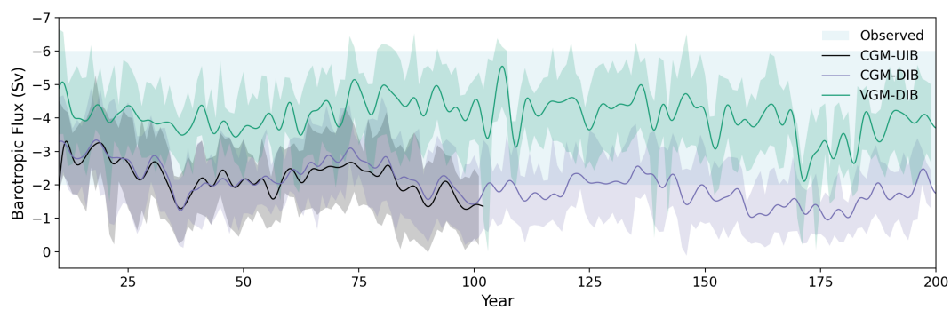
Figure 10. Barotropic transport in the Weddell Gyre for each simulation. The flux is computed from monthly-averaged velocities across Transect C in Wang et al. (2012) to facilitate comparison with reanalysis ( 75^{\circ}\text{S} , 30^{\circ}\text{W} to 72^{\circ}\text{S} , 25^{\circ}\text{W} ). The barotropic fluxes are low-pass-filtered in time with a cutoff of 3 months and the running annual minimum and maximum are bounded with shading. Range from higher resolution models and reanalysis (Mazloff et al., 2010; Wang et al., 2012) shown with blue shading.
