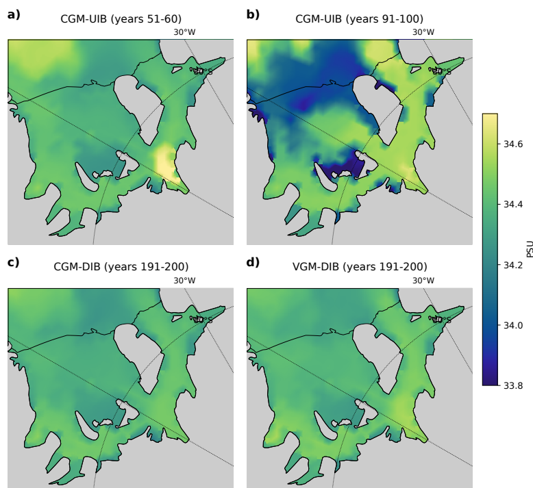
Figure 6. As in Fig. 5 but showing sea floor salinity.
