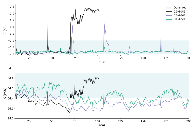
Figure 8. Time series of temperature (a) and salinity (b) at observational site M31W (Ryan et al., 2017) located in the Filchner Trough. The observational range is shaded.
