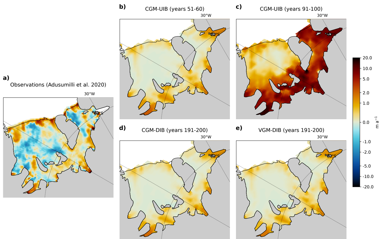
Figure 2. FRIS basal melt rates ( \text{m yr}^{-1} of freshwater). a) basal ice-shelf melt rate from Adusumilli et al. (2020). b) CGM-UIB run averaged over years 51-60. c) CGM-UIB run averaged over years 91-100 after the melt regime change has occurred. d) CGM-DIB run averaged over years 191-200. e) VGM-DIB run averaged over years 191-200. Note the nonlinear color scale.
