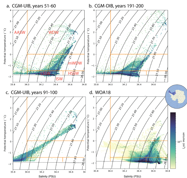
Figure 4. Temperature-salinity distribution for the western Weddell Sea continental shelf for depths shallower than 1000 m. a) CGM-UIB run averaged over years 51-60. b) CGM-DIB run averaged over years 191-200. c) CGM-UIB run averaged over years 91-100, after the melt regime change has occurred. d) Observations from World Ocean Atlas 2018. Boundaries for water masses are shown with orange lines and follow Naughten et al. (2018), renamed for Weddell Sea water masses, consistent with Kerr et al. (2018): Antarctic Surface Water (AASW), Weddell Deep Water (WDW), modified Weddell Deep Water (mWDW), Low Salinity Shelf Water (LSSW), High Salinity Shelf Water (HSSW), and Ice Shelf Water (ISW).
