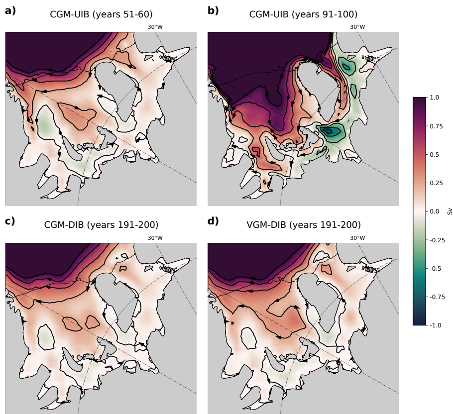
Figure 3. FRIS barotropic streamfunction ( Sv ) modeled by E3SM. Streamlines show direction of depth-integrated transport, spaced at 0.25 Sv intervals. a) CGM-UIB run averaged over years 51-60. b) CGM-UIB run averaged over years 91-100 after the melt regime change has occurred. c) CGM-DIB run averaged over years 191-200. d) VGM-DIB run averaged over years 191-200.
