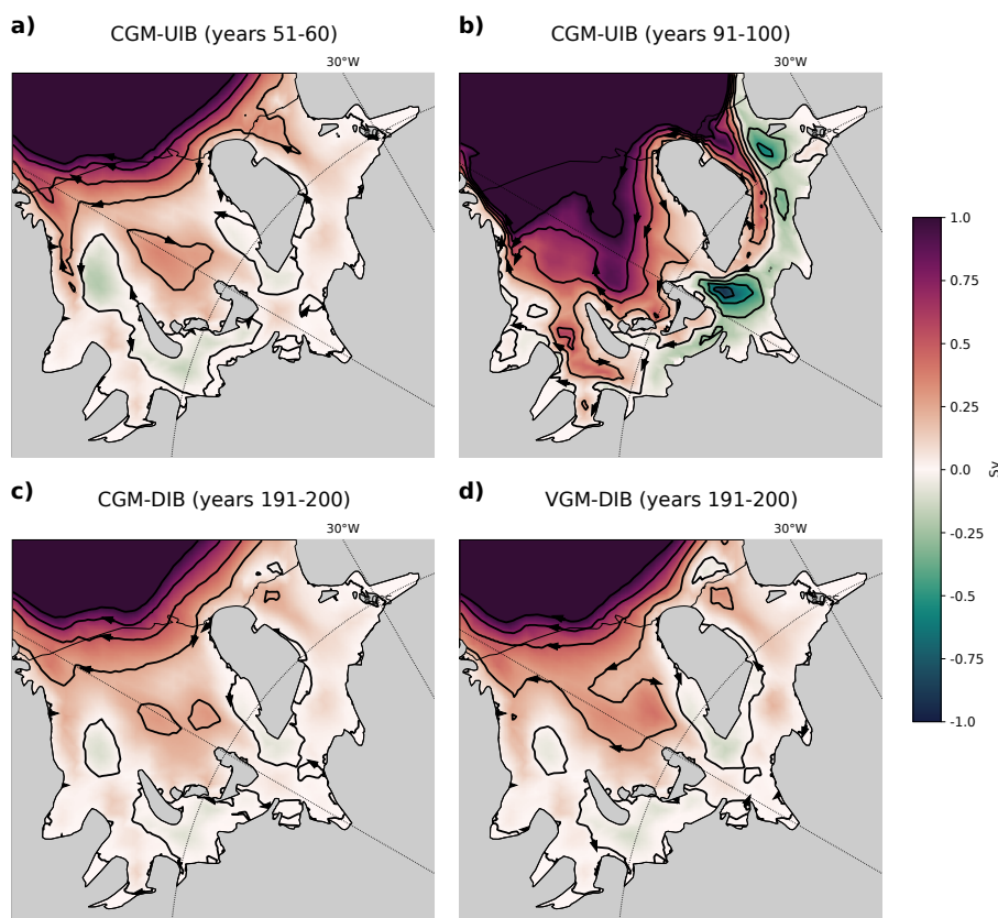
Figure 4. Modeled FRIS barotropic streamfunction (Sv) modeled by E3SM . Streamlines show direction of depth-integrated transport, spaced at 0.25 Sv intervals. a) CGM-UIB run averaged over years 51-60. b) CGM-UIB run averaged over years 91-100 after the melt regime change has occurred. c) CGM-DIB run averaged over years 191-200. d) VGM-DIB run averaged over years 191-200.
