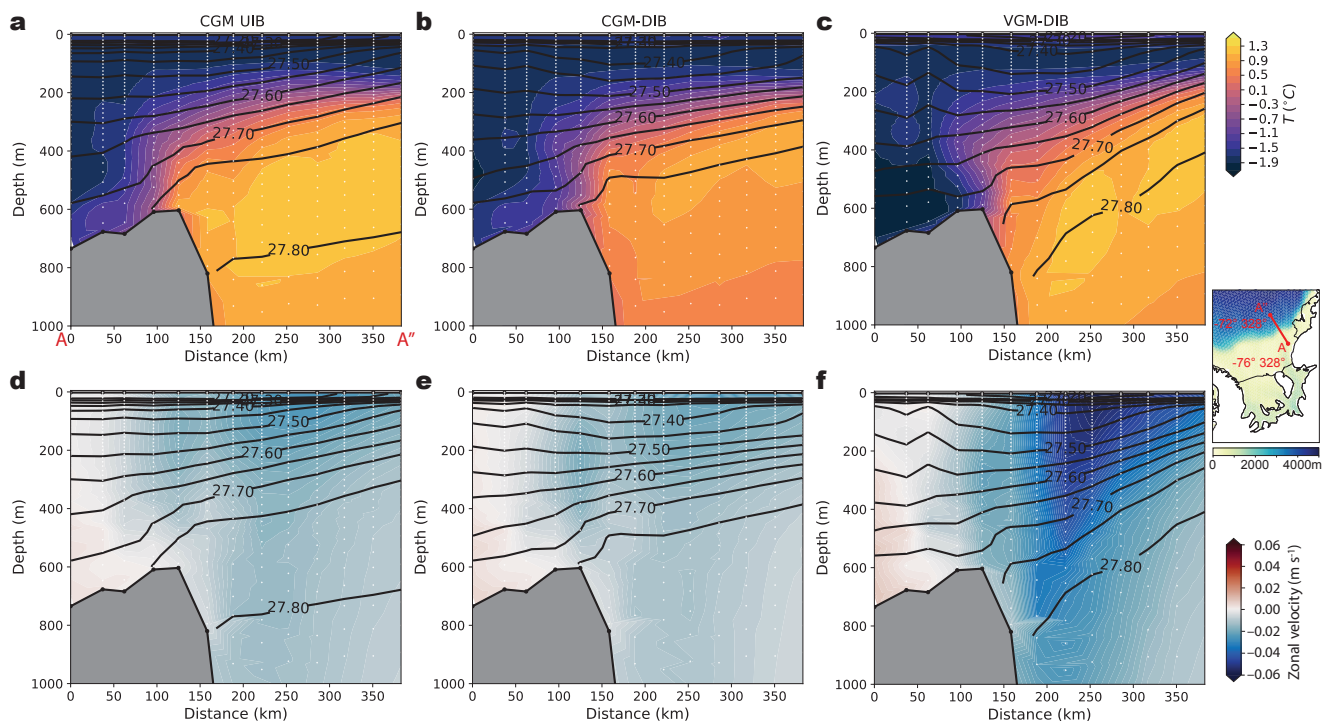
Figure 10. Cross sections of temperature (colors) and potential density anomalies (contours, referenced to 1000 db) along across the continental shelf break at the Filchner Trough averaged over years 91-100-51 to 60 (prior to melt regime change) for CGM-UIB (a,d) and years 191 to 200 for CGM-DIB (b,e) and VGM-DIB (c,f). Panels a-c show temperature (colors) and potential density anomalies (contours, referenced to the surface). Panels d-f show eastward zonal velocity (colors) with potential density anomalies as in a-c. White dots indicate model data points used to construct the cross-section. Inset map shows location of transect A-A", as does Fig. 1.
