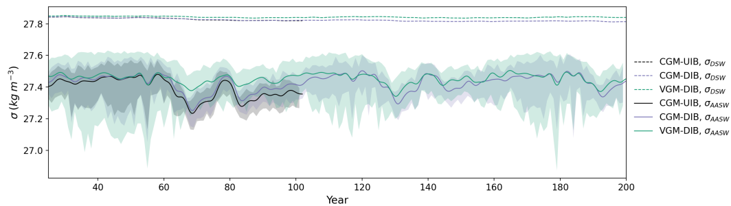
Figure 8. Potential density on the Weddell Sea continental shelf between 30°W and 0°W. \sigma_{AASW} corresponds to the average monthly density above the thermocline (solid lines) and \sigma_{DSW} corresponds to the average monthly density below the thermocline (dashed lines). Both quantities are low-pass-filtered in time with a cutoff of 3 months and the running annual minimum and maximum are bounded with shading. The thermocline depth is calculated as in Hattermann (2018).
