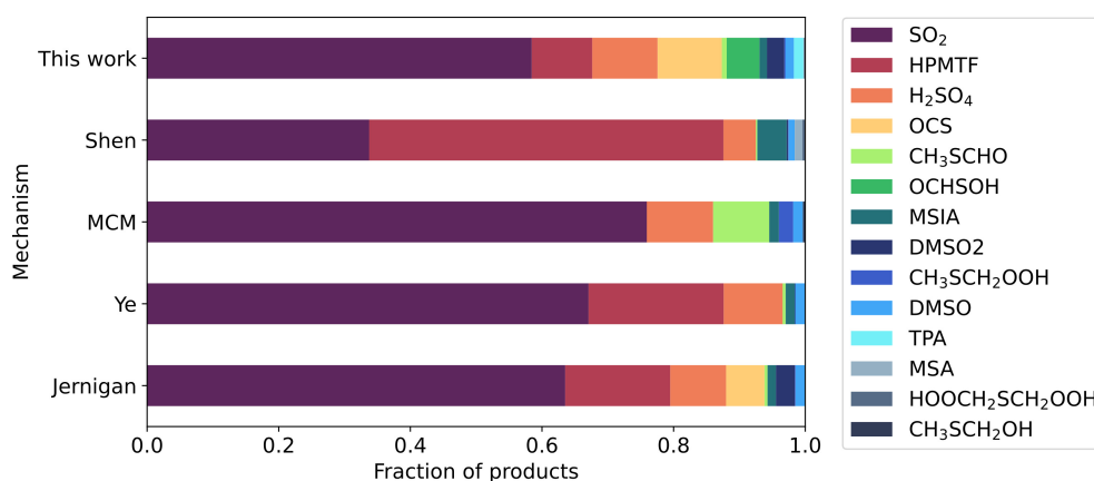
Figure 8. The distribution of DMS oxidation products from the marine boundary layer run for each mechanism, based on the average concentration of the products over the last two days of the run. The data from this figure is included as percentages in the supplementary (Table S8).
