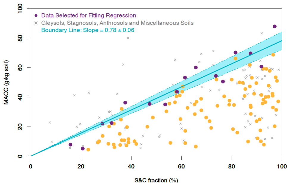
185 Figure 1: Boundary analysis of mineral associated organic C (MAOC) versus silt & clay content of the fine soil based on the Begill et al. (2023) dataset, without Gleysols, Stagnosols, Anthrosols, and “miscellaneous” soils (indicated by grey crosses). The boundary line (in blue) is based on the 90 th percentile (purple dots) with 95% confidence interval (blue shade). Orange dots are all other soils in the dataset, including Cambisols, Luvisols, Phaeozems, Regosols, and Vertisols. Note that a much weaker trend between MAOC and the silt & clay content is visible for the subgroup of soils with grey crosses, indicating the presence of non-texture dependent factors (e.g. anoxic conditions) determining the measured MAOC content in those soils.
