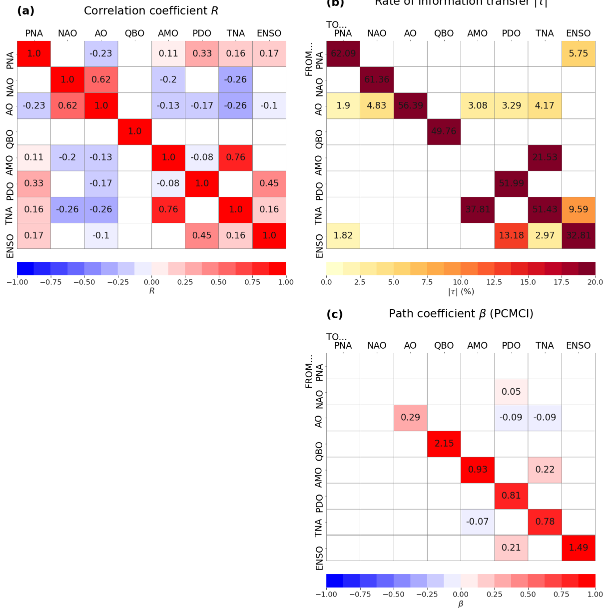
Figure 8. Results from the real-world case study: (a) correlation coefficient, (b) rate of information transfer (LKIF, absolute value), and (c) maximum path coefficient (PCMCI) when using 3 lags (0 to 2 months). Only significant values at the \alpha = 5\% level are shown.
