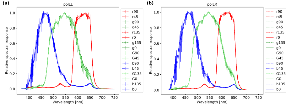
Figure 8. Relative spectral response function with uncertainty for the different color and polarization channels of the poLL camera (a) and poLR camera (b).
