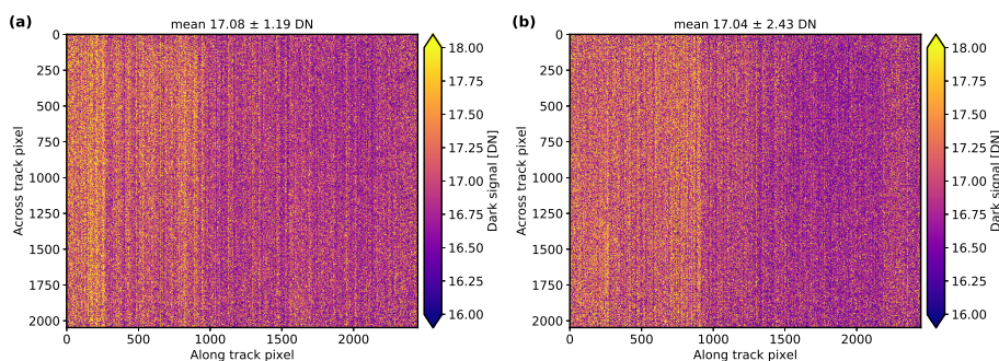
Figure 3. Spatial distribution of dark signal averaged over 100 dark measurements with 50 frames each at an exposure time of 5ms and constant temperature for the poLL camera (a) and poLR camera (b).
