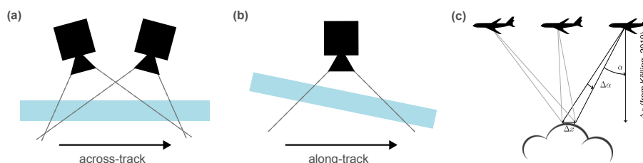
Figure 2. (a) and (b) Installation geometry of the two polarization resolving cameras. The window in front of the cameras is shown in light blue, the dashed lines indicate the field of view of the cameras. (c) Observation geometry (Figure from Pörtge et al. (2023)).
