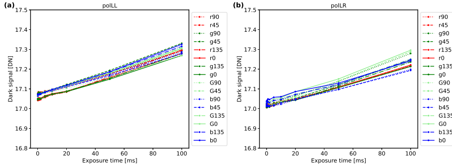
Figure 5. Exposure time dependence of dark signal averaged over 50 frames at constant temperature for the polLL camera (a) and polLR camera (b). The different lines show the different color and polarization channels.
