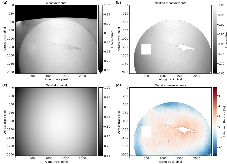
Figure 10. Flat-field model results for the red channel of the poLL camera. (a) Mean normalized, dark signal corrected total intensity. (b) Part of measurement in (a) used in the vignetting correction (removed LIS upper hemisphere, reflections, and dirt affected areas). (c) Vignetting model fitted to the measurements. (d) Relative difference between vignetting model and measurements.
