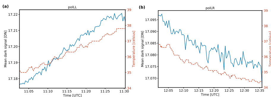
Figure 4. Temperature dependence of dark signal averaged over 50 frames for each temperature at an exposure time of 5ms for the poLL camera (a) and poLR camera (b). The red dashed curves indicate the temperature variations, the blue solid curve shows mean dark signal.
