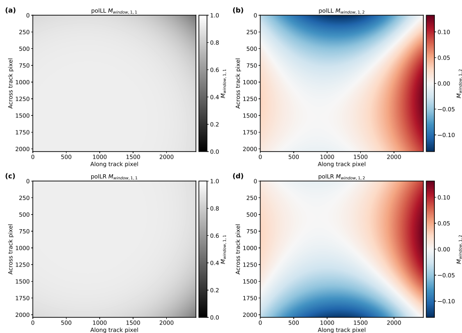
Figure 9. 1,1- and 1,2-components of the Mueller matrix describing the window for the red channel of the poLL and poLR camera.
