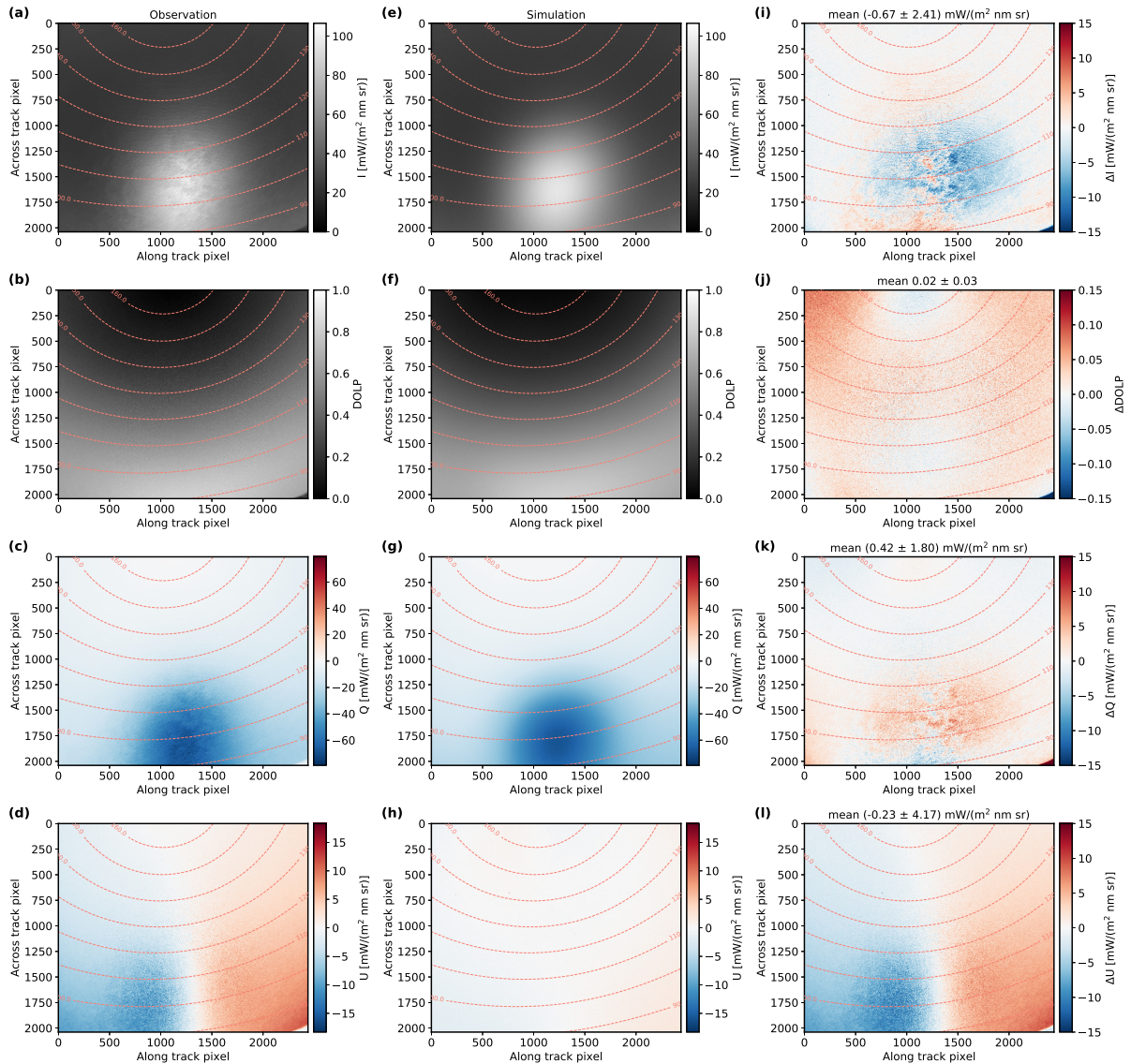
Figure 12. (a) - (d) Example sunglint observation of the green channel of the polLR camera on 2020-01-22 at 16:20 UTC. (e) - (h) Sunglint simulation corresponding to the observation in (a) - (d). (i) - (l) Absolute difference of the sunglint observation and simulation in (a) - (d) and (e) - (h). Mean and standard deviation of the absolute differences are given in the respective titles. (a), (e), (i) Total intensity. (b), (f), (j) Degree of linear polarization, (c), (g), (k) Q component of the Stokes vector. (d), (h), (l) U component of the Stokes vector. The dashed lines indicate scattering angles.
