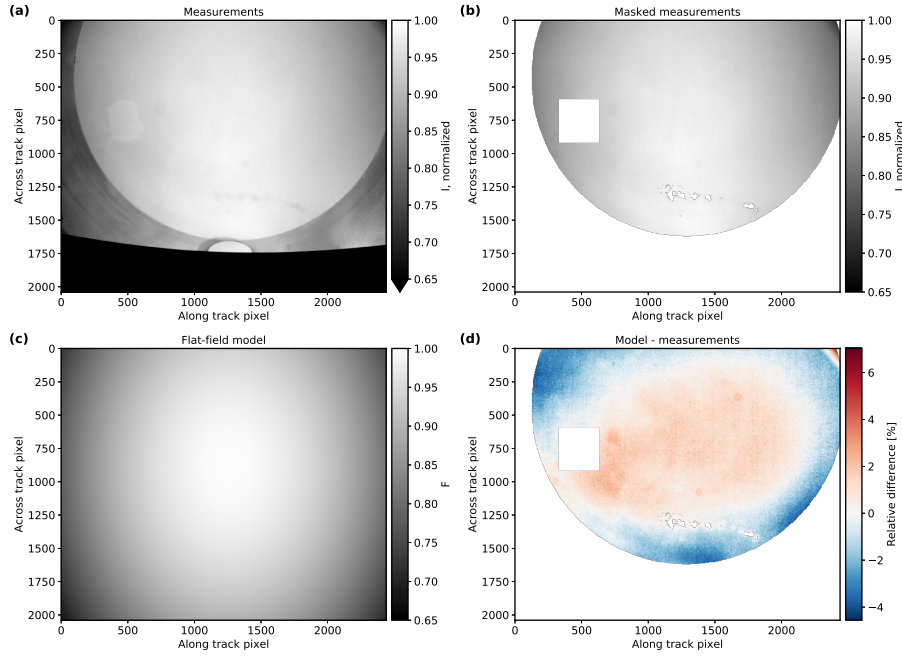
Figure 11. Flat-field model results for the red channel of the poLR camera. (a) Mean normalized, dark signal corrected total intensity. (b) Part of measurement in (a) used in the vignetting correction (removed LIS upper hemisphere, reflections, and dirt affected areas). (c) Vignetting model fitted to the measurements. (d) Relative difference between vignetting model and measurements.
