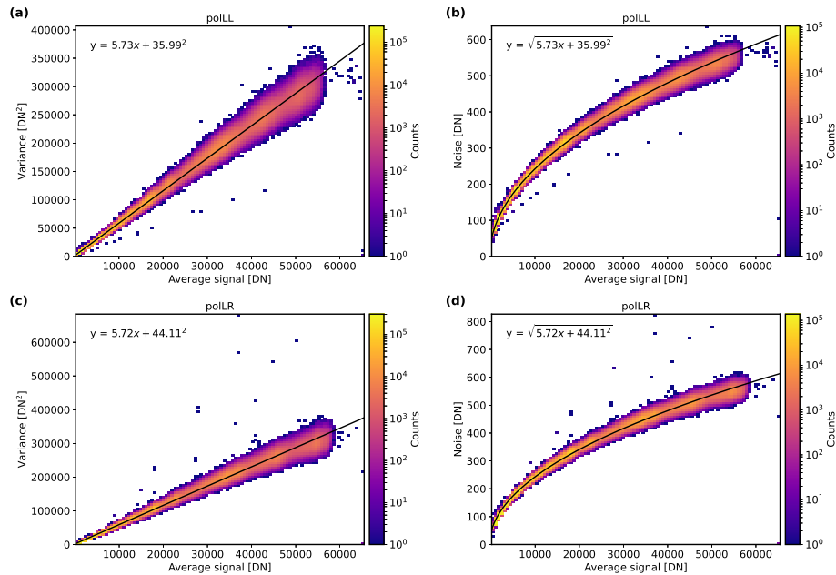
Figure 7. Noise characteristics of the r90 channel of the poLL camera ((a) and (b)) and the poLR camera ((c) and (d)). Panels (a) and (c) show two-dimensional histograms of the variance as a function of average dark signal corrected signal and panels (b) and (d) the noise. The solid black lines denote the least-squares fit of the Poisson model given by the equation on the respective panel.
