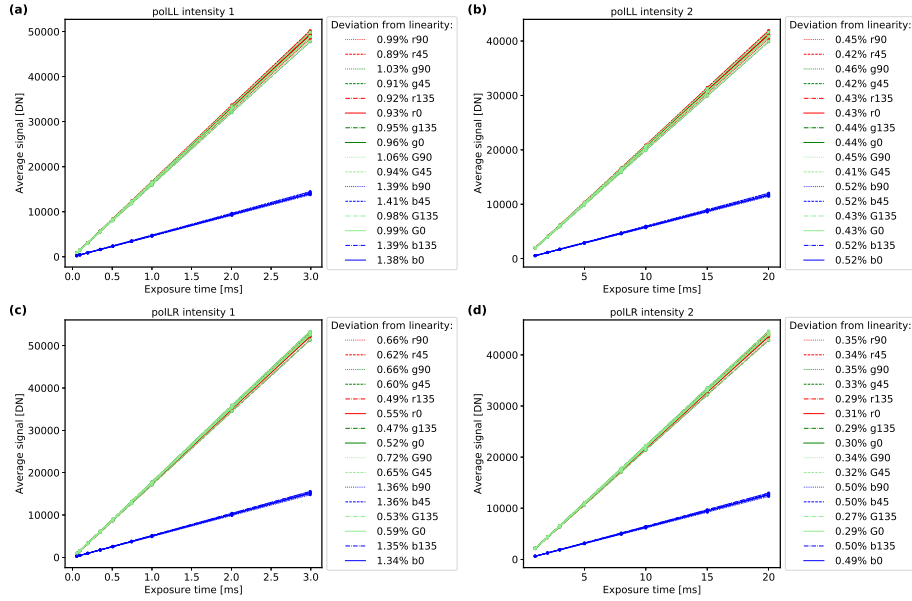
Figure 6. Linearity of mean radiometric signal S_0 with exposure time for the different channels of the polLL camera ((a) and (b)) and the polLR camera ((c) and (d)) for two different intensities of the large integrating sphere. The dots indicate the observed signal, the lines are a linear fit assuming a perfectly linear sensor. The deviation of the observed signal of each channel from the linear model is given in the legends.
