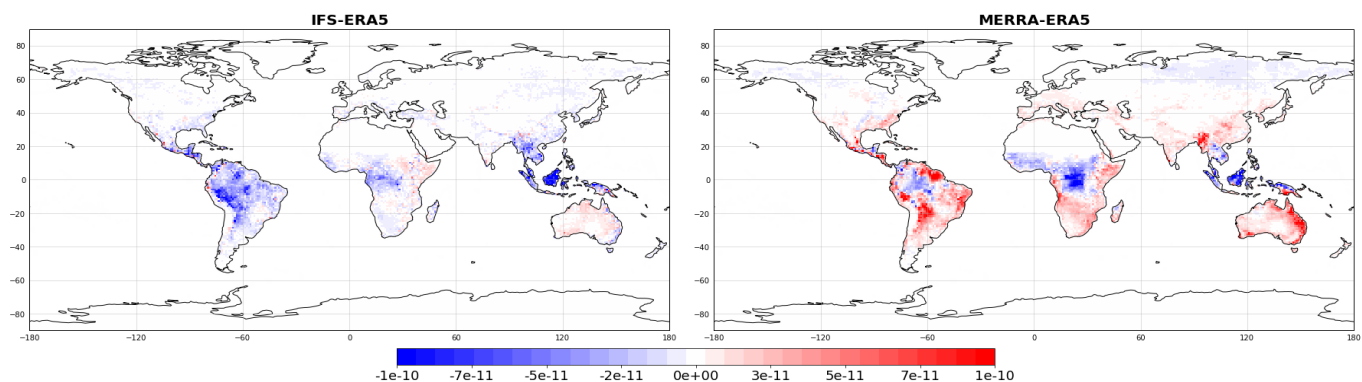
Figure 9. Annual mean isoprene difference ( \text{kg/m}^2/\text{s} ) between S1-IFS and reference simulation (left) and between S1-MERRA and reference simulation (right).
