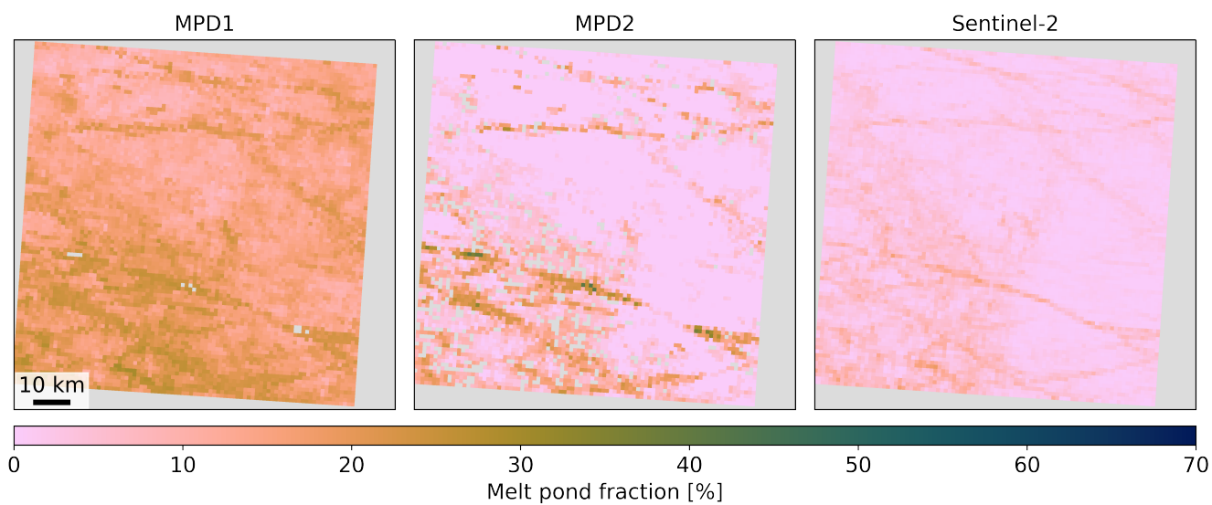
Figure A4. Same as Figure 15 but for an example from June 17, 2021 at approximately 81°N and 131°W. All maps share the same scale and color map.
