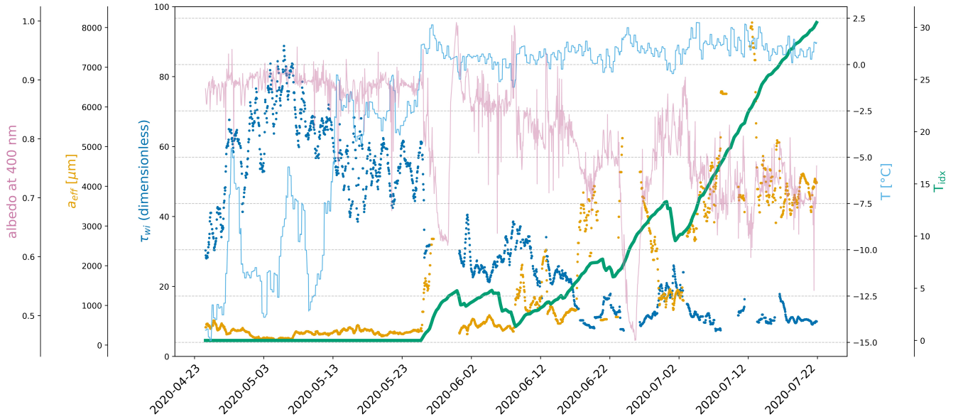
Figure 6. Albedo at 400 nm (pink, thin solid line) measured by the radiation station 2020R12, effective grain size a_{eff} (orange, dots) and optical thickness \tau_{wi} (dark blue, dots) retrieved from the spectral albedo measurements of the radiation station, 2-m air temperature (light blue, thin solid line) from ERA5, and the temperature index T_{idx} (green, thick solid line) derived from the air temperature.
