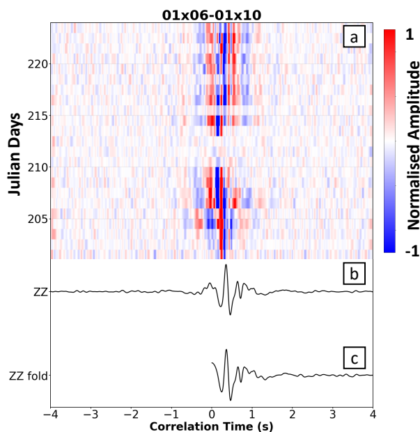
Figure 2. (a) Daily ZZ correlation functions plotted as a correlogram for station pair 01x06-01x10 (an inter-station distance of 850 m). (b) Stack of the ZZ correlation functions for the whole month, and (c) the final folded ZZ correlation function for station pair 01x06-01x10. Data are filtered between 1 Hz and 7 Hz.
