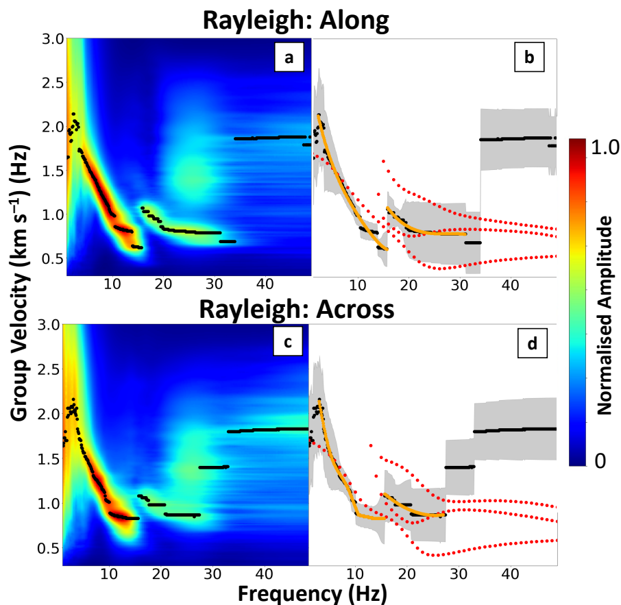
Figure 5. Left: stacked dispersion diagrams for Rayleigh waves for (a) along and (c) across flow stations, with the maximum amplitude shown by the black dots. Right: The maximum group velocity (black) and error ( \pm one standard deviation). Orange shows the smoothed values used as the input for MCMC inversion. Red dots are the forward-modeled dispersion curves obtained from a velocity model generated using only the fundamental mode.
