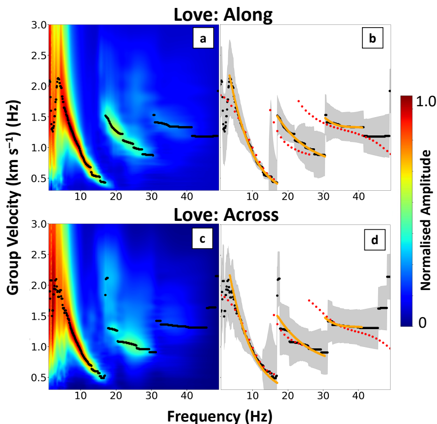
Figure 4. Left: stacked dispersion diagram for Love waves for (A) along and (C) across flow stations, with the maximum amplitude shown by the black dots. Right: The maximum group velocity (black) and error ( \pm one standard deviation). Orange shows the smoothed values used as the input for Markov Chain Monte Carlo inversion. Red dots are the forward-modeled dispersion curves.
