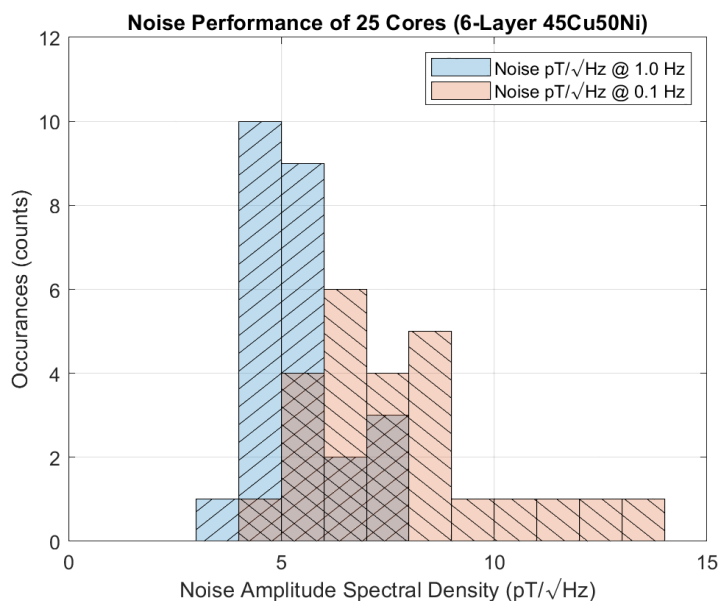
355 Fig. 9. 1.0Hz and 0.10Hz noise PSDs probability density plot for twenty-five 6-layer 45Cu50Ni racetrack sensor cores. Cross-hatched columns indicate sensor cores for both test frequencies.
