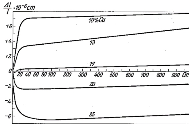
845 Fig. A17. Magnetostriction \Delta l/l as function of the applied field strength for 70% Ni, for various Cu-contents; 1100C-handling.
