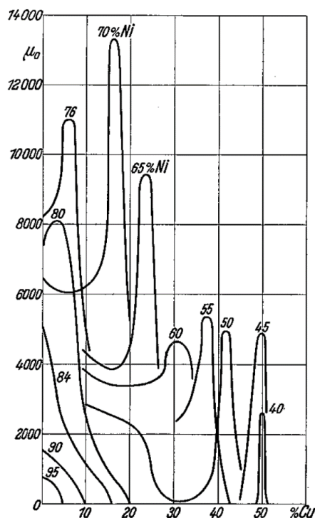
750 Fig. A4. Initial permeability \mu_0 as function of Cu-content; sections for various Ni-contents; Permalloy-handling.
