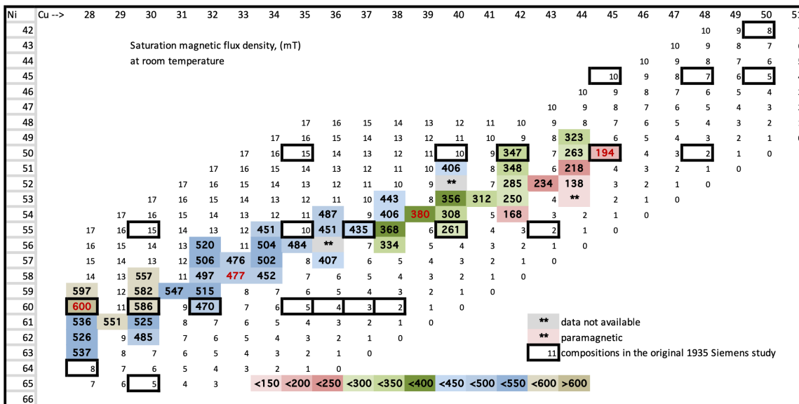
305 Fig. 4. Saturation induction, B_s , in mT. Highest values are presented in blues, to the left, and lowest values are presented in reds, to the right.
