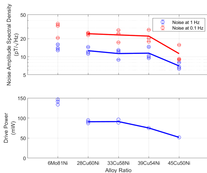
350 Fig. 8. Fluxgate noise PSD and power consumption for five alloys.
