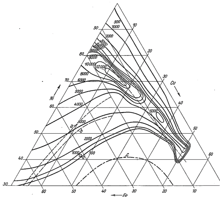
755 Fig. A6: Lines of constant initial permeability (-) in the FeNiCu system; Permalloy handling; Boundaries of phase separation region from other authors (a,b,c,d); Line of constant Ni:Fe ratio (---).
