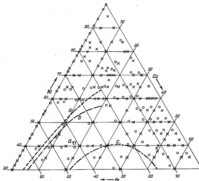
610 Fig. A1. Locations of alloys investigated in the FeNiCu-diagram in weight-percent (x) and in atomic-percent (o). Locations of phase separation region boundaries (a, b, c, d) taken from other authors.
