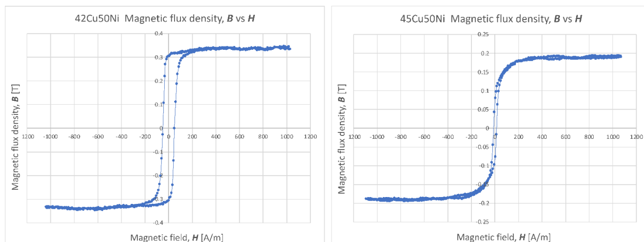
400 Fig. 10. Saturation B/H curves for alloys 42Cu50Ni and 45Cu50Ni.
