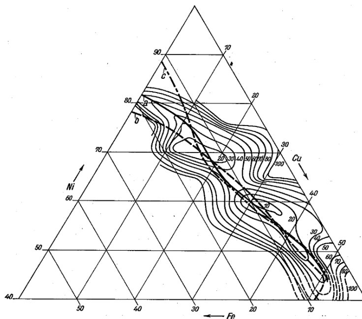
875 Fig. A19. Lines of constant field strength for saturation magnetostriction; Line of magnetostriction null (curve a); Lines of highest initial permeability for 1100C-handling (curve c) and for Permalloy-handling (curve b).
