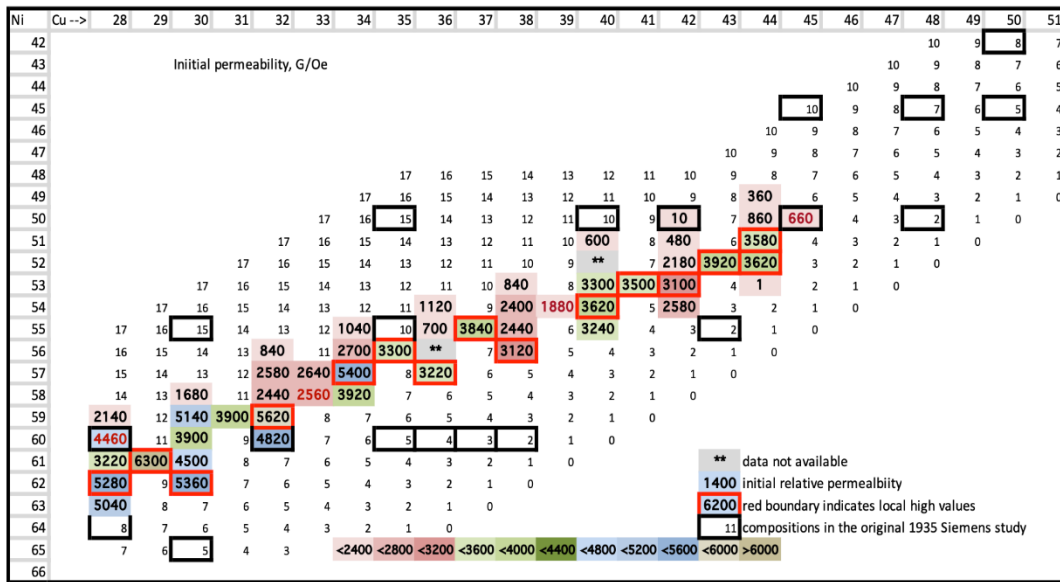
Fig. 6. Initial permeabilities. Highest permeabilities are colour-coded as blues and browns. Fifteen cells have been outlined in red with which we are indicating local high values for initial permeabilities.
