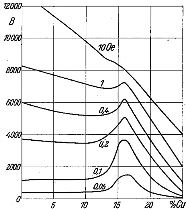
Fig. A2. Induction B as function of Cu-content for various field strengths; section for 70% Ni; Permalloy-handing.
