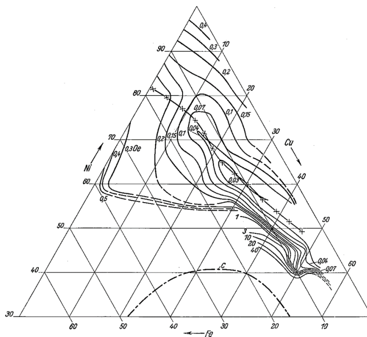
775 Fig. A11. Lines of constant coercivity (-) and line of zero magnetostriction in the FeNiCu system (-x-x); 1100C-handling.
