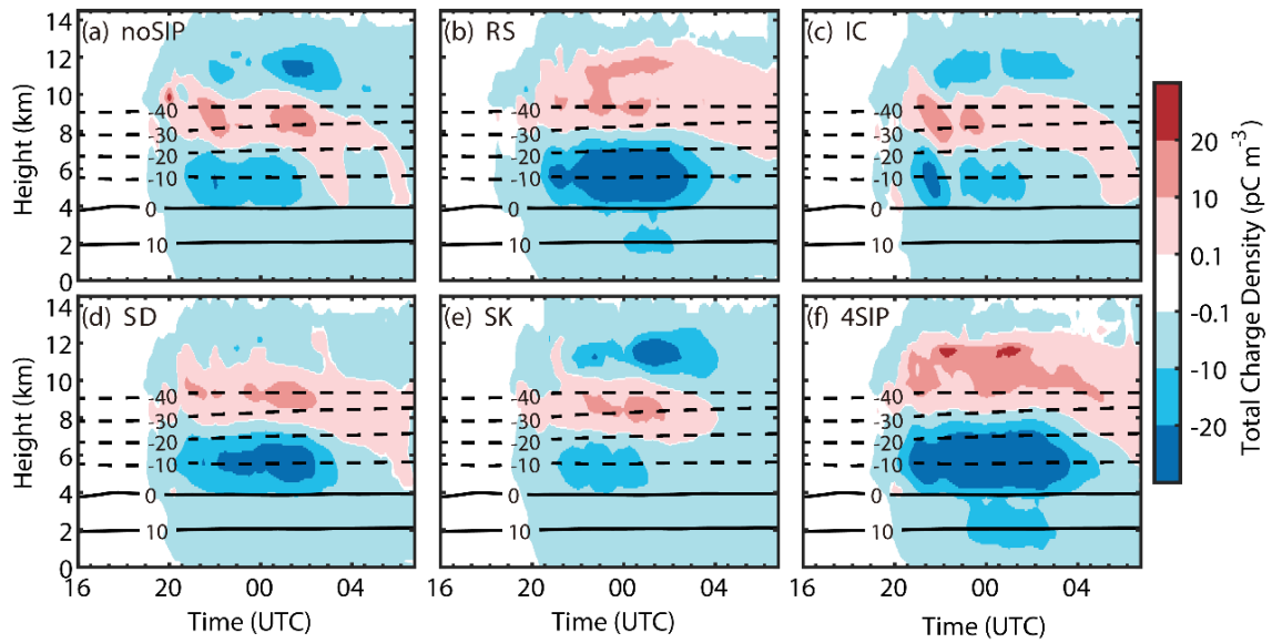
Figure 16: Time-height diagrams of the total charge density (colored) and temperature (contours) from the six numerical experiments. (a) experiment without SIP, (b) experiment with rime-splintering, (c) experiment with ice-ice collisional breakup, (d) experiment with shattering of freezing drops, (e) experiment with sublimational breakup of ice, and (f) experiment with four SIP processes.
