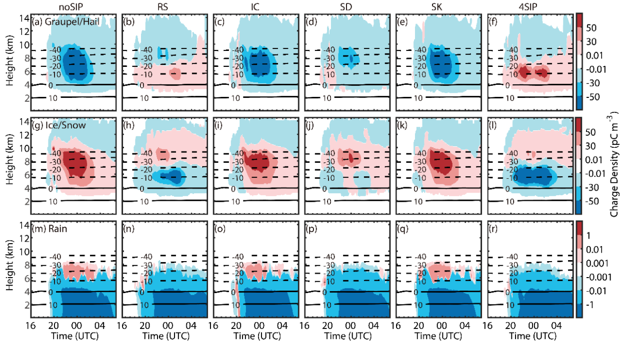
Figure 13: Time-height diagrams of the charge density carried by (a-f) graupel/hail, (g-l) ice/snow, and (m-r) rain from the six simulations. (a, g, m) experiment without SIP, (b, h, n) experiment with rime-splintering, (c, i, o) experiment with ice-ice collisional breakup, (d, j, p) experiment with shattering of freezing drops, (e, k, q) experiment with sublimational breakup of ice, and (f, l, r) experiment with four SIP processes. The black contours are the isotherms.
