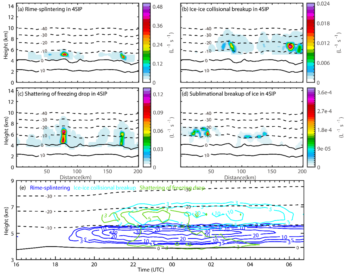
Figure 11: Cross-sections of the secondary ice production rates by different SIP processes resulting from the 4SIP experiment at 01:00 Nov. 28 th . (a) rime-splintering, (b) ice-ice collisional breakup, (c) shattering of freezing drops, (d) sublimational breakup of ice, and (e) the time-height diagram of the mean ice production rate by different SIP processes.
