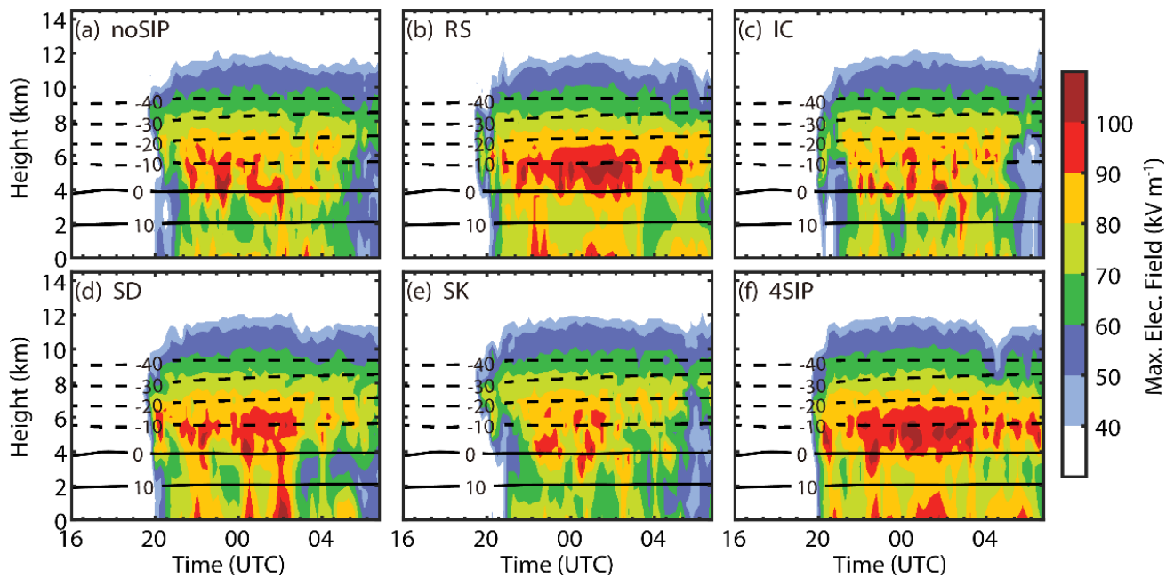
465 Figure 19: Time-height diagrams of the maximum vertical electric field from the six numerical experiments. (a) experiment without SIP, (b) experiment with rime-splintering, (c) experiment with ice-ice collisional breakup, (d) experiment with shattering of freezing drops, (e) experiment with sublimational breakup of ice, and (f) experiment with four SIP processes.
