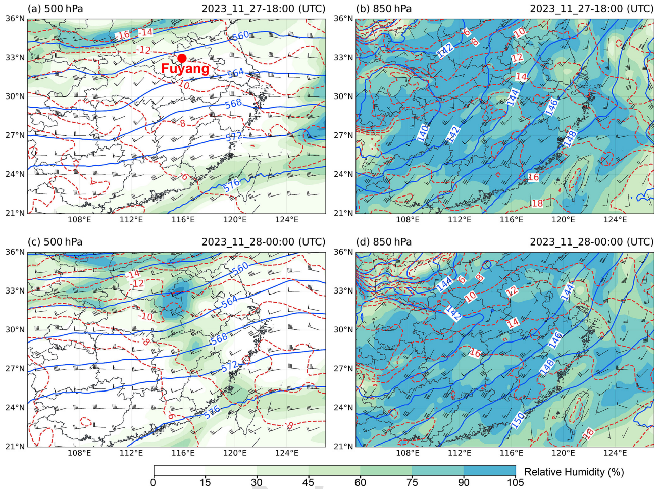
Figure 1. Synoptic conditions of the thunderstorm that occurred at (a,b) 18:00 UTC on 27 November and (c,d) 00:00 on 28 November. Panels (a) and (c) show the 500 mb geopotential height, isotherms, and wind barbs. (b,d) Same as (a) and (c) but for 850 mb. The red dot in (a) indicates the location of the sounding measurement that is shown in Fig. 2.
