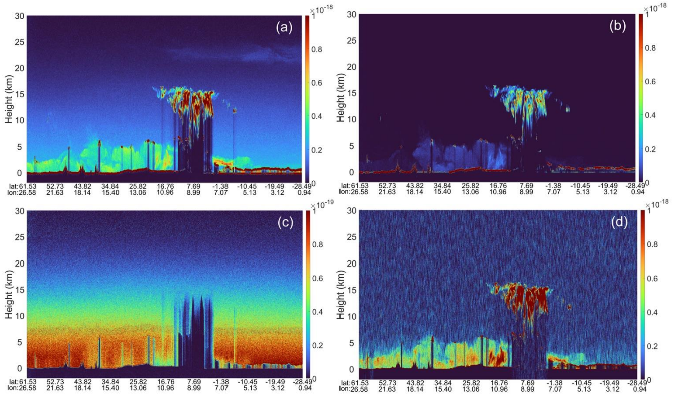
225 Figure 5: ACDL-A optical power signals in (a) 532 nm parallel polarized channel, (b) 532 nm perpendicular polarized channel, (c) 532 nm molecular channel and (d) 1064 nm channel on 00:45:23 UTC to 01:10:22 UTC on June 27, 2022.
