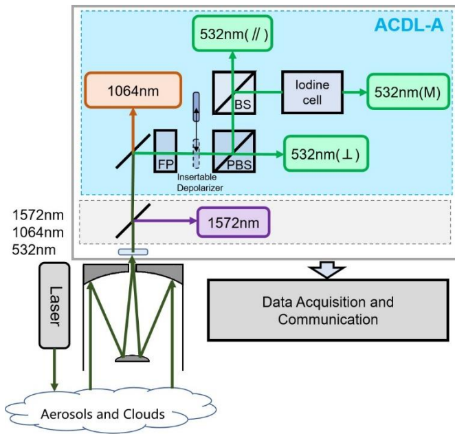
115 Figure 1: Schematic diagram of ACDL-A.
