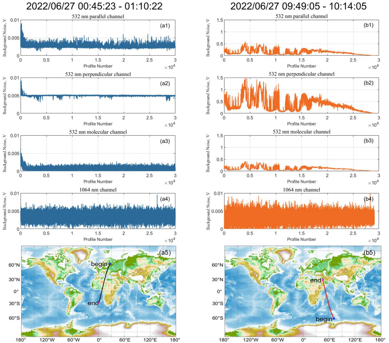
200 Figure 4: The background signal value subtracted from each echo signal in nighttime (blue dash on the left) or daytime (orange dash on the right) segment of data, both on June 27, 2022. Corresponding to each channel in order from top to bottom, (a1, b1) parallel-polarized channel at 532 nm, (a2, b2) cross-polarized channel at 532 nm, (a3, b3) molecular channel at 532 nm, (a4, b4) 1064 nm channel, and (a5, b5) satellite orbit.
