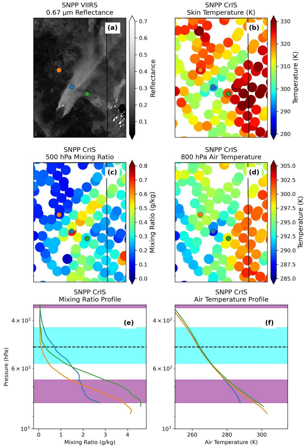
345 Figure 4: Suomi-NPP VIIRS 0.67 micron visible reflectance (a) , CrIS surface skin temperature (b), CrIS 500 hPa mixing ratio (c), and CrIS 800 mb air temperature (d), as well as profiles of CrIS mixing ratio (e) and temperature (f) from one location inside the smoke plume (blue) and two locations outside of the plume (orange and green). The cyan shading in panels e and f denotes where the mixing ratio at the blue point is greater than at the orange and green points by more than 0.1 g/kg, while the purple shading denotes regions in which the air temperature at the blue point is less than at the orange and green points by more than 0.5 K.
