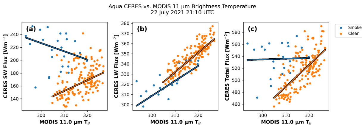
540 Figure 8: Scatter plots of CERES SW flux (a), LW flux (b), and total flux (SW + LW, c) with MODIS 11 \mu\text{m} brightness temperature within the plume (blue) and outside the plume (orange) for the MODIS and CERES overpasses on 22 July 2021 at 21:10 UTC shown in Fig. 1.
