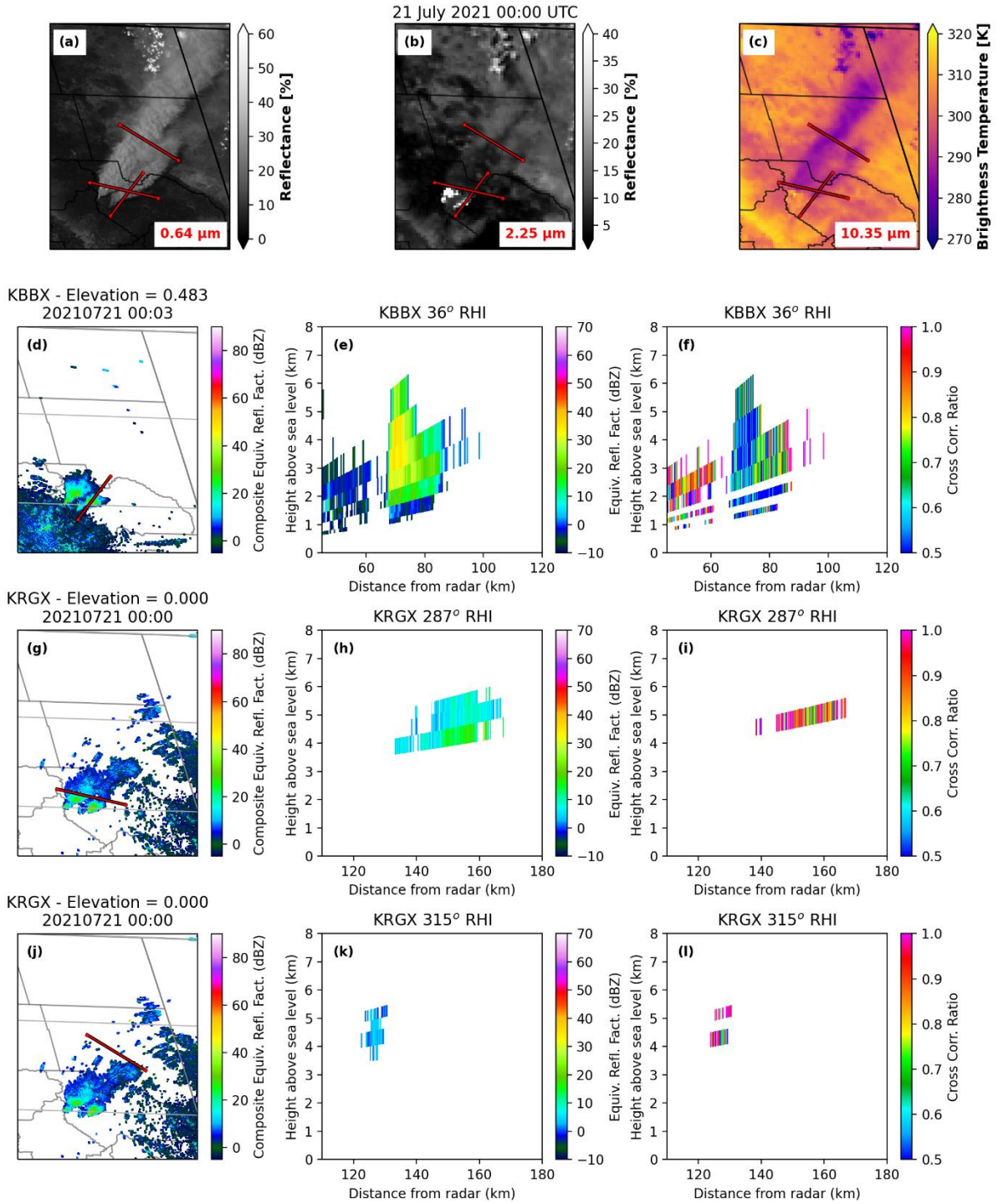
Figure 3. Comparison of GOES-17 and NEXRAD radar observations derived from the Beale AFB radar (KBBX, southwest of figure) and Reno, NV NWS radar (KRGX, southeast of figure) at 00:00 UTC 21 July 2021. First row: GOES-17 visible reflectance (a), shortwave IR reflectance (b), and thermal IR brightness temperature (c), with radar cross section locations added as red lines along azimuths from KBBX and KRGX. Second row: KBBX plan position indicator (PPI) of composite reflectivity (d), and range-height indicator (RHI) of reflectivity (e) and correlation coefficient (f). Third row: as in the second row, but for KRGX. Fourth row: as in the third row, but for a cross section much farther downwind of the fire.
