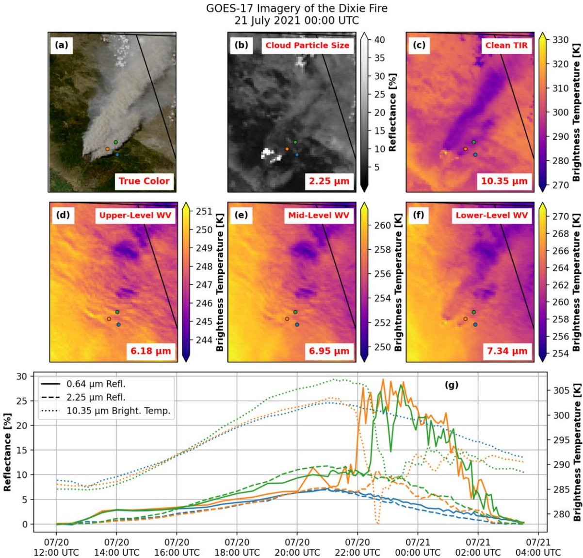
265 Figure 2: GOES-17 true color (a), shortwave infrared (2.25 μm, (b)), thermal infrared (10.35 μm, (c)), upper-level water vapor (6.18 μm, (d)), mid-level water vapor (6.95 μm, (e)), and low-level water vapor (7.34 μm, (f)) imagery of the Dixie Fire at 21 July 2021, 00:00 UTC. Third row: Time series of GOES-17 0.64 μm visible reflectance (solid), 2.25 μm shortwave infrared reflectance (dashed), and 10.35 μm brightness temperature (dotted) for points outside of the Dixie Fire smoke plume (blue) and inside the plume (orange and green) near the fire site.
