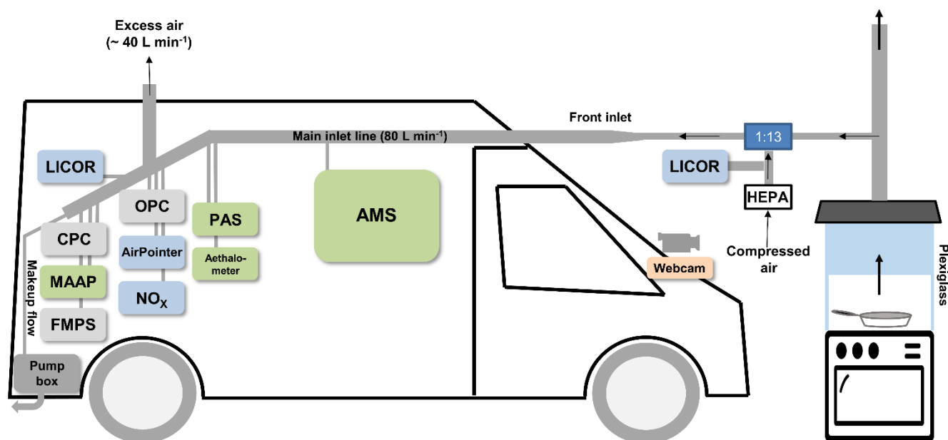
145 Figure 1: Scheme of the laboratory setup for the cooking experiments (MoLa scheme adapted from Drewnick et al., 2012). HEPA: high-efficiency particulate air filter. For details on the instrumentation, see Table S2.
