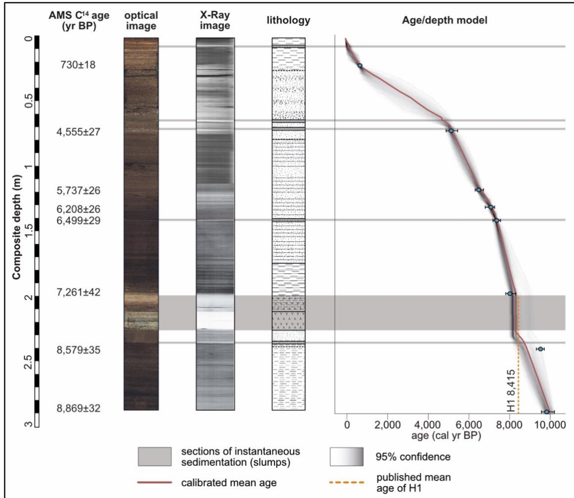
Figure 6 Radiocarbon ages, optical photography, radiography, lithology, and age-depth model of the composite sediment record for Laguna Meseta with the mean age for the Hudson H1 tephra (Stern et al., 2016). The age-depth model was developed
