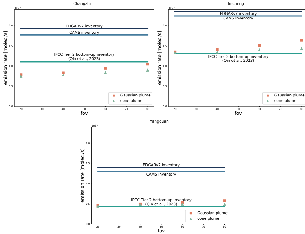
Figure 4: Estimates of emission rates in Changzhi, Jincheng and Yangquan regions with respect to different opening angles based on cone plume and Gaussian plume. The three different inventories are presented as well.
