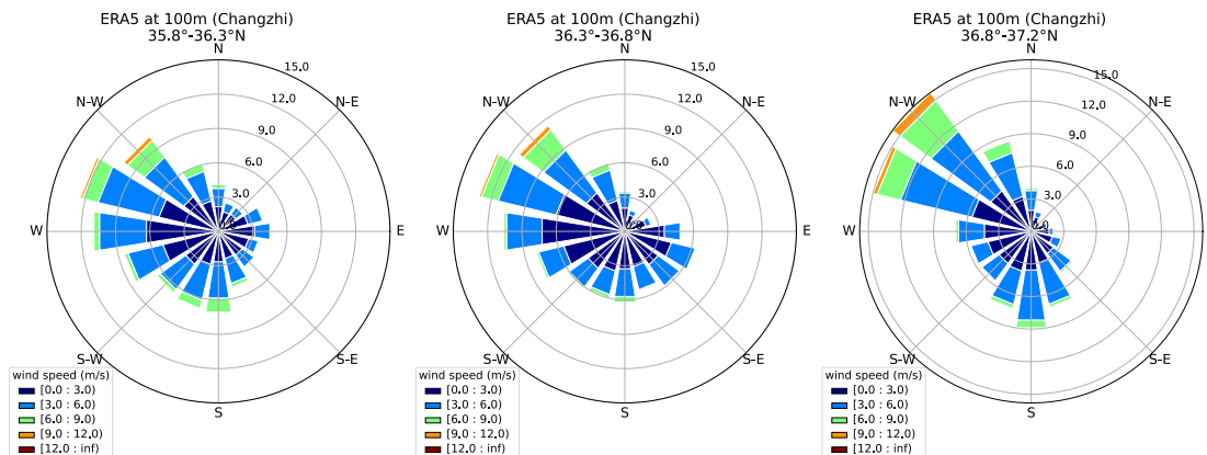
Figure 5: Wind roses plots for local daytime (08:00–18:00 UTC) from May 2018 to April 2023 for the ERA5 model wind for three subregions in Changzhi. The region range is given in the title of each subfigure.
