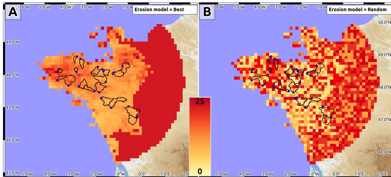
Figure 6. Best-fit and random denudation rate models. Denudation rates modeled on 10 x 10 km rectangular grid using the best-fit (A) and random (B) predictions models (cf. text). Sampled drainage basins and sampling locations are shown by the black outlines and blue dots.
