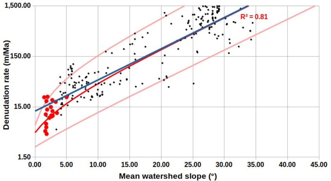
285 Figure 5: Model of denudation rates ( \text{m}\cdot\text{Ma}^{-1} ) vs. mean basin slopes ( ^{\circ} ). Red and black dots are the data for the Brittany area (this study) and from the Octopus database, respectively. The best-fit exponential function is in blue. The final, upper and lower models are in red. The uncertainties of individual values are not represented but are typically of the order of 10 %.
