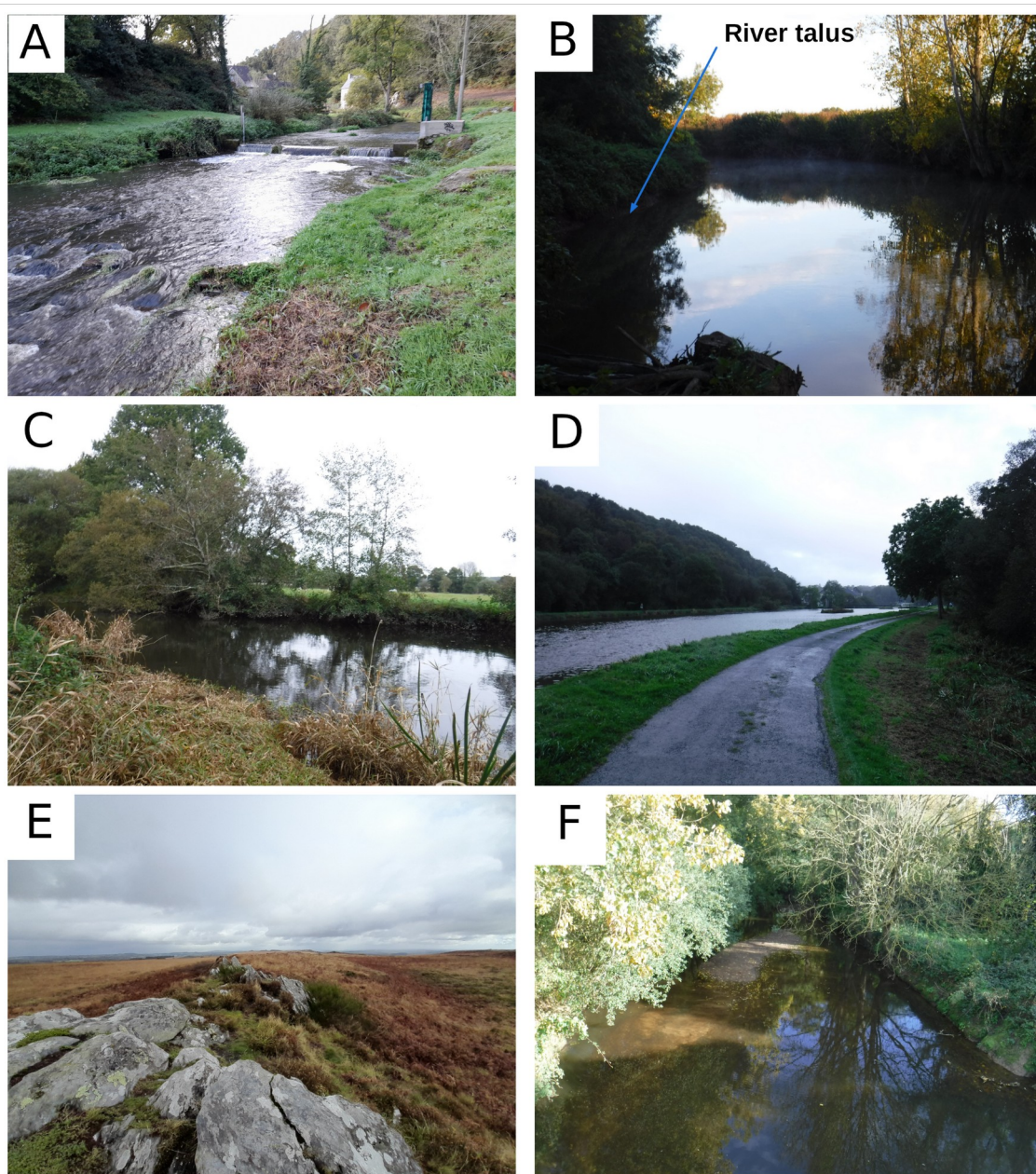
Figure 3: Photographs of common landscape and sampling site types. A- Guindy river sampling site. Example of minor anthropic disturbances. B- Meu river sampling site. Example of surrounding flat topography with local river talus and generalized tree-covered flanks. C- Claie river sampling site. Example of surrounding flat topography with local river talus and crop/bocage landscape. D- Example of localized relief, southern Brittany. E- Roc'h-Ruiz. Example of sampled outcrop in shrub-land areas. F- Arguenon sample site. Example of sampled central sand-bar. Photos: O. Malcles
