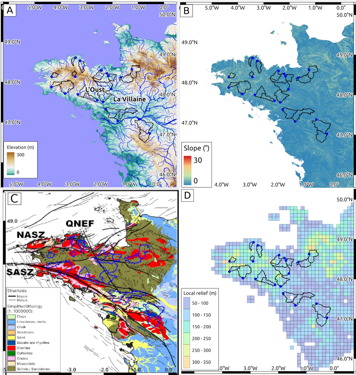
Figure 2: Morphology of the Armorican Massif and neighboring areas. Studied watersheds are delimited by the black polygons with the sampling sites identified by blue points. A: Elevation (DEM data from JAXA) and river networks (©IGN). The basins of Oust and Vilaine rivers are located. B: Slope. C: Simplified geology (BRGM, http://geoservices.brgm.fr/geologie ). Main tectonic structures
