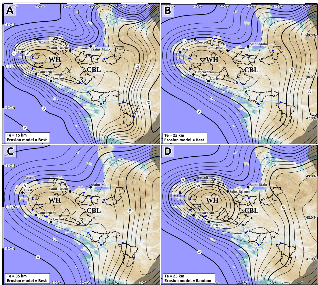
435 Figure 9. Predicted Late Pleistocene – Holocene uplift rates due to denudation rates. Isocontours of uplift rates in \text{m.Ma}^{-1} . A, B, C: Mean erosion model and three elastic plate thicknesses (15, 25, 35 km). D: Random erosion model and 25 km elastic plate thickness. The grey area on the east side shows where uplift rates are biased by model border effects and must not to be considered. CBL and WH stands for Central Brittany Lowland and Western Highland, respectively.
