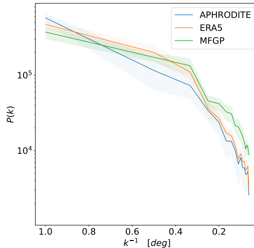
Figure 6. Power spectrum of the MFGP model, ERA5 and APHRODITE over a 2° by 2° area (31°-33°N, 77°-79°E) between 2000-2009. ERA5 and APHRODITE data are linearly interpolated to the same resolution as the MFGP output. The y-axis shows the power spectral density as a function of resolution, i.e. the inverse of the wavenumber k . The continuous lines show the average spectral densities and the shaded areas represent their standard deviation over time. All three datasets are z-scored prior to analysis.
