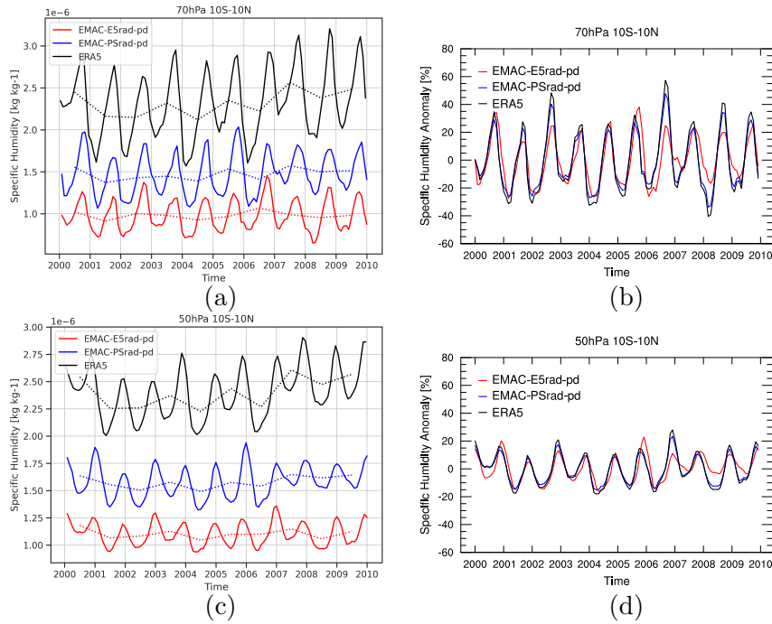
Figure 8. Tape recorder signal at 70 hPa (top row) and 50 hPa (bottom row) given by the specific humidity averaged over 10^{\circ} \text{ S} - 10^{\circ} \text{ N} . (a, c) Time series of specific humidity in 10^{-6} \text{ kg kg}^{-1} . (b, d) Relative anomaly (in percent) of the tape recorder signal, i.e. displayed is the relative anomaly with respect to the respective long-term mean (all months weighted equally).
