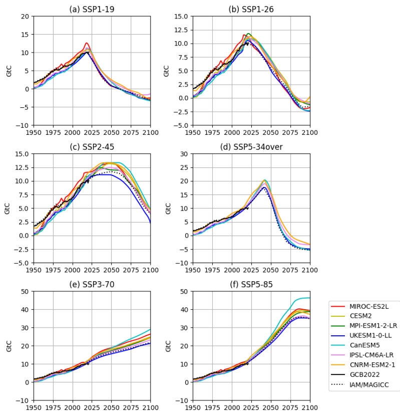
Figure 2: Compatible fossil emissions for a range of scenarios and Earth System Models in CMIP6, showing MAGICC calculated CO 2 emissions from IAM scenarios (Meinshausen et al., 2020) (dotted black), and the compatible fossil emissions in CMIP6 ScenarioMIP simulations (colored lines). Historical fossil emissions from the global carbon project (GCB2022 (Friedlingstein et al., 2022b)) are shown for context.
