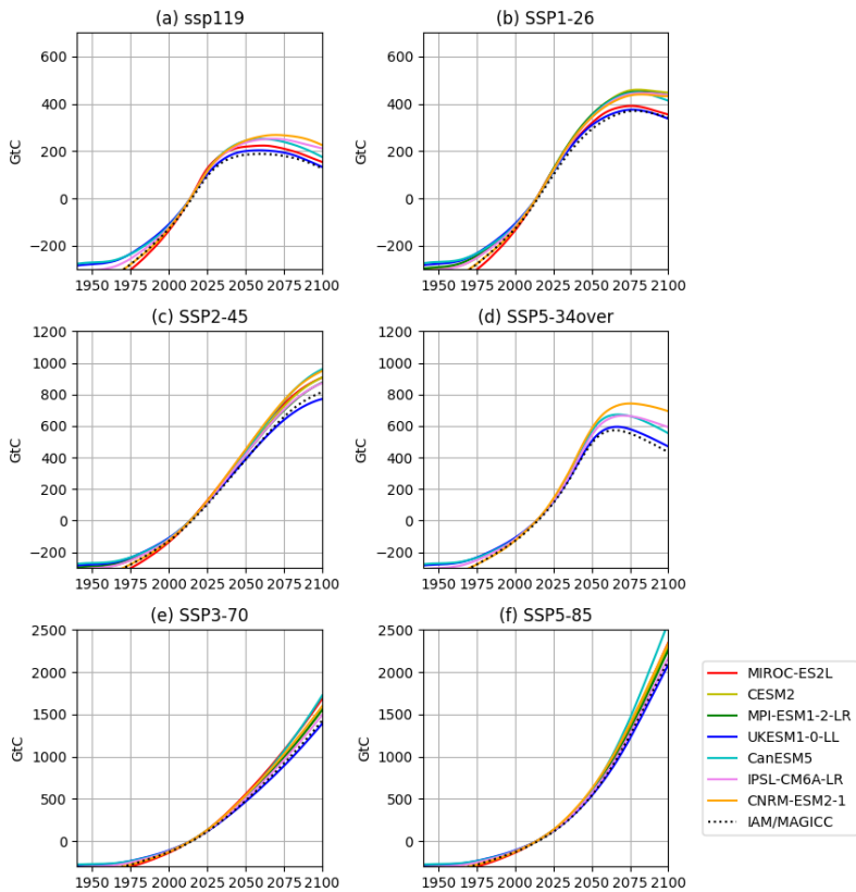
825 Figure A1: cumulative compatible fossil emissions (relative to 2014) for a range of scenarios and Earth System Models in CMIP6, showing MAGICCC calculated CO 2 emissions from IAM scenarios (Meinshausen et al., 2020) (dotted black), and the compatible fossil emissions in CMIP6 ScenarioMIP simulations (colored lines).
