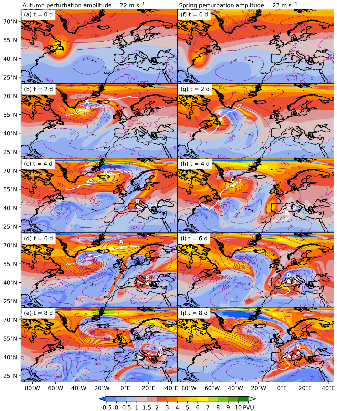
Figure 9. Same as Fig. 53f-j for initial conditions corresponding to the climatological mean in SON-autumn (a-e) and MAM-spring (f-j).
