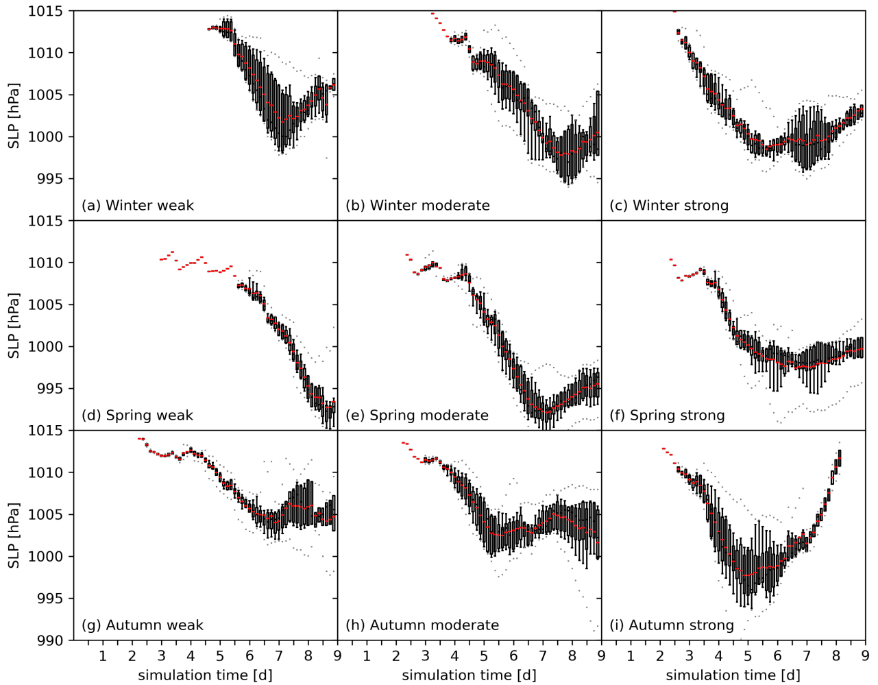
Figure 12. SLP evolution of Mediterranean cyclones in all (a-c) DJFwinter, (d-f) MAMspring, and (g-i) SON-autumn simulations, perturbed with a (a,d,g) weak upper-level PV anomaly, (b,e,h) moderate-intensity anomaly experiments, and (c,f,i) strong PV anomaly. Boxes mark the interquartile range, whiskers the 10th and 90th percentile and the red and black line the mean and median, respectively. The grey dots mark outliers of the 10th and 90th percentiles.
