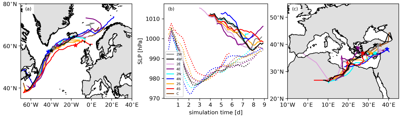
Figure 7. Cyclone tracks and characteristics for all non-SPPT-9 experiments in winter with a perturbation strength-amplitude of 22 \text{ m s}^{-1} . (a) North Atlantic cyclone tracks, maximum intensity highlighted with asterisks ; (b) SLP evolution of the North Atlantic (dotted) and Mediterranean (solid) cyclones. The legend indicates the horizontal location of the initial perturbation relative to the location of the maximum zonal jet: 2 and 4 mark displacements by 200 and 400 km, respectively and E, N, W, S indicate the direction of the shift. C labels the experiment with the perturbation located at the center of the jet; (c) Mediterranean cyclone tracks, asterisks again highlight maximum intensity.
