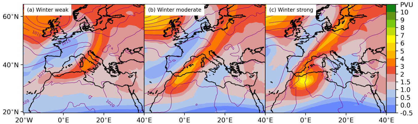
Figure 6. Composites after 4 d of 9 simulations each with slightly displaced initial perturbations (Table 1) for (a) “weak”, 11^{-1} , (b) “moderate”, 22^{-1} , and (c) “strong”, 34^{-1} perturbation amplitudes. Colors show PV at 300 hPa, and the purple contours SLP with 5 hPa intervals.
