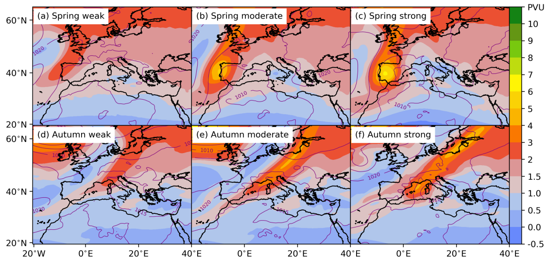
Figure 10. Same as Fig. 6 for initial conditions corresponding to the climatological mean in MAM-spring (a-c) and SON-autumn (d-f).
