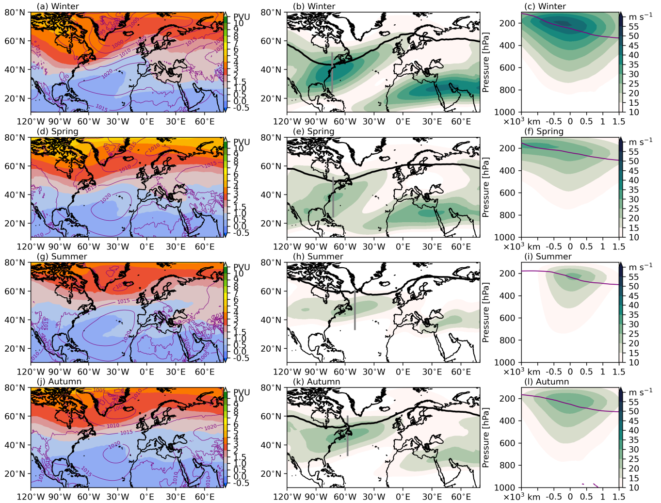
Figure 1. Overview of the climatological atmospheric conditions in DJF winter (a-c), MAM spring (d-f), JJA summer (g-i) and SON autumn (j-l). (a,d,g,j): PV at 300 hPa, the purple contours show SLP with intervals of 5 hPa; (b,e,h,k): Zonal wind at 300 hPa, the black line shows the 2 PVU contour; (c,f,i,l): Vertical cross section of zonal wind along grey line in (b,e,h,k) from south to north. The 2 PVU contour is shown in purple.
