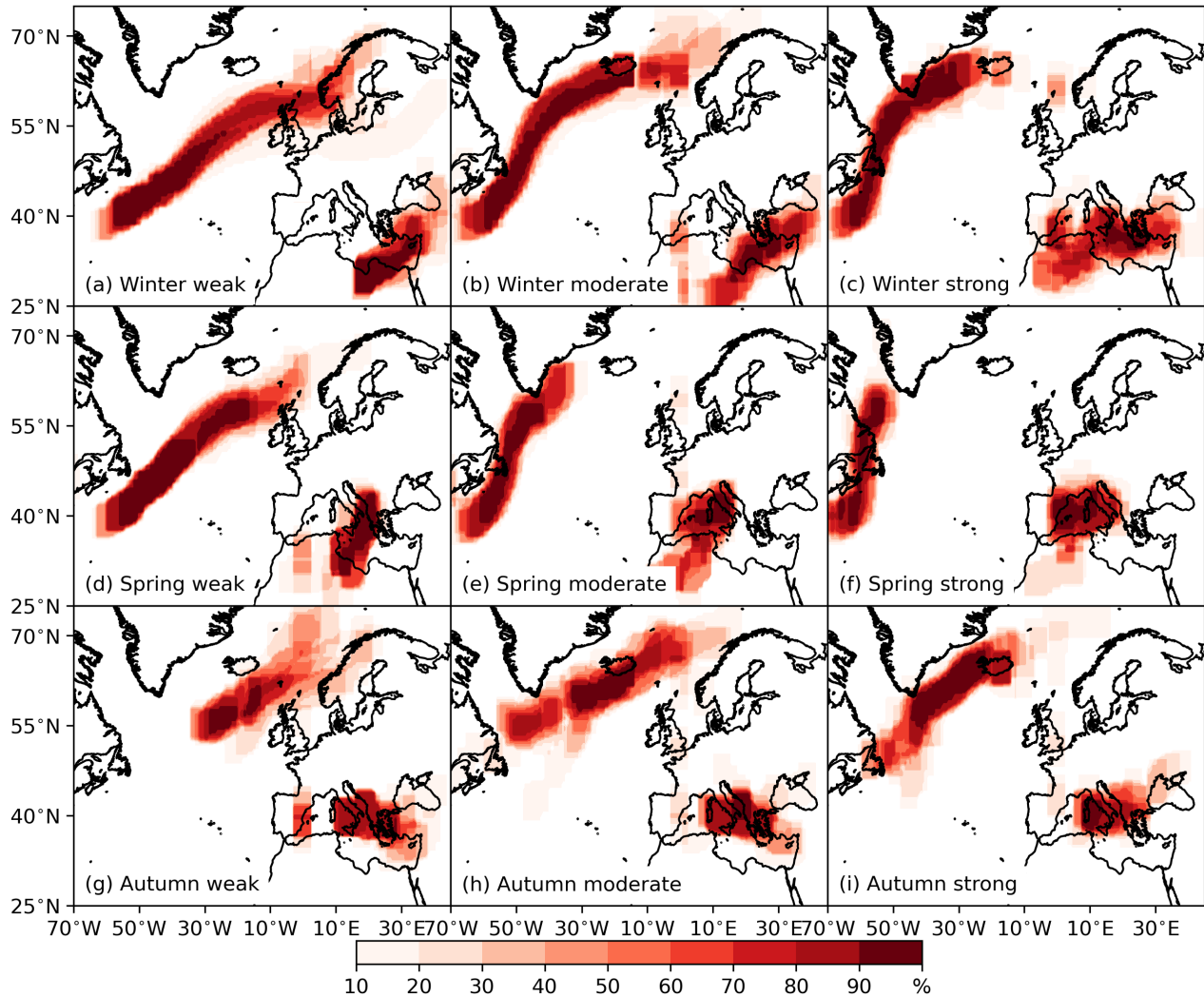
Figure 11. Cyclone track density for all DJF-winter (a-c), MAM-spring (d-f), SON-autumn (g-i) experiments, initialized with (a,d,g) weak, (b,e,h) moderate, and (c,f,i) strong initial perturbation experiments.
