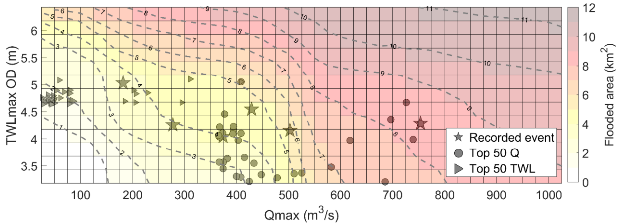
75 Figure S2: Results from Scenario-3: MAX SURGE, -3 HOUR LAG. Coloured surface represents modelled FloodArea exceeding the baseline areal threshold, from combinations of 520 Q and TWL (tide + min surge) scenarios with a -3 hour time lag (peak river is 3 hrs before peak HW). The 12 contours link common flooded area values. Shapes indicate the magnitude of river discharge and total water level (tide + surge) for recorded flood events (stars), top 50 most extreme TWL (triangles) and Q (circles).
