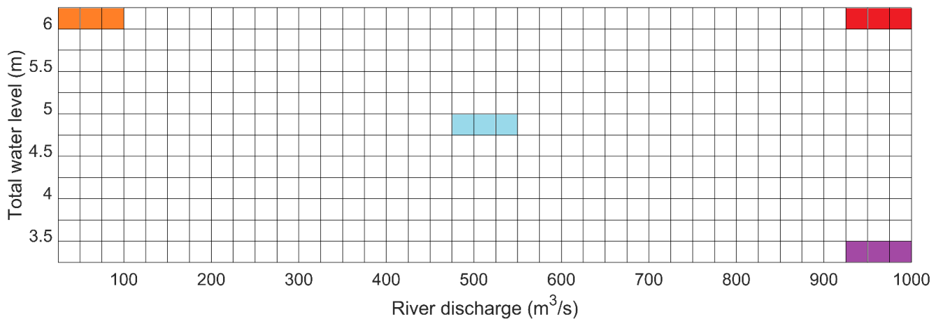
Figure S3: Four cases across the TWLmax: Q max parameter space: (a) TWL-dominant ( Q_{1-3}TWL_{13} ) - orange; (b) extreme compound ( Q_{38-40}TWL_{13} ) - red; (c) moderate compound ( Q_{19-20}TWL_7 ) - blue; and (d) river-dominant ( Q_{38-40}TWL_1 ) - purple.
