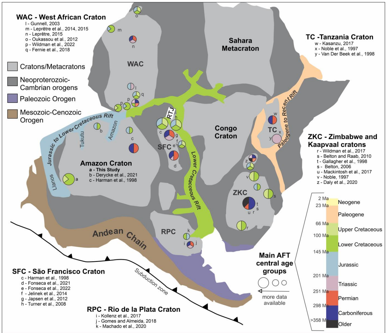
440 Figure 7: Apatite fission track (AFT) age compilation for cratonic segments that once were part of West Gondwana (ca. 180 Ma). Pie chart size indicates sample quantity, while colours represent main AFT central age groups in the region. RTJ: Recôncavo-Tucano-Jatobá aulacogen.
