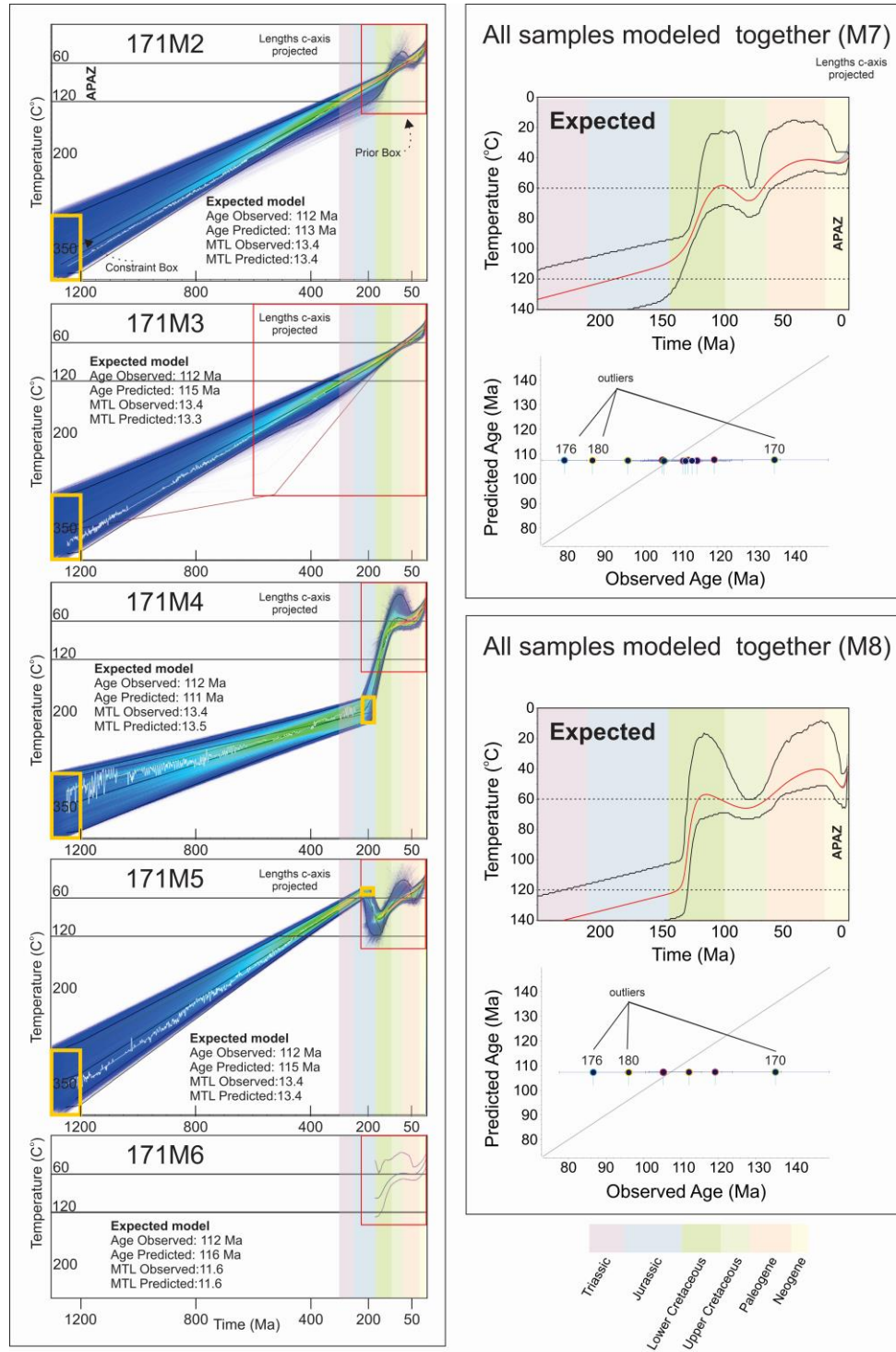
Figure 4: Thermal history modelling results (see section 5 for details).
