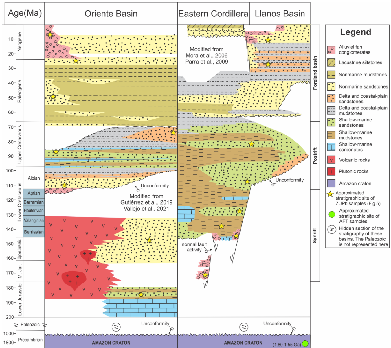
Figure 3: Simplified stratigraphic chart of the Llanos and Oriente basins providing the stratigraphic context for published detrital zircon U-Pb data that we depict in Fig. 6 (modified from Mora et al., 2006; Parra et al., 2009; Gutiérrez et al., 2019; Vallejo et al., 2021). The ages in blue refer to the time range of basement cooling constrained by our AFT data.
