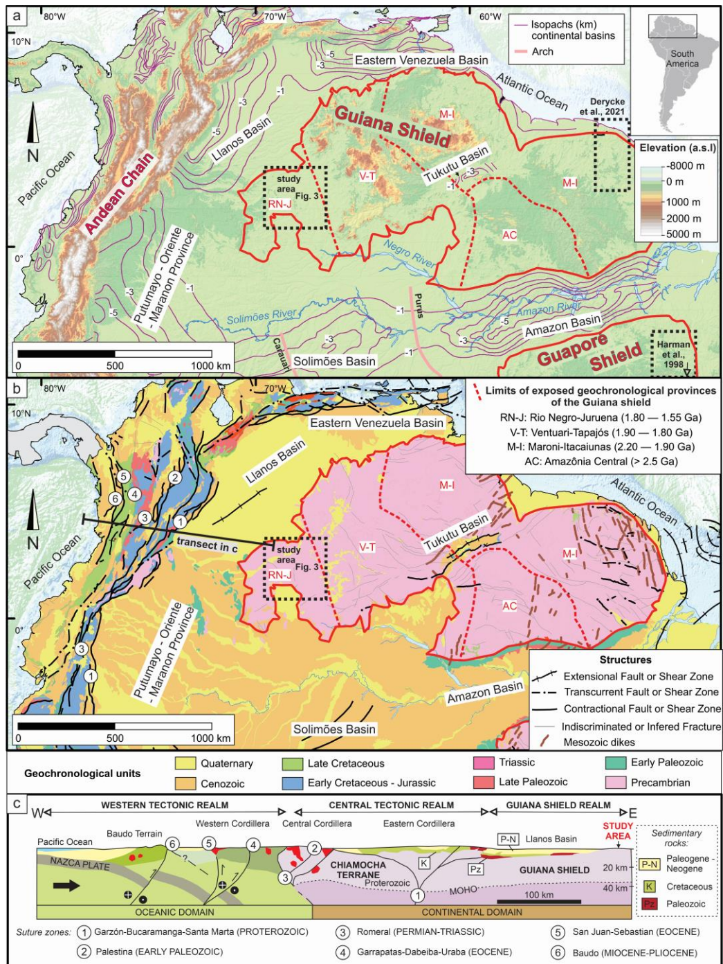
65 Figure 1: a) Digital elevation map (SRTM, USGS) of northern South America, with main tectonic structures, terranes and basins indicated (modified from Gómez et al., 2019). Our study area and the regions where previous low-temperature thermochronology date were obtained are delineated by the dashed boxes. b) Geochronological units with main tectonic structures, terranes and basins
