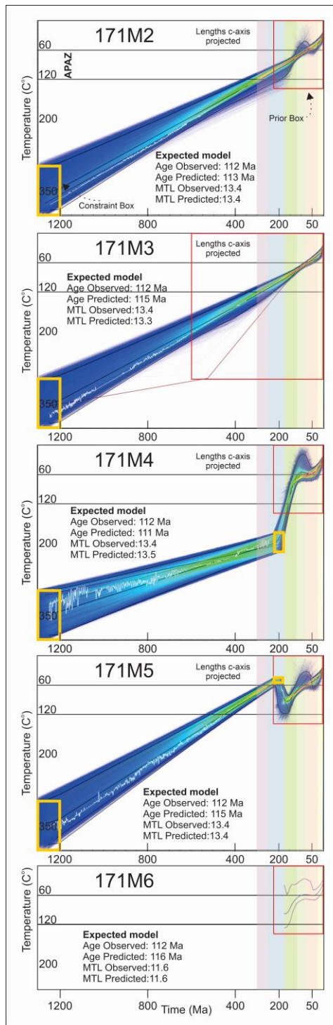
260 Figure 4: Thermal history modelling results (see section 5 for details).
