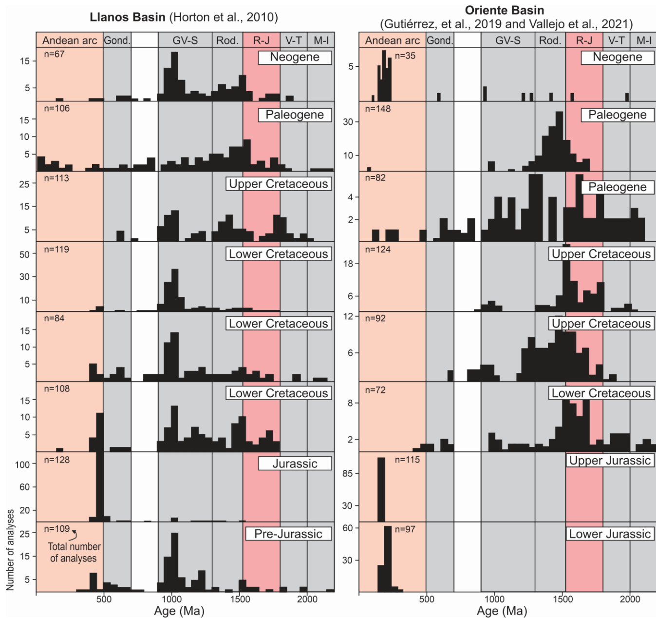
420 Figure 65: Age histograms depicting detrital zircon U-Pb ages for representative sedimentary rocks from the Llanos and Oriente basins. Stratigraphic location of samples shown in Fig. 3. Data from Horton et al., (2010), Gutiérrez et al., (2019) and Vallejo et al., (2021). M-I: Maroni-Itacaíñas belt; V-T: Ventuari-Tapajós belt; R-J: Río Negro-Juruena; Rod.: Rondonia belt; GV-S: Greenville-Sunsás; Gond.: Gondwanides orogeny.
