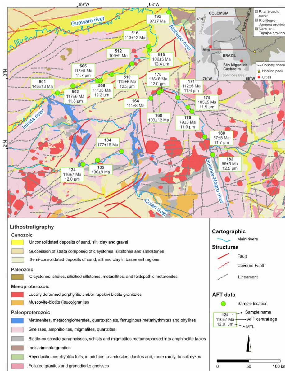
100 Figure 23: Geological map of the study area with sample site locations and apatite fission track (AFT) results (modified from Almeida and Mendes, 2021).
