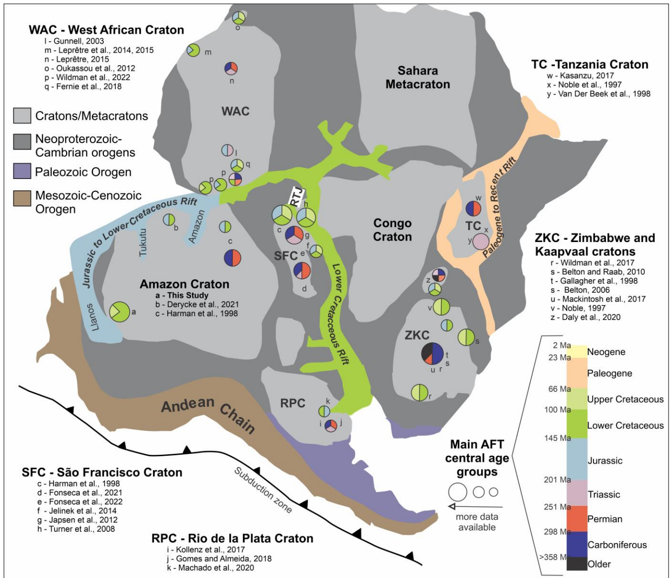
Figure 76: Apatite fission track (AFT) age compilation for cratonic segments that once were part of West Gondwana (ca. 180 Ma). Pie chart size indicates sample quantity, while colours represent main AFT central age groups in the region. RTJ: Recôncavo-Tucano-Jatobá aulacogen.
