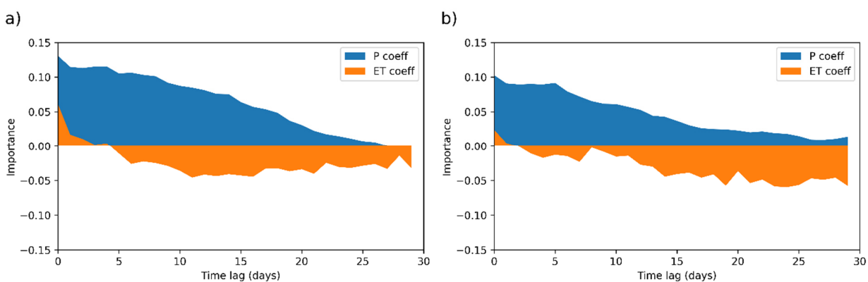
Figure 7: Model coefficients for precipitation and actual evapotranspiration: a) model 2004, with calibration period of 2004-2011, b) model 2015, with calibration period of 2015-2022.
