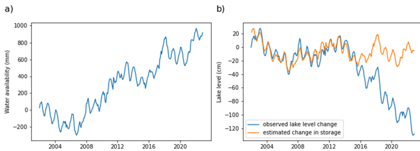
370 Figure 4: Water balance modeling: a) cumulative sum of water availability, b) observed and estimated lake levels.
