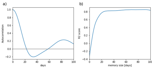
Figure 3: Lake response time analysis: a) autocorrelation of lake levels, b) fit quality of linear models of the weather forcing-lake level relations (eq. 6) using different system memory timeframes.
