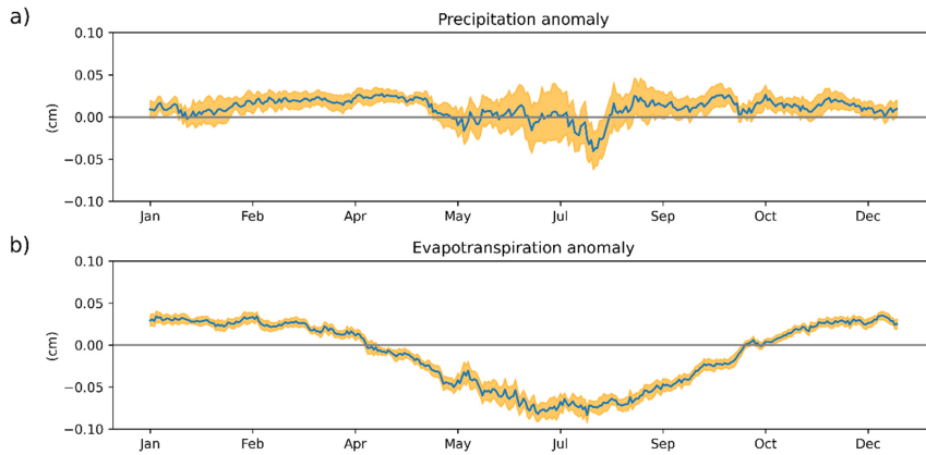
470 Figure 9: Yearly dynamics of the model discrepancies (model 2015-model 2004): a) median difference in precipitation response with confidence intervals, b) median difference in evapotranspiration response with confidence intervals.
