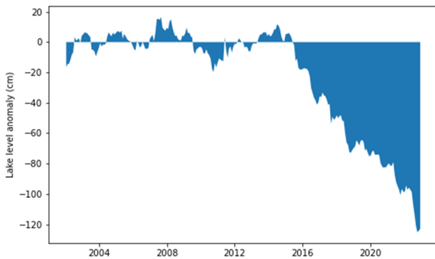
385 Figure 5. – Differences between the observations and the water balance model (non-climatic water balance anomaly). At positive values there is surplus water in the lake compared to the model, at negative values the lake shows a water deficit that is unaccounted for by the model.
