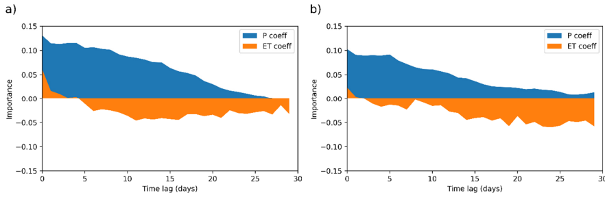
425 Figure 7: Model coefficients for precipitation and actual evapotranspiration: a) model 2004, with calibration period of 2004-2011, b) model 2015, with calibration period of 2015-2022.
