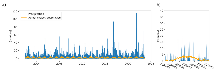
Figure 2: Weather forcing input data from the CER v2 dataset: a) investigation period, b) example year of 2009.
