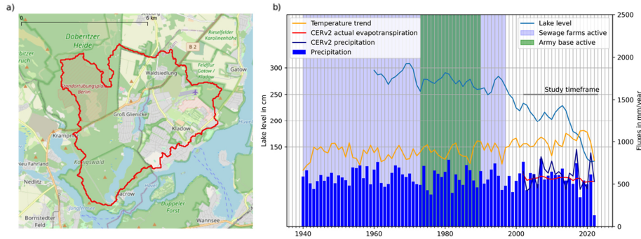
320 Figure 1: a) Catchment of the Groß Glienicke Lake (© OpenStreetMap contributors 2023. Distributed under the Open Data Commons Open Database License (ODbL) v1.0.), b) Overview of lake level changes of Groß Glienicke Lake together with concurrent timeseries of temperature and precipitation. Key events potentially impacting the lake system are shown as background colors.
