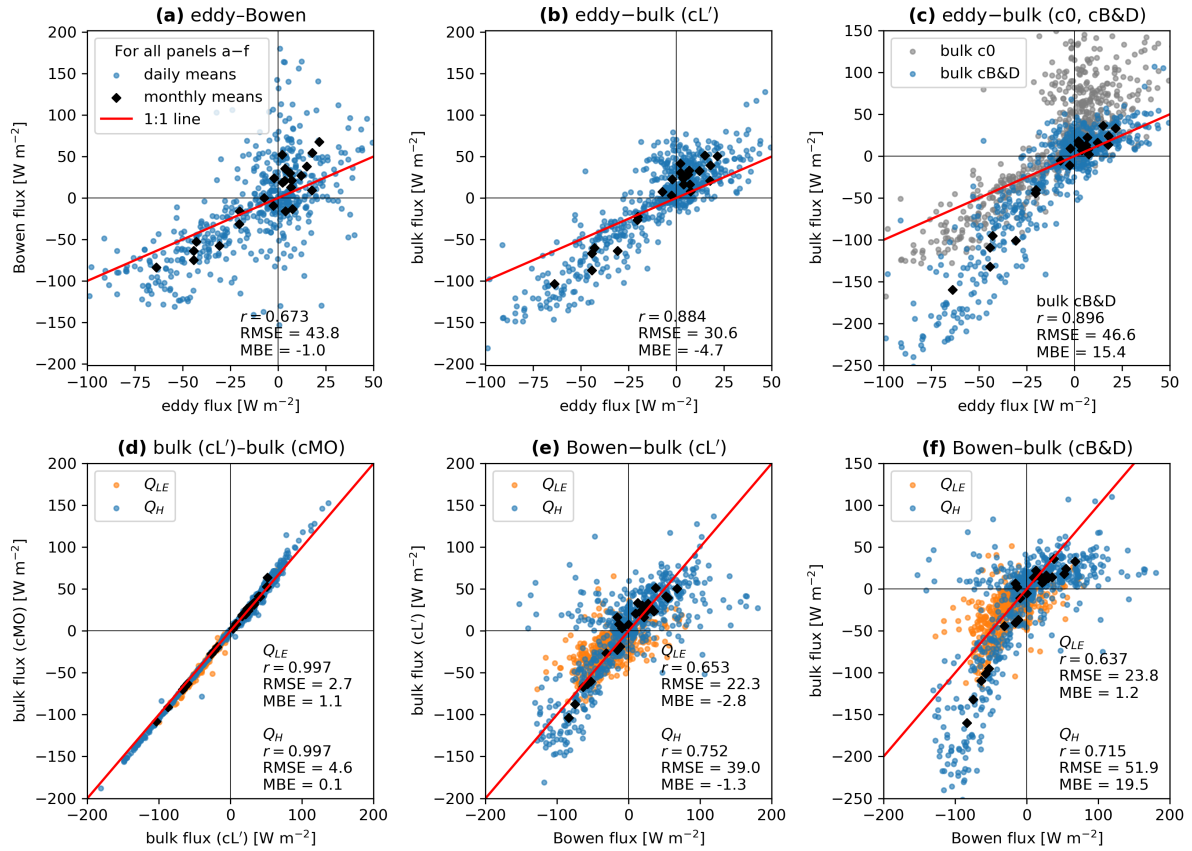
Figure 7. Comparison of turbulent flux estimates from different parameterisations (daily and monthly averages; cf. Fig. 6 for time series). Comparison metrics: root mean square error (RMSE [ \text{W m}^{-2} ]), mean bias error (MBE [ \text{W m}^{-2} ]) and Pearson correlation coefficient ( r [-]) on daily estimates.
