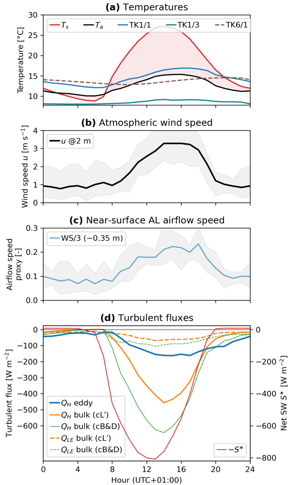
Figure 12. Hourly averages of (a) temperatures, (b) atmospheric wind speed, (c) near-surface AL airflow speed, (d) sensible turbulent fluxes and net short-wave radiation S^* during a summer fair-weather period (15–19 July 2022). The cavity air is stably stratified ( TK1/1 > TK1/3 ), but the air in the cavity roof is warmer and unstable compared with the outside air. During clear summer nights, the atmospheric air and the blocky surface cool down more strongly than the air in the near-surface coarse-blocky AL that receives heat from the blocks (air temperature TK1/1 approaches the rock temperature TK6/1 in the night). Conversely to the calculated bulk fluxes, the measured eddy flux decays slowly in the evening–midnight (18–24 h) and remains upwards (negative) despite the small temperature gradient in the early morning (3–7 h, (a)). The turbulent sensible flux draws heat from the near-surface AL that is nocturnally warmer than T_a and thus unstable. (b, c) Atmospheric wind and AL airflow speeds co-vary in phase (but at \sim 10\times smaller magnitudes), follow the net radiation with some delay and are closely related to the turbulent fluxes (d). The specific humidity shows small diurnal oscillations; the associated Q_{LE} vary less than Q_H in absolute terms.
