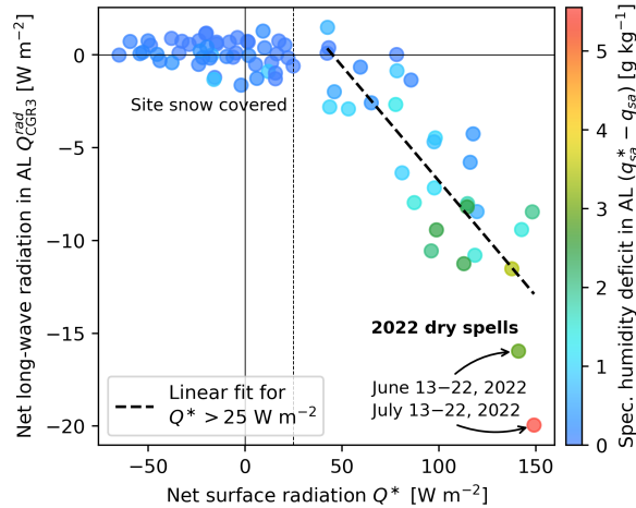
Figure 13. Relation between measured 10-day averaged surface net radiation Q^* and measured 10-day averaged in-cavity long-wave radiation Q_{\text{CGR3}}^{\text{rad}} (of the consecutive 10-day window) summarises the relation between Q^* , Q_H and Q_{LE} . The in-cavity net long-wave radiation Q_{\text{CGR3}}^{\text{rad}} represents the radiative downward heat transfer Q_r towards the ground ice table (note that upward heat transfer is primarily by convection and not represented by the radiation measurements; Q_{\text{CGR3}}^{\text{rad}} = Q_r \approx 0 \text{ W m}^{-2} during cooling episodes). Of the available net radiation Q^* , 90% is exported into the atmosphere by Q_H + Q_{LE} . Only 10% is transmitted deeper into the ground and available to warm the AL and to melt ground ice. Latent turbulent heat export is less efficient during dry spells, when the coarse-blocky AL dries out and evaporation becomes increasingly moisture-limited (outliers from June, July 2022). The relations between in-cavity long-wave radiation and air temperature, surface temperature ( \propto L^\dagger ), or Q_H are qualitatively similar.
