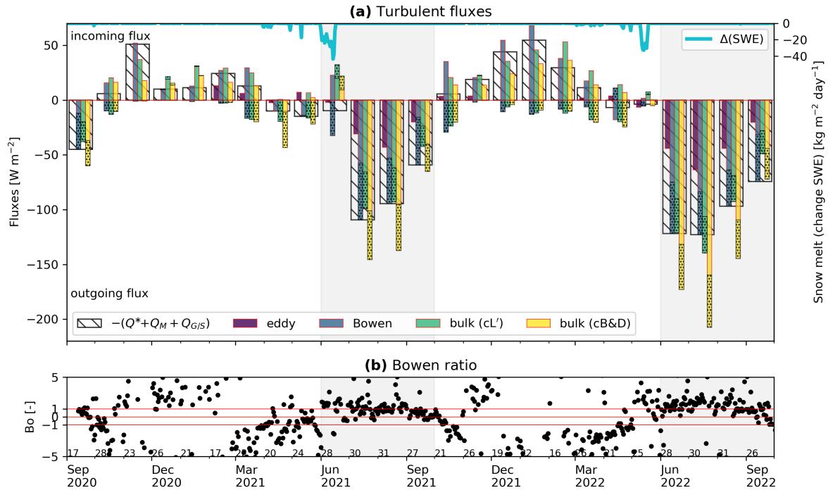
Figure 6. (a) Sensible and latent (dotted boxes) turbulent surface fluxes. Available energy from net radiation Q^* , snowmelt Q_M and ground heat flux Q_G (hatched boxes) is partitioned into sensible Q_H^{\text{Bo}} and latent Q_{LE}^{\text{Bo}} turbulent fluxes according to the Bowen ratio. The Bowen SEB is closed by design. Bulk fluxes differ according to the stability function and do not necessarily close the SEB. (b) Bowen ratio (Eq. 8). November–March: large scatter in winter because Q_{LE}^{\text{Bo}} is small and changes direction (unstable calculation). June/July–October: \text{Bo} \sim 0.5 – 2.5 , reflecting the wet-cool summer 2021 and the dry-hot summer 2022 (Fig. 3). Monthly average based on 16–31 valid values per month.
