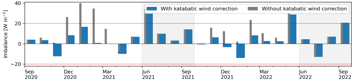
Figure 10. SEB imbalance (monthly averages). Turbulent fluxes calculated using modified Louis (1979) ( cL' ) bulk parametrisation. Correcting excessively high wind speed measured in the low-level katabatic jet at thick snow cover improves the SEB in the snow-rich winter 2020–2021 (katabatic wind correction; Sect. 6.2, Eq. 23).
