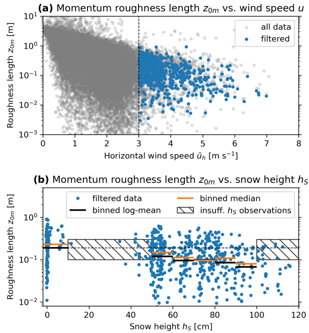
Figure 9. Calculated momentum roughness length z_{0m} vs. (a) horizontal wind speed \bar{u}_h and (b) snow height h_S . Of all values (grey dots), 2.1% met the quality criteria (blue dots). Momentum roughness length decreases from 0.19 to 0.07 m ( \times 10^{-0.43} ) with snow height increasing from 0 to 100 cm.
