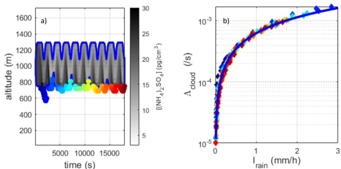
398 Figure 17. On the left: spatial-temporal distribution of the ammonium sulfate concentration in the contour of the cloud (criterion based on 399 the concentration of hydrometeors with a threshold set at 0.01 particle \cdot cm^{-3} ). On the right: correlation between the scavenging coefficient 400 and the precipitation intensity determined at the base of the cloud, (—) adjusted by a power law.
