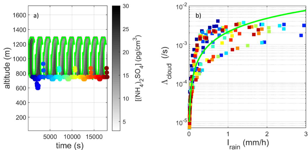
394 Figure 16. On the left: spatial-temporal distribution of the ammonium sulfate concentration in the cloud contour (—) criterion based on the 395 mass concentration of hydrometeors with a diameter greater than 64 \mu m with a threshold set at 0.01 g \cdot m^{-3} ). On the right: correlation 396 between the scavenging coefficient and the precipitation intensity determined at the base of the cloud, (—) adjusted by a power law.
