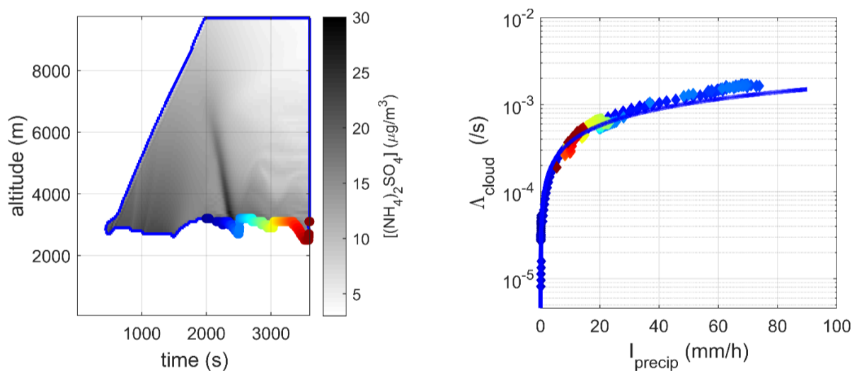
300 Figure 9. On the left: spatial-temporal distribution of the ammonium sulfate concentration in the cloud contour (— cloud contour for a mass 301 concentration of cloud hydrometeors greater than 0.001 \text{ g}\cdot\text{m}^{-3} ). On the right: correlation between the scavenging coefficient and the 302 precipitation intensity determined at the base of the cloud, (—) adjusted by a power law. Coloured points indicated where and when the 303 scavenging coefficient is calculated, colours are time increasing from the start (blue) to the end (red) of the rainfall.
