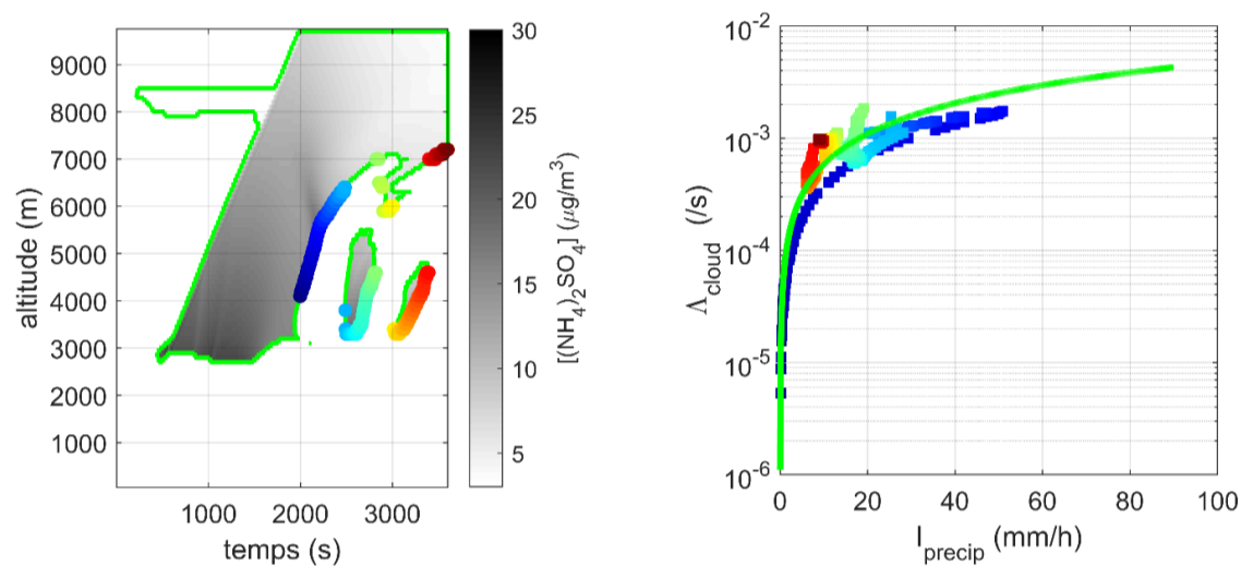
300 Figure 9. On the left: spatial-temporal distribution of the ammonium sulfate concentration in the cloud contour (— cloud contour for a mass 301 concentration of cloud hydrometeors greater than 0.001 \text{ g}\cdot\text{m}^{-3} ). On the right: correlation between the scavenging coefficient and the 302 precipitation intensity determined at the base of the cloud, (—) adjusted by a power law. Coloured points indicated where and when the 303 scavenging coefficient is calculated, colours are time increasing from the start (blue) to the end (red) of the rainfall.
