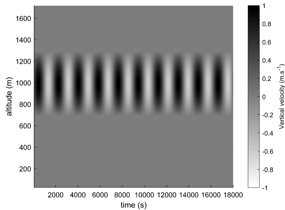
345 Figure 11. Spatial-temporal distribution of the vertical components of atmospheric flows (Zhang et al. , 2004)
