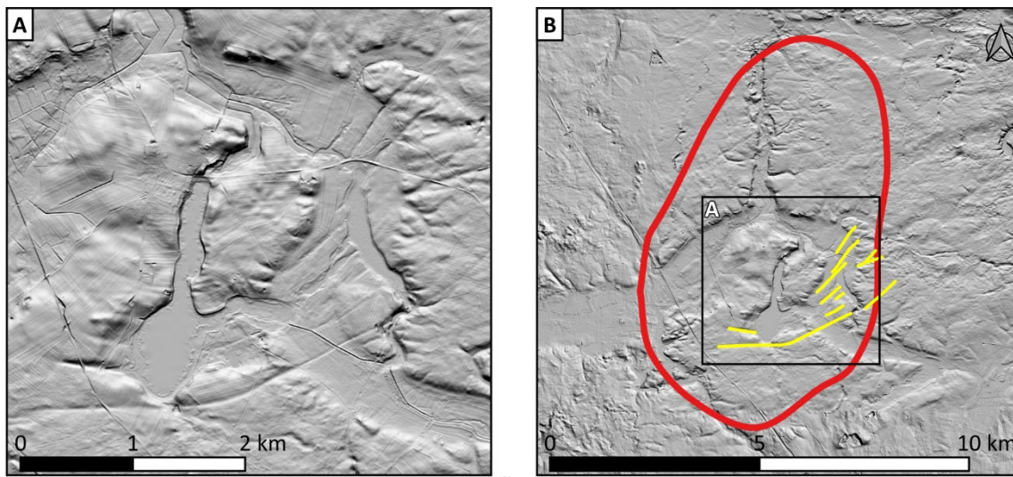
Figure 4: Hillshade maps of the Netzeband salt dome region. A: Detail view of the surface cracks found at the land surface atop the salt dome. B: Location of the surface cracks with relation to the outline of the salt structure. Hillshade with 5x vertical exaggeration based on 1 m LiDAR digital terrain model (GeoBasis-DE/LGB, 2020).
