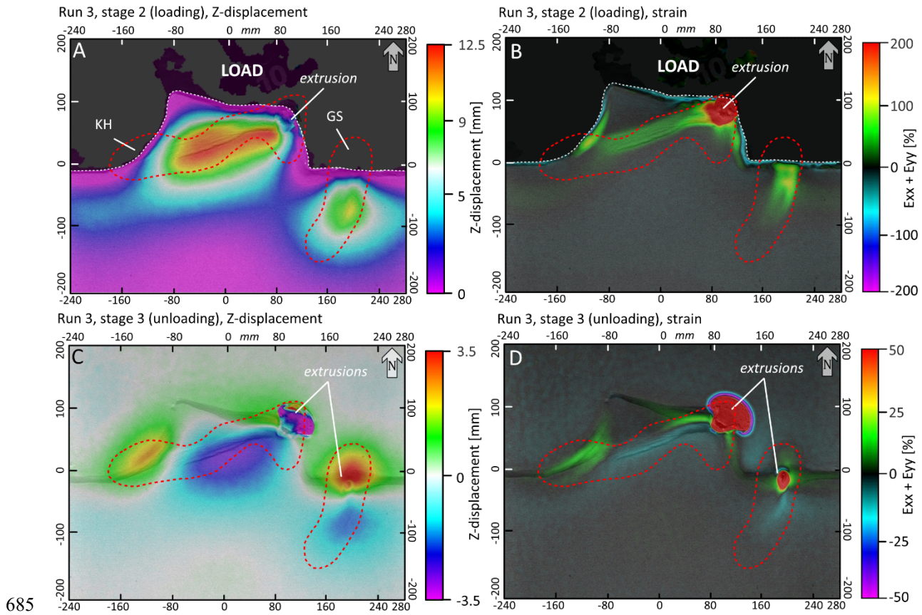
Figure 9: Summarizing DIC imagery of run 3. In stage 2, the load was applied to the north of the dotted white line. A: Z-map showing total vertical displacement in mm of stage 2. B: Strain [%] map of the total strain of stage 2. C: Z-map showing total vertical displacement in mm of stage 3. D: Strain [%] map of the total strain of stage 3. Red dashed outlines depict approximate position of salt structures.
