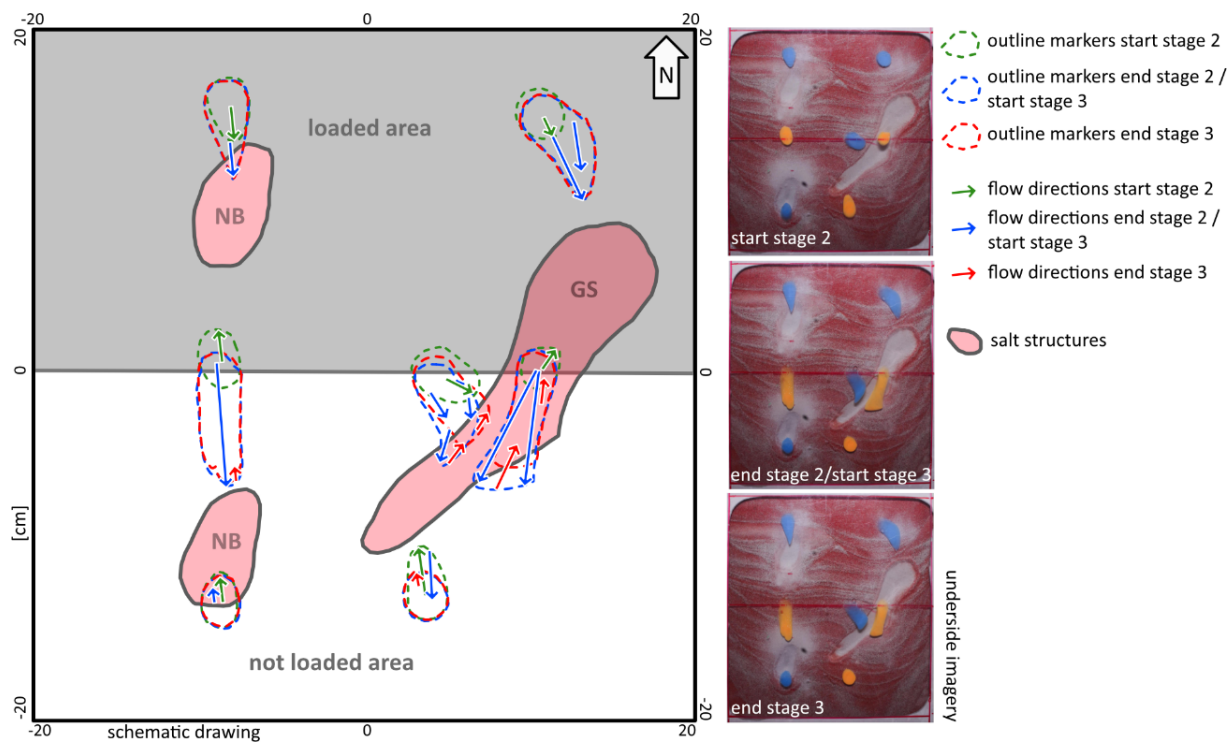
680 Figure 7: Schematic drawing of flow patterns during three stages, based on underside imagery of run 2.
