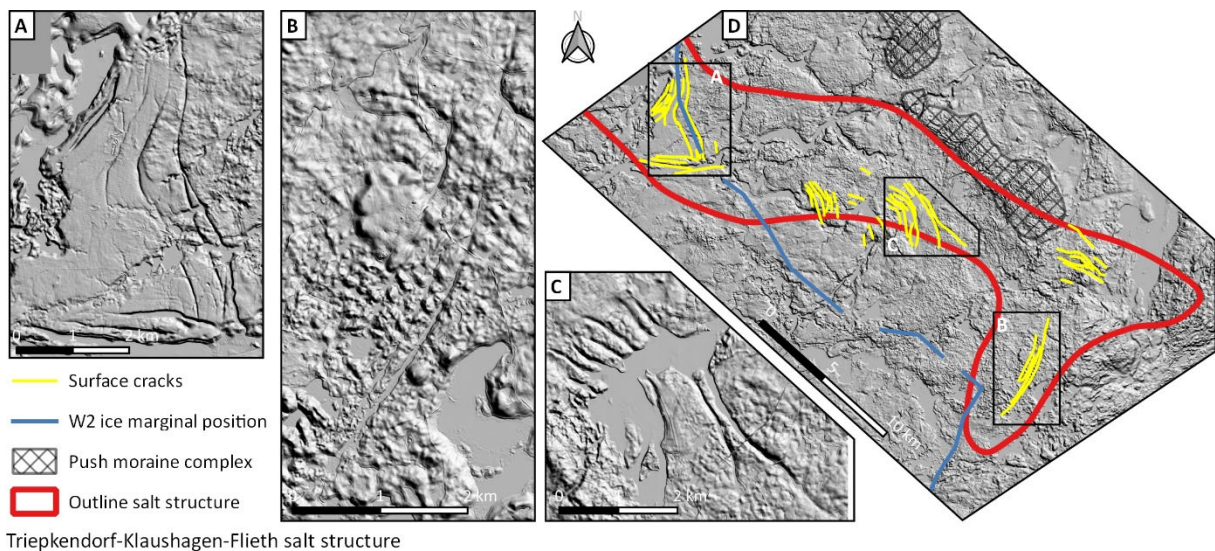
Figure 3: Hillshade maps of the Triepkendorf-Klaushagen-Flieth salt structure region. A: Detail view of the surface cracks found at the land surface atop the salt pillow in the Thomsdorf area. B: Detail view of the surface cracks found at the land surface atop the salt pillow in the Friedrichswalde area. C: Detail view of the surface cracks found at the land surface atop the salt pillow in the lake Kuhzer See area. D: Location of the surface cracks with relation to the outline of the salt structure. Hillshade with 5x vertical exaggeration based on 1 m LiDAR digital terrain model (GeoBasis-DE/LGB, 2020).
