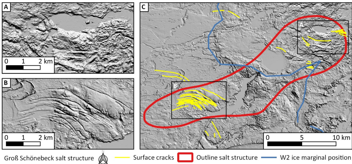
Figure 2: Hillshade maps of the Groß Schönebeck salt pillow region. A: Detail view of the surface cracks found at the land surface atop the salt pillow in the Altkünkendorf area. B: Detail view of the surface cracks found at the land surface atop the salt pillow in the Schorfheide area. C: Location of the surface cracks with relation to the outline of the buried salt structure. Hillshade with 5x vertical exaggeration based on 1 m LiDAR digital terrain model (GeoBasis-DE/LGB, 2020).
