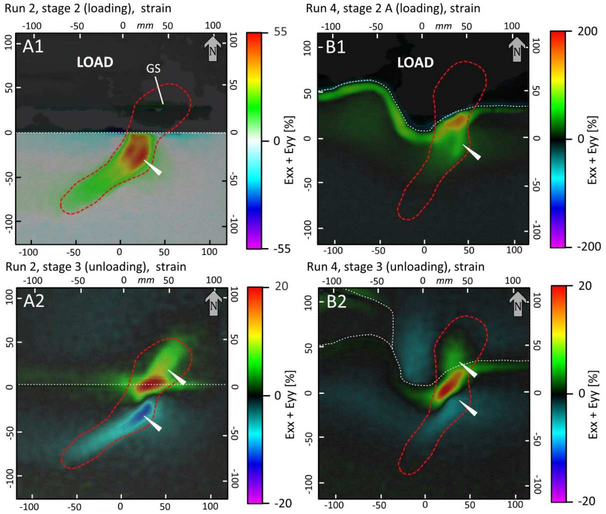
Figure 8: Comparison of strain patterns above GS pillow using different load geometries (white dashed line): Left column - straight load margin; right column: lobate load margin. Red dashed outlines depict approximate position of salt structures. White arrows indicate position of crestral graben structures.
