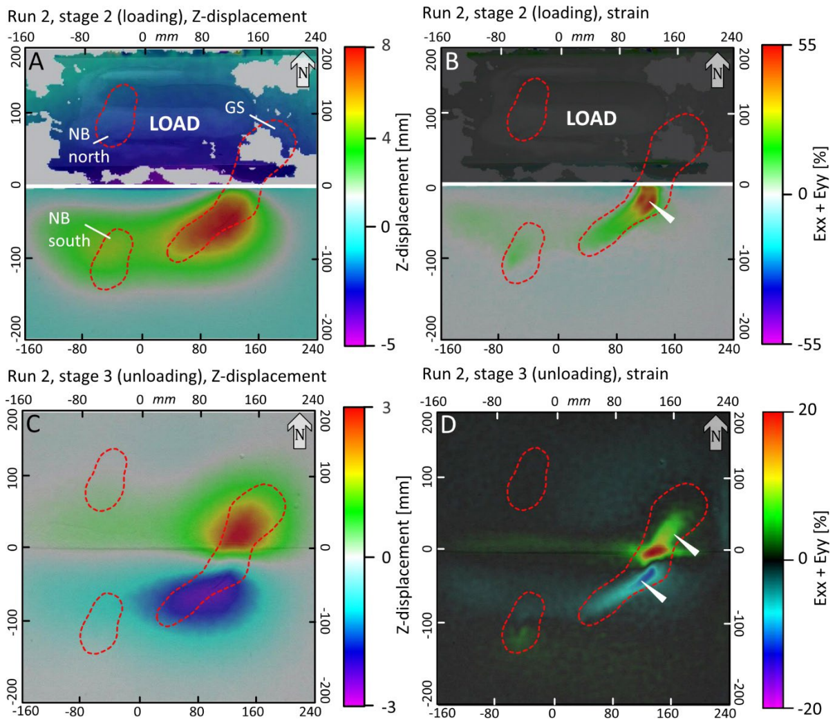
Figure 7: Summarizing DIC imagery of run 2. In stage 2, the load was applied to the north of the horizontal white line. A: Z-map showing total vertical displacement in mm of stage 2. The grey colors in the upper half of the figure are “no data” areas. B: Strain [%] map of the total strain of stage 2. C: Z-map showing total vertical displacement in mm of stage 3. D: Strain [%] map of the total strain of stage 3. Red dashed outlines depict approximate position of salt structures. White arrows indicate position of crestal graben structure.
