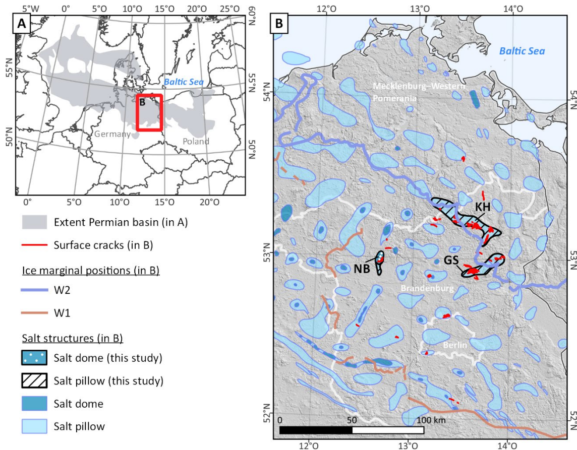
Figure 6: Overview map. Bright blue polygons: salt pillows; dark blue polygons: salt domes (InSpEE, 2015). Polygons with black outline: Salt structures investigated in this study (see Figures 2 – 5 for detail maps). GS – Groß Schönebeck study site; KH – Klaushagen study site; NB – Netzeband study site. Brown line: LLGM (W1) ice extent, blue line: gLGM (W2) ice extent (Lüthgens and Hardt, 2022; Lüthgens et al., 2020). White lines in B are German administrative borders plotted for orientation.
