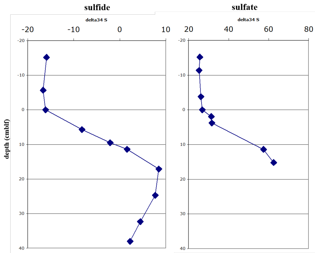
Figure S2 | \delta^{34}\text{S} profiles of sulfide and sulfate measured in Lake Cadagno bottom waters and surface sediments in 1991.
