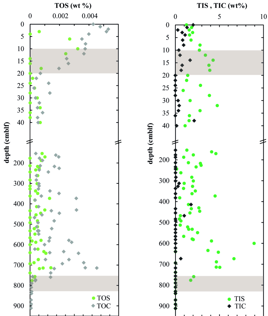
Figure S1 | TOC and TOS content (left) and TIC and TIS content (right) in the sediment column of Lake Cadagno. The shaded regions denote the upper and lower sulfate depletion zones. Note the break in the y-axis.
