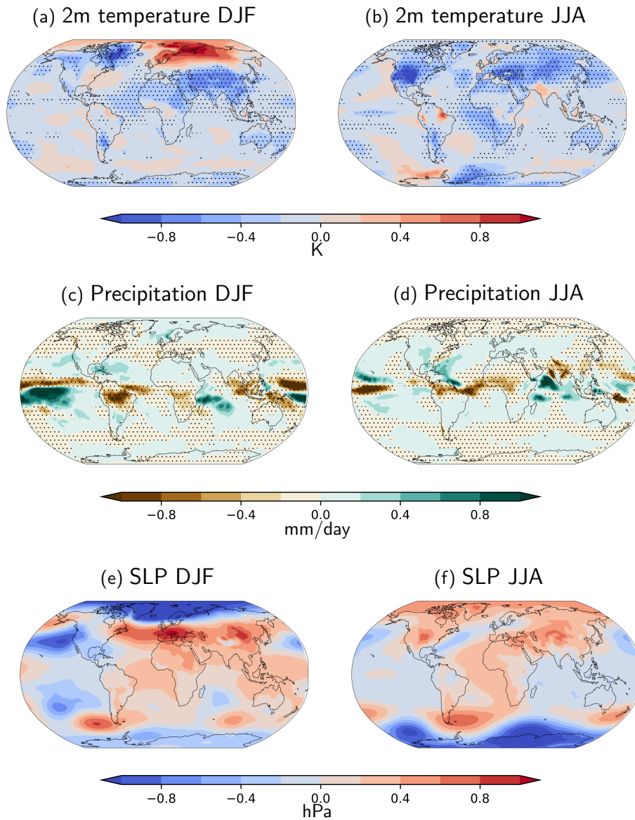
Figure 4. Response to volcanic forcing. Difference between the first winter (DJF, left column) and summer (JJA, right column) after an eruption for 2m temperature (top), precipitation (middle) and sea level pressure (bottom) and the same quantity averaged over the 5 previous summers/winters. The resulting response was then averaged over 15 major eruptions (same as in Fischer et al. (2007), table 1 therein.) and across all ensemble members. Only significant values are shown, i.e. grid points where the response is outside the 5 to 95 percentile range of 1000 surrogates with each surrogate being created by picking 15 random years and then computing the averaged difference between these 15 random years w.r.t. the 5 years before.
