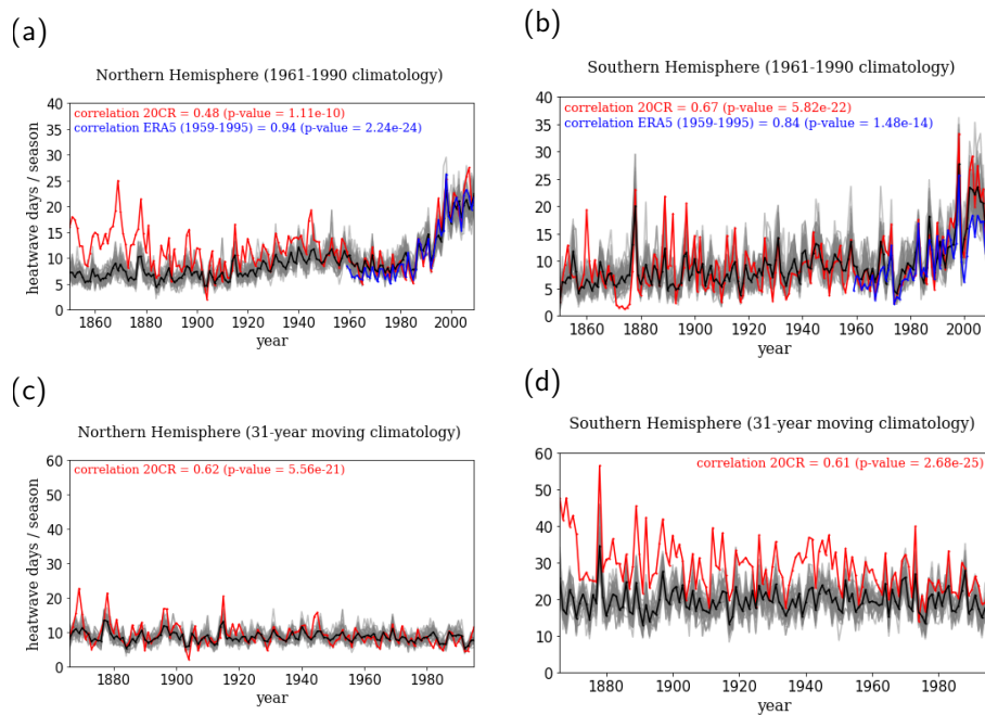
Figure 7. Ability of Mode-Sim to capture late 19 th and 20 th heat waves for (a) Northern hemisphere (10°N to 80°N) in boreal summer (May to September) and (b) Southern hemisphere (65°S-0°) in austral summer (November to March). Shown is the number of heatwave days per season defined as days when 2m temperature exceeds the 90 th percentile of the 1961 to 1990 reference period. Light colours show the individual Mode-Sim ensemble members, the black line the Mode-Sim ensemble mean, the blue line ERA5 and the red line the 20CRv3 ensemble mean. (c) and (d) same as (a) and (b), but with using the 90 th percentile of a 31-year running climatology.
