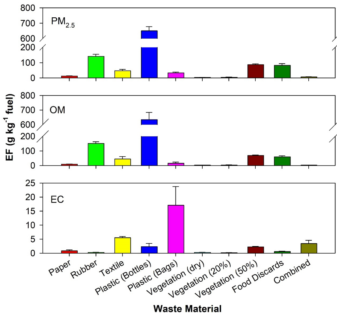
175 Figure 3: Emission factors for PM_{2.5} , organic matter (OM= OC \times 1.4), and elemental carbon (EC). The error bars represent the larger of the propagated analytical uncertainty or the standard error of multiple runs.
