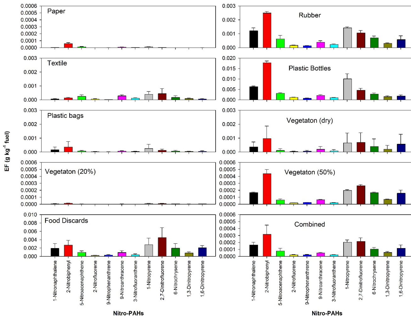
Figure 9: Emission factors for nitro-PAHs.
