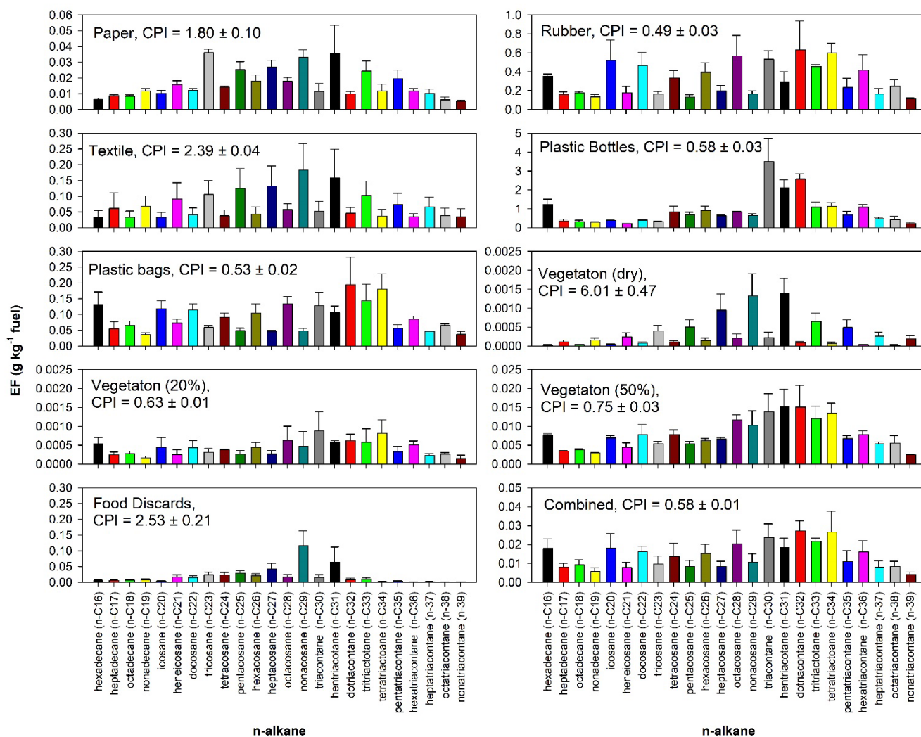
335 Figure 11: Emission factors for n-alkanes.
