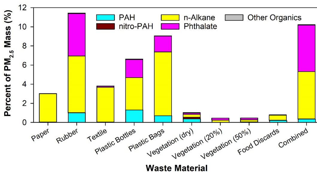
275 Figure 7: Abundances for organic groups (% of PM 2.5 mass).
