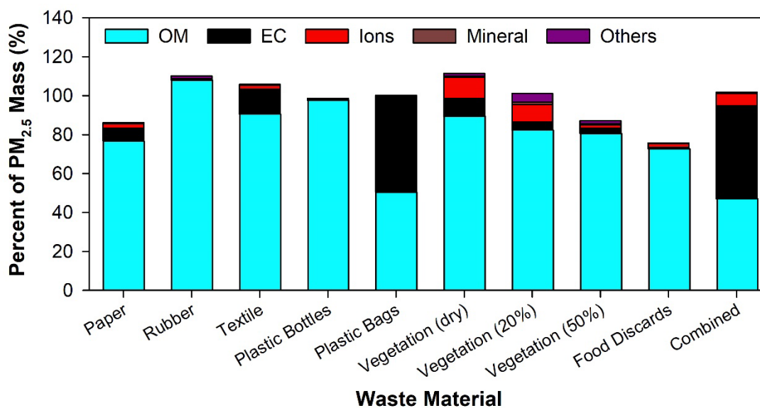
Figure 2: Abundances of major PM 2.5 compositions (percent of PM 2.5 mass) from burning of different waste materials (organic matter= OC × 1.4; ions is the sum of ammonium (NH 4 + ), sodium (Na + ), magnesium (Mg 2+ ), potassium (K + ), calcium (Ca 2+ ), fluoride (F - ), chloride (Cl - ), nitrite (NO 2 - ), nitrate (NO 3 - ), and sulfate (SO 4 2- ) by IC; minerals = 2.2×Al + 2.49×Si + 1.63×Ca + 2.42×Fe + 1.94×Ti.
