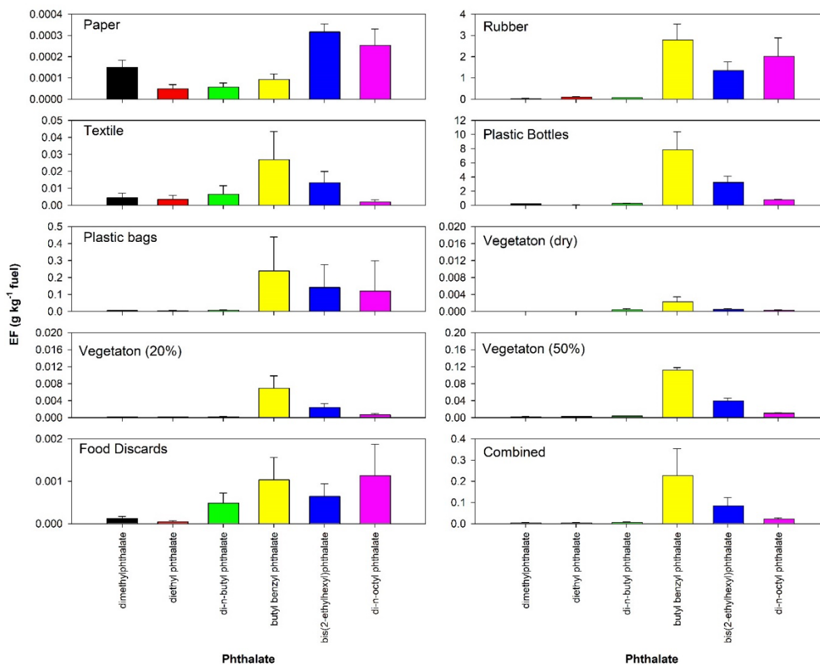
Figure 12: Emission factors for phthalates.
